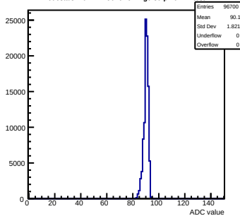
Pedestals mcm111-5610-rlv1-g0-s0-p1 ch 21 test1
