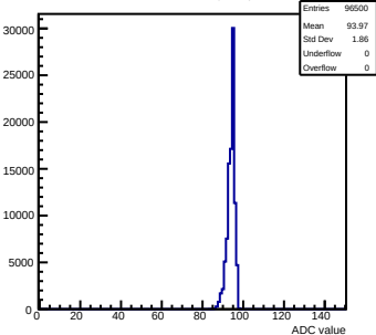
Pedestals mcm111-5610-refv1-g0-s0-p1 ch 113 test1
