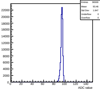
Pedestals mcm111-5610-refv1-g0-s0-p1 ch 123 test1
