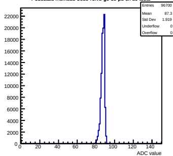
Pedestals mcm111-5610-rlv1-g0-s0-p1 ch 19 test1
