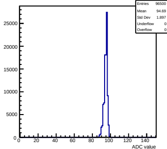
Pedestals mcm111-5610-refv1-g0-s0-p1 ch 122 test1
