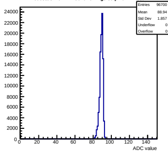
Pedestals mcm111-5610-rlv1-g0-s0-p1 ch 22 test1
