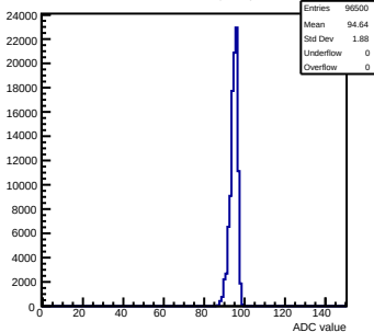
Pedestals mcm111-5610-refv1-g0-s0-p1 ch 116 test1
