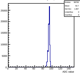
Pedestals mcm111-5610-rlv1-g0-s0-p1 ch 24 test1
