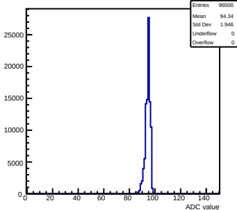
Pedestals mcm111-5610-refv1-g0-s0-p1 ch 112 test1
