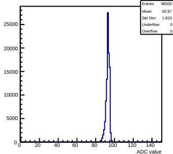
Pedestals mcm111-5610-refv1-g0-s0-p1 ch 118 test1
