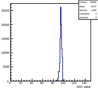
Pedestals mcm111-5610-refv1-g0-s0-p1 ch 127 test1
