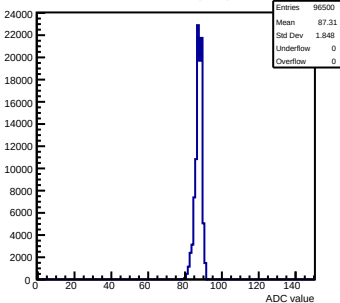
Pedestals mcm111-5610-refv1-g0-s0-p1 ch 119 test1
