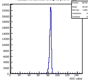
Pedestals mcm111-5610-rlv1-g0-s0-p1 ch 17 test1
