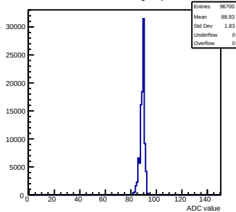
Pedestals mcm111-5610-rlv1-g0-s0-p1 ch 26 test1
