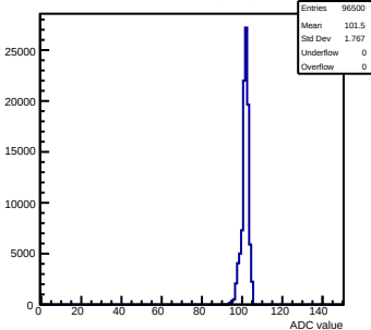
Pedestals mcm111-5610-refv1-g0-s0-p1 ch 115 test1
