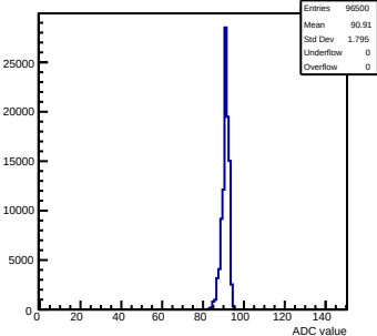
Pedestals mcm111-5610-refv1-g0-s0-p1 ch 125 test1
