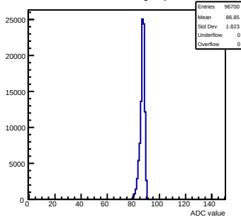
Pedestals mcm111-5610-rlv1-g0-s0-p1 ch 29 test1
