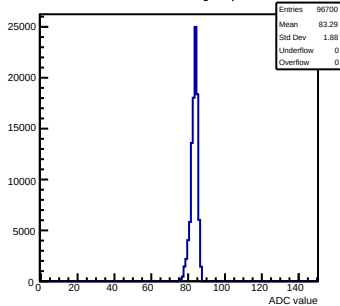
Pedestals mcm111-5610-rlv1-g0-s0-p1 ch 25 test1
