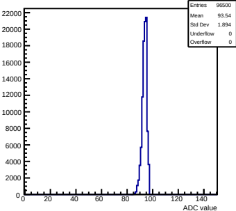
Pedestals mcm111-5610-refv1-g0-s0-p1 ch 121 test1
