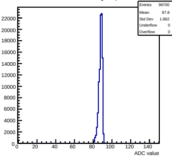
Pedestals mcm111-5610-rlv1-g0-s0-p1 ch 28 test1
