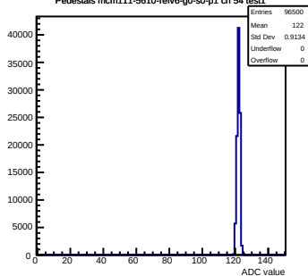
Pedestals mcm111-5610-relv6-g0-s0-p1 ch 54 test1
