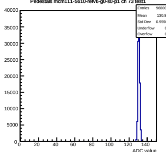
Pedestals mcm111-5610-refv6-g0-s0-p1 ch 73 test1
