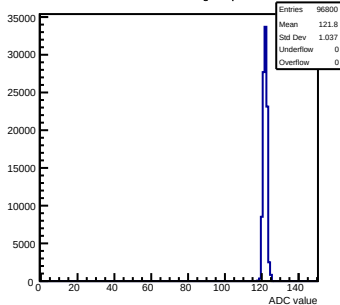
Pedestals mcm111-5610-refv6-g0-s0-p1 ch 14 test1
