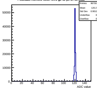
Pedestals mcm111-5610-relv6-g0-s0-p1 ch 18 test1
