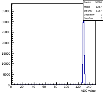
Pedestals mcm111-5610-refv6-g0-s0-p1 ch 104 test1
