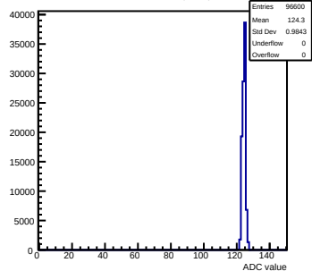
Pedestals mcm111-5610-refv6-g0-s0-p1 ch 101 test1
