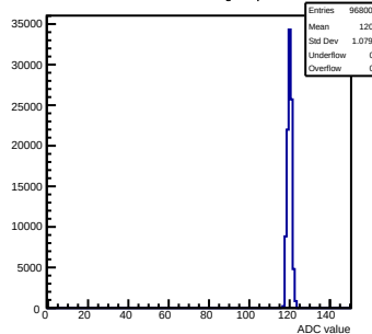
Pedestals mcm111-5610-refv6-g0-s0-p1 ch 11 test1
