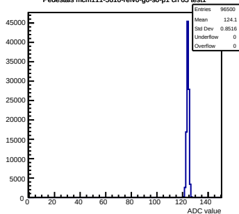
Pedestals mcm111-5610-relv6-g0-s0-p1 ch 63 test1
