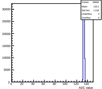
Pedestals mcm111-5610-refv6-g0-s0-p1 ch 111 test1
