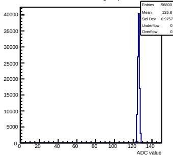
Pedestals mcm111-5610-refv6-g0-s0-p1 ch 10 test1
