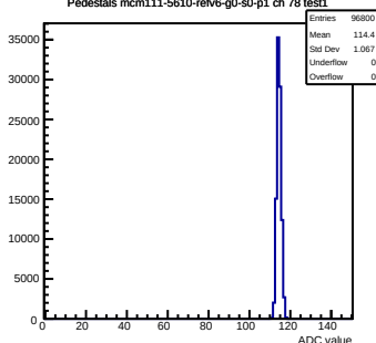
Pedestals mcm111-5610-refv6-g0-s0-p1 ch 78 test1
