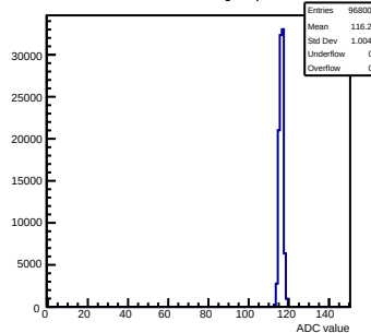
Pedestals mcm111-5610-refv6-g0-s0-p1 ch 15 test1
