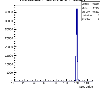
Pedestals mcm111-5610-relv6-g0-s0-p1 ch 60 test1
