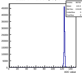
Pedestals mcm111-5610-relv6-g0-s0-p1 ch 24 test1
