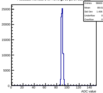
Pedestals mcm112-3414-refv1-g0-s0-p1 ch 102 test1
