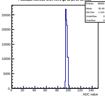
Pedestals mcm112-3414-refv1-g0-s0-p1 ch 98 test1
