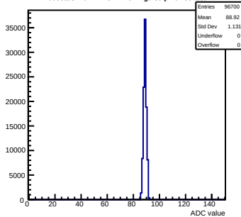
Pedestals mcm112-3414-rv1-g0-s0-p1 ch 85 test1
