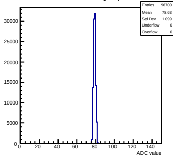
Pedestals mcm112-3414-rv1-g0-s0-p1 ch 94 test1
