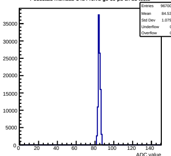
Pedestals mcm112-3414-rfv1-g0-s0-p1 ch 25 test1
