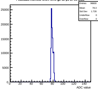
Pedestals mcm112-3414-refv1-g0-s0-p1 ch 96 test1
