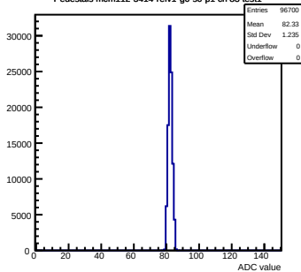
Pedestals mcm112-3414-rv1-g0-s0-p1 ch 83 test1
