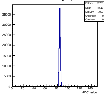
Pedestals mcm112-3414-rv1-g0-s0-p1 ch 91 test1
