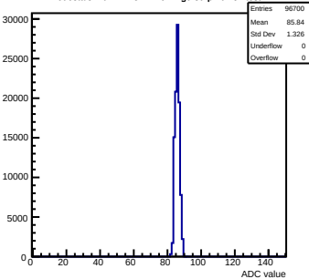
Pedestals mcm112-3414-rv1-g0-s0-p1 ch 84 test1
