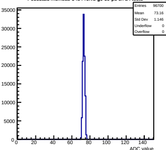
Pedestals mcm112-3414-rfv1-g0-s0-p1 ch 24 test1
