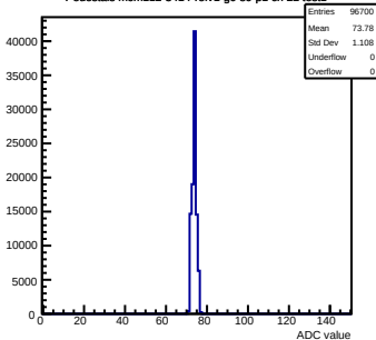
Pedestals mcm112-3414-rfv1-g0-s0-p1 ch 22 test1
