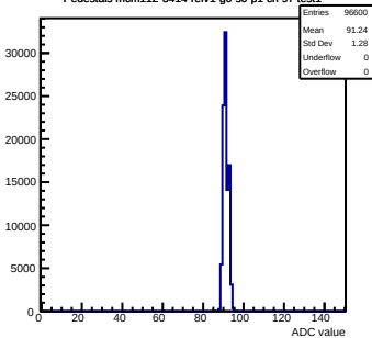
Pedestals mcm112-3414-refv1-g0-s0-p1 ch 97 test1
