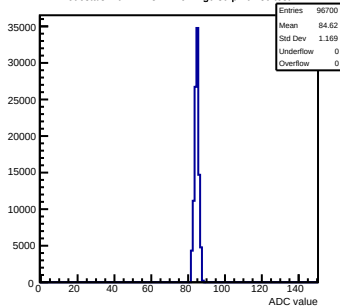
Pedestals mcm112-3414-rv1-g0-s0-p1 ch 89 test1
