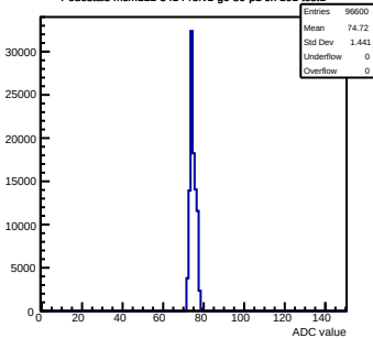
Pedestals mcm112-3414-refv1-g0-s0-p1 ch 101 test1
