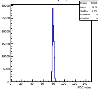
Pedestals mcm112-3414-refv1-g0-s0-p1 ch 111 test1
