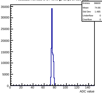
Pedestals mcm112-3414-refv1-g0-s0-p1 ch 100 test1
