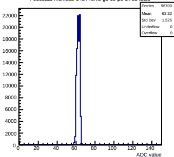
Pedestals mcm112-3414-refv2-g0-s0-p1 ch 25 test1
