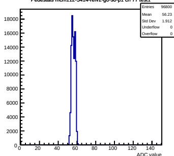
Pedestals mcm112-3414-refv2-g0-s0-p1 ch 77 test1
