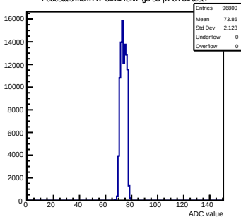
Pedestals mcm112-3414-refv2-g0-s0-p1 ch 64 test1
