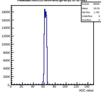
Pedestals mcm112-3414-refv2-g0-s0-p1 ch 52 test1
