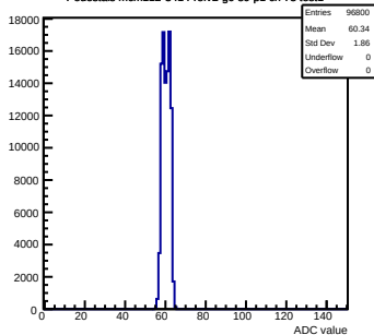
Pedestals mcm112-3414-refv2-g0-s0-p1 ch 73 test1
