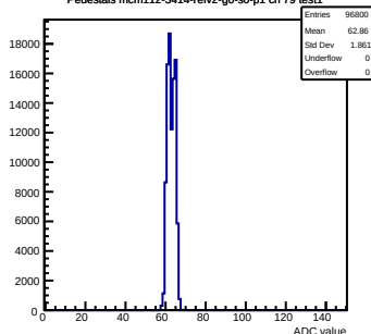
Pedestals mcm112-3414-refv2-g0-s0-p1 ch 79 test1
