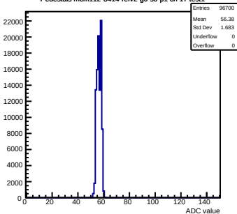
Pedestals mcm112-3414-refv2-g0-s0-p1 ch 17 test1
