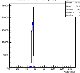
Pedestals mcm112-3414-refv2-g0-s0-p1 ch 27 test1
