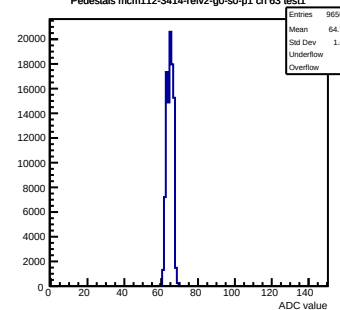
Pedestals mcm112-3414-refv2-g0-s0-p1 ch 63 test1
