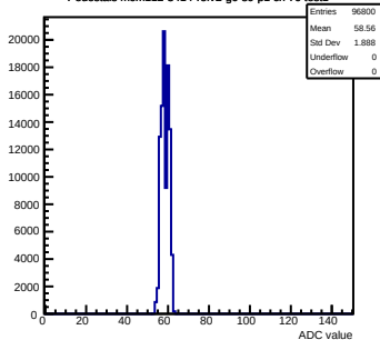
Pedestals mcm112-3414-refv2-g0-s0-p1 ch 70 test1
