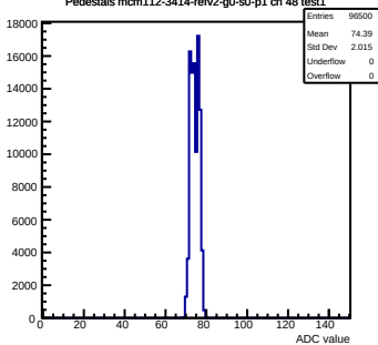
Pedestals mcm112-3414-refv2-g0-s0-p1 ch 48 test1
