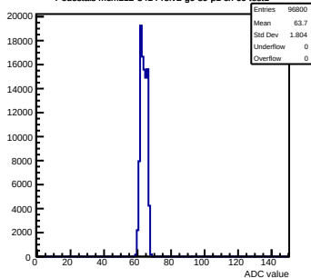
Pedestals mcm112-3414-refv2-g0-s0-p1 ch 69 test1
