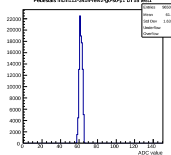
Pedestals mcm112-3414-refv2-g0-s0-p1 ch 58 test1
