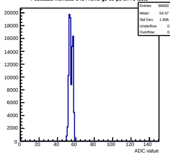
Pedestals mcm112-3414-refv2-g0-s0-p1 ch 75 test1
