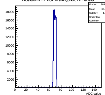
Pedestals mcm112-3414-refv2-g0-s0-p1 ch 59 test1
