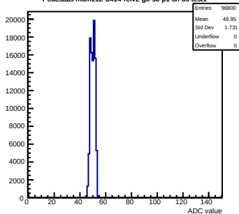
Pedestals mcm112-3414-refv2-g0-s0-p1 ch 65 test1
