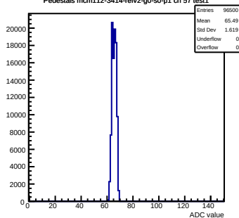
Pedestals mcm112-3414-refv2-g0-s0-p1 ch 57 test1
