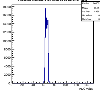
Pedestals mcm112-3414-refv2-g0-s0-p1 ch 67 test1
