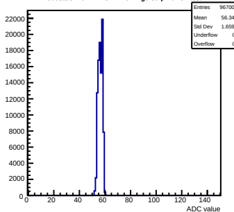
Pedestals mcm112-3414-refv2-g0-s0-p1 ch 31 test1
