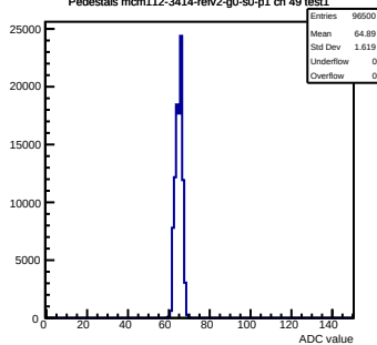
Pedestals mcm112-3414-refv2-g0-s0-p1 ch 49 test1
