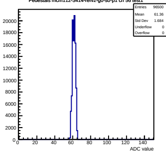
Pedestals mcm112-3414-refv2-g0-s0-p1 ch 56 test1
