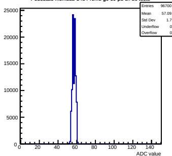
Pedestals mcm112-3414-refv2-g0-s0-p1 ch 26 test1
