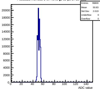
Pedestals mcm112-3414-refv2-g0-s0-p1 ch 68 test1
