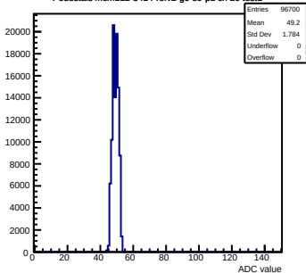
Pedestals mcm112-3414-refv2-g0-s0-p1 ch 20 test1
