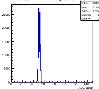
Pedestals mcm112-3414-refv2-g0-s0-p1 ch 22 test1
