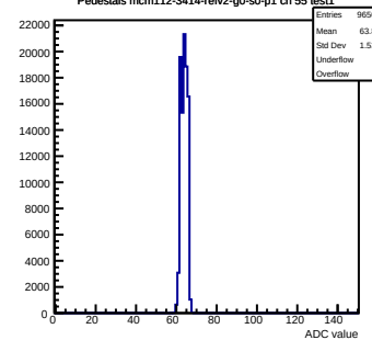
Pedestals mcm112-3414-refv2-g0-s0-p1 ch 55 test1
