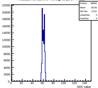
Pedestals mcm112-3414-refv2-g0-s0-p1 ch 74 test1
