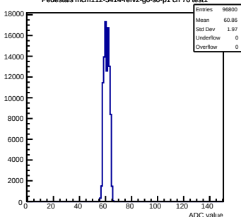
Pedestals mcm112-3414-refv2-g0-s0-p1 ch 76 test1
