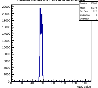
Pedestals mcm112-3414-refv2-g0-s0-p1 ch 66 test1
