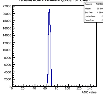
Pedestals mcm112-3414-refv2-g0-s0-p1 ch 53 test1
