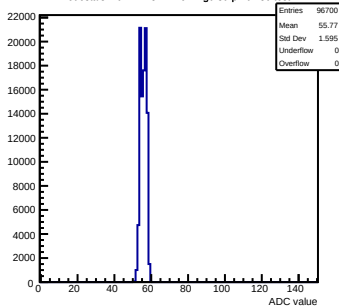
Pedestals mcm112-3414-refv2-g0-s0-p1 ch 30 test1
