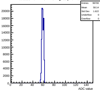
Pedestals mcm112-3414-refv2-g0-s0-p1 ch 29 test1
