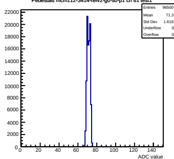
Pedestals mcm112-3414-refv2-g0-s0-p1 ch 61 test1
