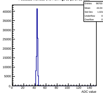
Pedestals mcm112-3414-rlv4-g0-s0-p1 ch 25 test1
