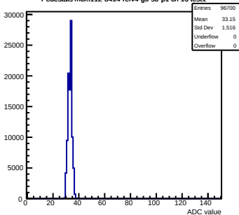
Pedestals mcm112-3414-rlv4-g0-s0-p1 ch 16 test1
