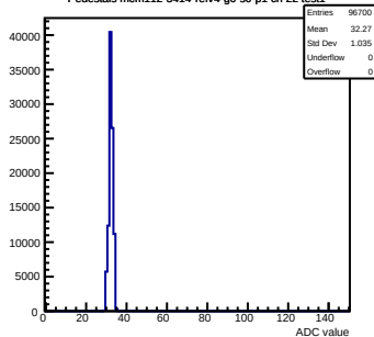
Pedestals mcm112-3414-rlv4-g0-s0-p1 ch 22 test1
