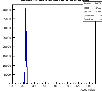
Pedestals mcm112-3414-rlv4-g0-s0-p1 ch 21 test1
