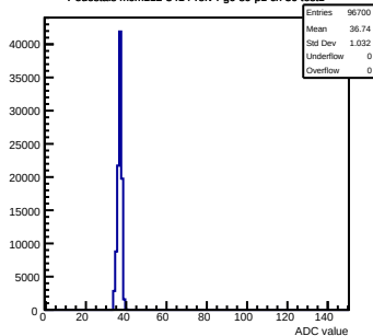
Pedestals mcm112-3414-rlv4-g0-s0-p1 ch 30 test1
