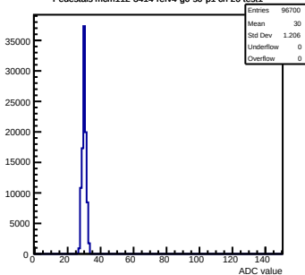
Pedestals mcm112-3414-rlv4-g0-s0-p1 ch 20 test1
