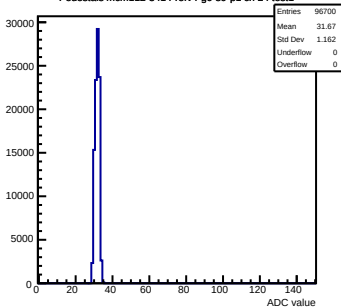
Pedestals mcm112-3414-rlv4-g0-s0-p1 ch 24 test1
