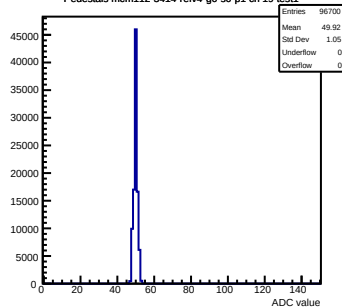
Pedestals mcm112-3414-rlv4-g0-s0-p1 ch 19 test1
