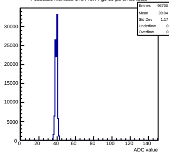
Pedestals mcm112-3414-rlv4-g0-s0-p1 ch 26 test1
