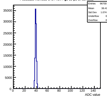
Pedestals mcm112-3414-rlv4-g0-s0-p1 ch 31 test1
