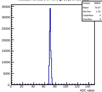
Pedestals mcm112-3414-refv5-g0-s0-p1 ch 100 test1
