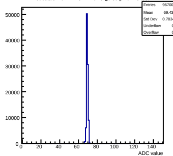
Pedestals mcm112-3414-rev5-g0-s0-p1 ch 23 test1
