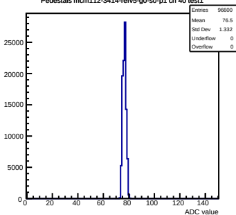
Pedestals mcm112-3414-rev5-g0-s0-p1 ch 40 test1
