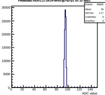
Pedestals mcm112-3414-rev5-g0-s0-p1 ch 32 test1
