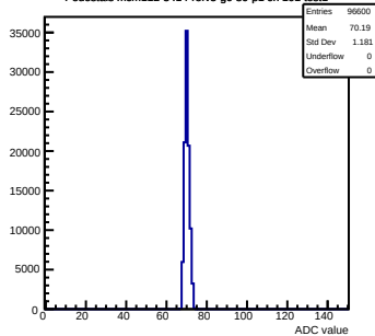
Pedestals mcm112-3414-refv5-g0-s0-p1 ch 101 test1
