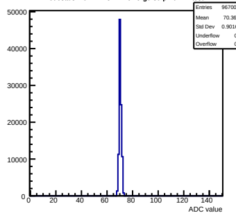
Pedestals mcm112-3414-rev5-g0-s0-p1 ch 27 test1
