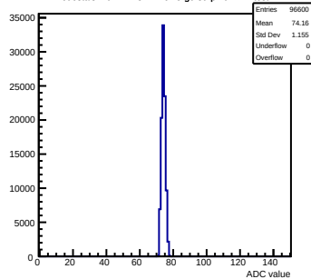
Pedestals mcm112-3414-refv5-g0-s0-p1 ch 111 test1
