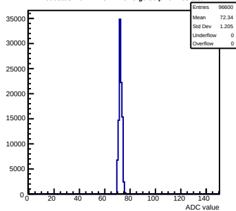
Pedestals mcm112-3414-refv5-g0-s0-p1 ch 105 test1
