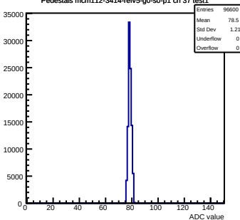
Pedestals mcm112-3414-rev5-g0-s0-p1 ch 37 test1
