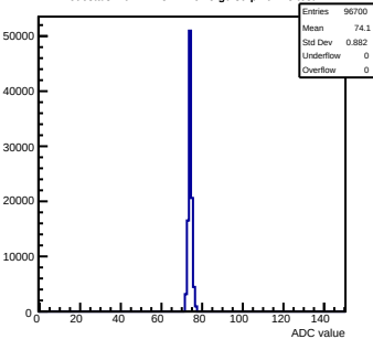
Pedestals mcm112-3414-rev5-g0-s0-p1 ch 28 test1
