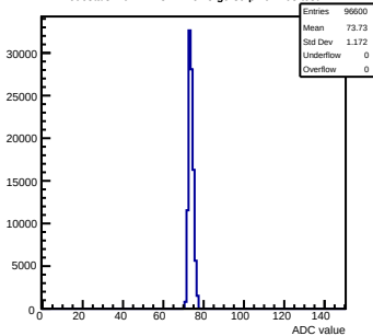
Pedestals mcm112-3414-refv5-g0-s0-p1 ch 108 test1
