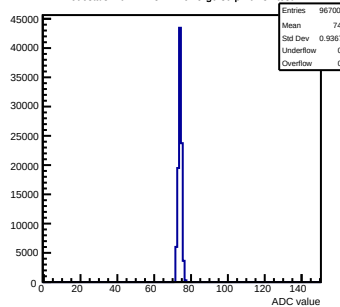
Pedestals mcm112-3414-rev5-g0-s0-p1 ch 31 test1
