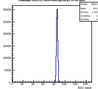
Pedestals mcm112-3414-rev5-g0-s0-p1 ch 43 test1
