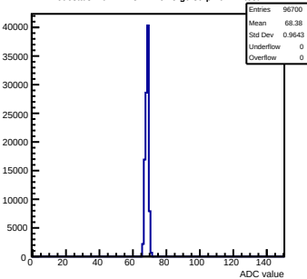
Pedestals mcm112-3414-rev5-g0-s0-p1 ch 24 test1
