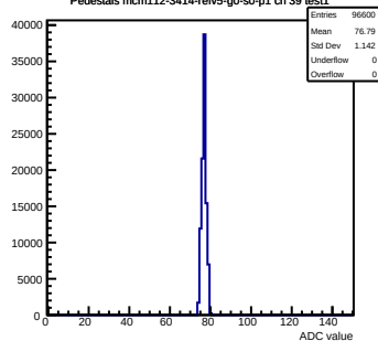
Pedestals mcm112-3414-rev5-g0-s0-p1 ch 39 test1
