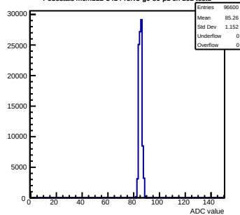
Pedestals mcm112-3414-refv5-g0-s0-p1 ch 102 test1
