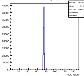
Pedestals mcm112-3414-rev5-g0-s0-p1 ch 30 test1
