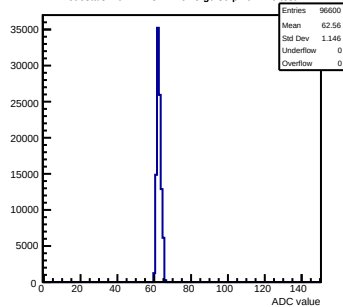
Pedestals mcm112-3414-refv5-g0-s0-p1 ch 110 test1
