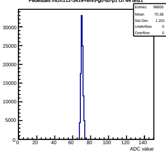
Pedestals mcm112-3414-rev5-g0-s0-p1 ch 44 test1
