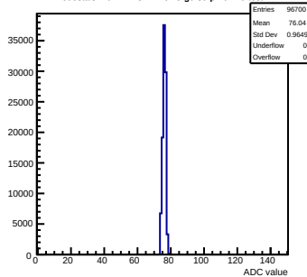
Pedestals mcm112-3414-rev5-g0-s0-p1 ch 29 test1
