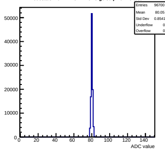
Pedestals mcm112-3414-rev5-g0-s0-p1 ch 25 test1
