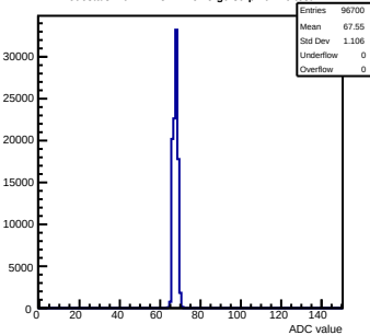
Pedestals mcm112-3414-rev5-g0-s0-p1 ch 20 test1
