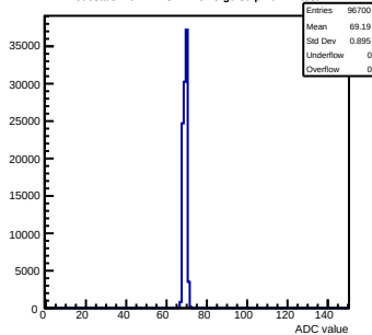
Pedestals mcm112-3414-rev5-g0-s0-p1 ch 22 test1
