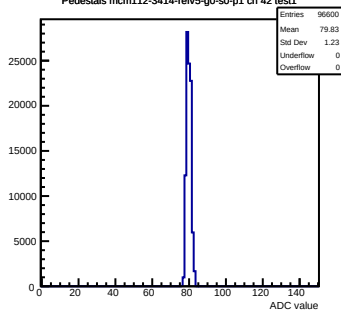
Pedestals mcm112-3414-rev5-g0-s0-p1 ch 42 test1
