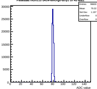
Pedestals mcm112-3414-rev5-g0-s0-p1 ch 45 test1
