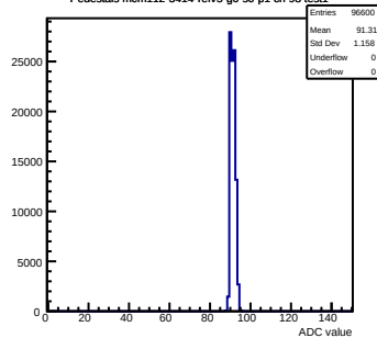
Pedestals mcm112-3414-refv5-g0-s0-p1 ch 98 test1
