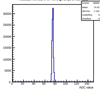
Pedestals mcm112-3414-refv5-g0-s0-p1 ch 103 test1
