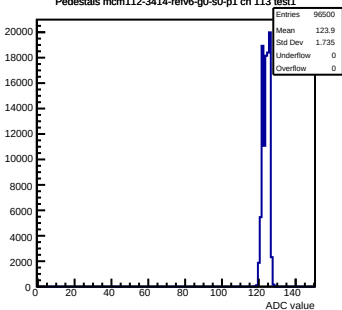
Pedestals mcm112-3414-refv6-g0-s0-p1 ch 113 test1
