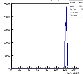
Pedestals mcm112-3414-rlv6-g0-s0-p1 ch 59 test1
