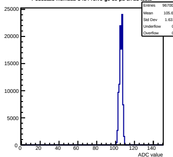
Pedestals mcm112-3414-rlv6-g0-s0-p1 ch 23 test1
