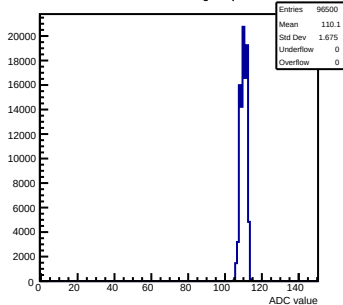
Pedestals mcm112-3414-rlv6-g0-s0-p1 ch 60 test1
