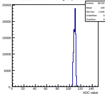
Pedestals mcm112-3414-rlv6-g0-s0-p1 ch 30 test1
