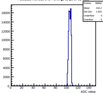
Pedestals mcm112-3414-rlv6-g0-s0-p1 ch 65 test1
