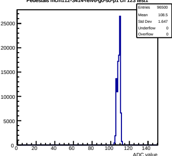
Pedestals mcm112-3414-refv6-g0-s0-p1 ch 123 test1
