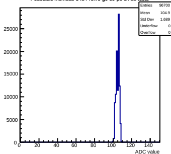
Pedestals mcm112-3414-rlv6-g0-s0-p1 ch 22 test1
