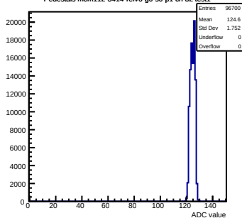
Pedestals mcm112-3414-rlv6-g0-s0-p1 ch 82 test1
