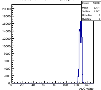
Pedestals mcm112-3414-rlv6-g0-s0-p1 ch 48 test1
