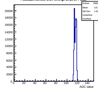
Pedestals mcm112-3414-rtv6-g0-s0-p1 ch 7 test1
