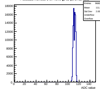
Pedestals mcm112-3414-rtv6-g0-s0-p1 ch 15 test1
