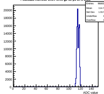
Pedestals mcm112-3414-rtv6-g0-s0-p1 ch 6 test1
