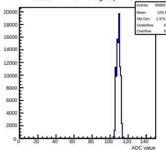
Pedestals mcm112-3414-rlv6-g0-s0-p1 ch 75 test1
