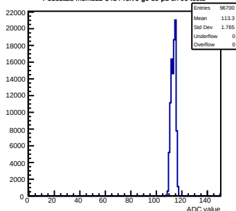
Pedestals mcm112-3414-rlv6-g0-s0-p1 ch 90 test1
