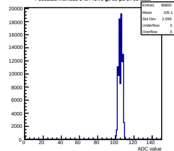
Pedestals mcm112-3414-rlv6-g0-s0-p1 ch 68 test1
