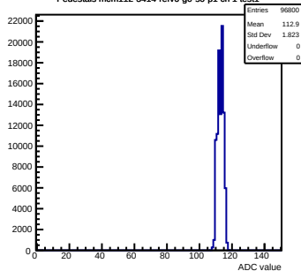
Pedestals mcm112-3414-rtv6-g0-s0-p1 ch 1 test1
