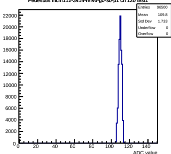
Pedestals mcm112-3414-refv6-g0-s0-p1 ch 120 test1
