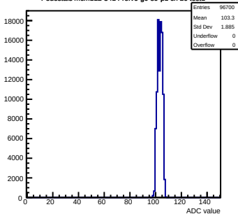
Pedestals mcm112-3414-rlv6-g0-s0-p1 ch 20 test1
