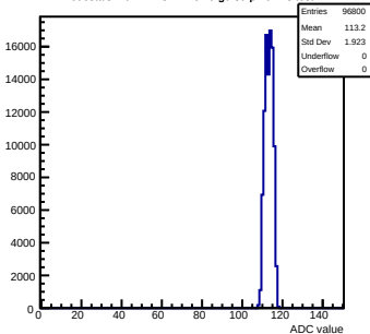
Pedestals mcm112-3414-rlv6-g0-s0-p1 ch 73 test1
