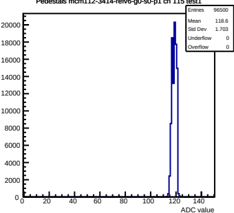
Pedestals mcm112-3414-refv6-g0-s0-p1 ch 115 test1
