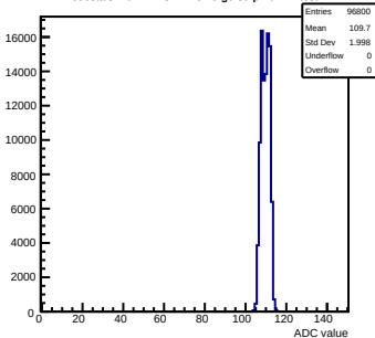
Pedestals mcm112-3414-rlv6-g0-s0-p1 ch 77 test1
