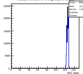
Pedestals mcm112-3414-rlv6-g0-s0-p1 ch 51 test1
