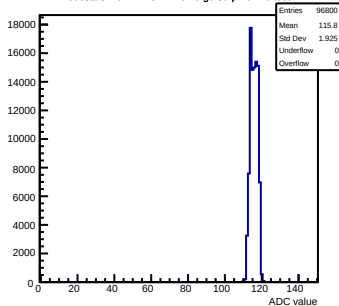
Pedestals mcm112-3414-rlv6-g0-s0-p1 ch 79 test1
