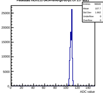
Pedestals mcm112-3414-refv6-g0-s0-p1 ch 117 test1
