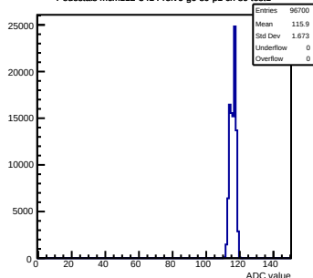
Pedestals mcm112-3414-rlv6-g0-s0-p1 ch 89 test1
