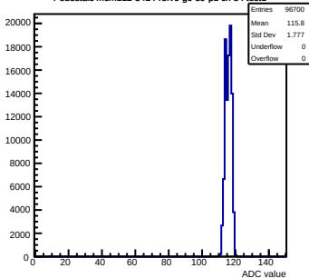
Pedestals mcm112-3414-rlv6-g0-s0-p1 ch 84 test1
