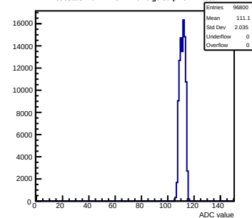
Pedestals mcm112-3414-rlv6-g0-s0-p1 ch 72 test1
