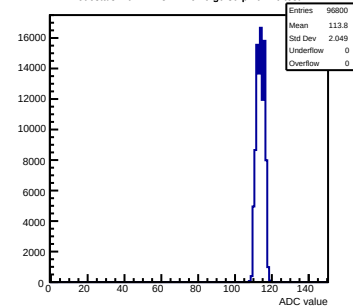
Pedestals mcm112-3414-rlv6-g0-s0-p1 ch 76 test1
