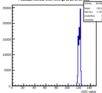
Pedestals mcm112-3414-rlv6-g0-s0-p1 ch 19 test1
