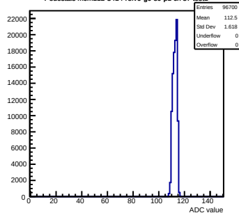
Pedestals mcm112-3414-rlv6-g0-s0-p1 ch 87 test1
