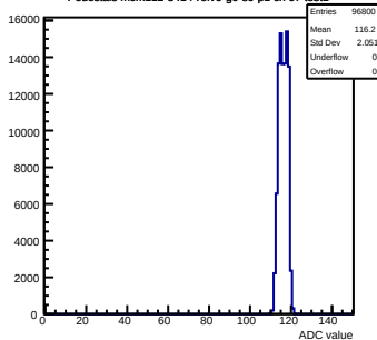
Pedestals mcm112-3414-rlv6-g0-s0-p1 ch 67 test1
