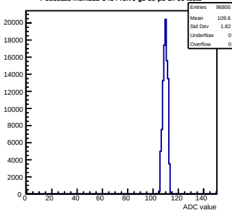
Pedestals mcm112-3414-rlv6-g0-s0-p1 ch 66 test1
