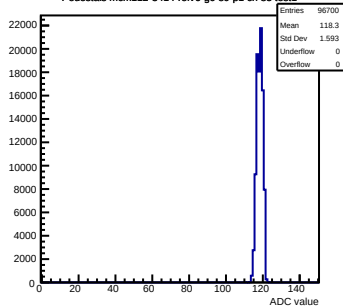
Pedestals mcm112-3414-rlv6-g0-s0-p1 ch 85 test1
