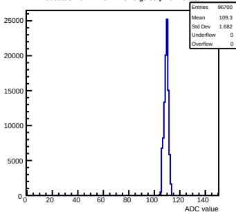
Pedestals mcm112-3414-rlv6-g0-s0-p1 ch 28 test1
