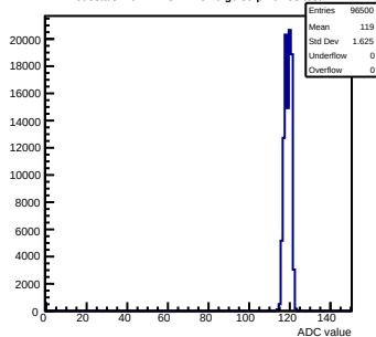
Pedestals mcm112-3414-rlv6-g0-s0-p1 ch 53 test1
