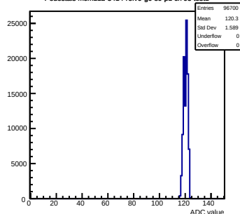
Pedestals mcm112-3414-rlv6-g0-s0-p1 ch 95 test1
