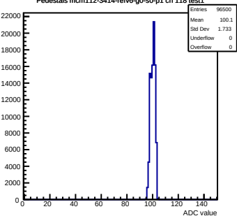
Pedestals mcm112-3414-refv6-g0-s0-p1 ch 118 test1
