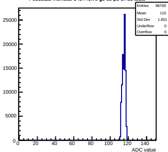
Pedestals mcm112-3414-rlv6-g0-s0-p1 ch 25 test1
