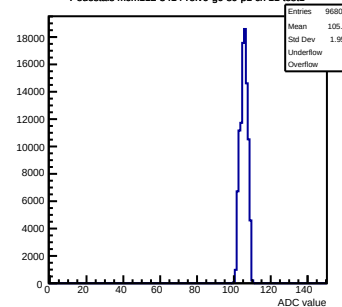
Pedestals mcm112-3414-rtv6-g0-s0-p1 ch 11 test1
