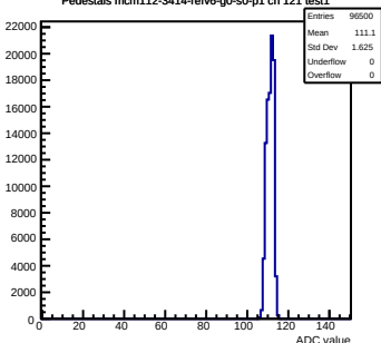
Pedestals mcm112-3414-refv6-g0-s0-p1 ch 121 test1
