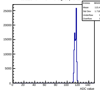
Pedestals mcm112-3414-rlv6-g0-s0-p1 ch 58 test1
