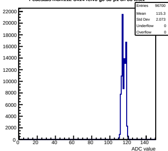
Pedestals mcm112-3414-rlv6-g0-s0-p1 ch 80 test1
