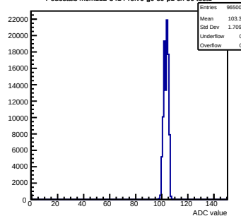
Pedestals mcm112-3414-rlv6-g0-s0-p1 ch 50 test1
