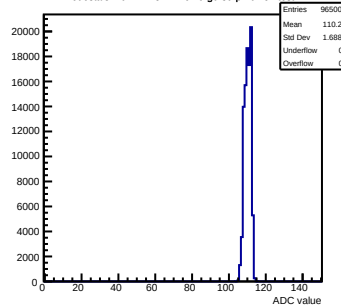
Pedestals mcm112-3414-rlv6-g0-s0-p1 ch 54 test1
