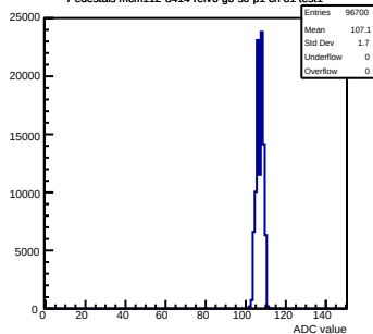
Pedestals mcm112-3414-rlv6-g0-s0-p1 ch 81 test1
