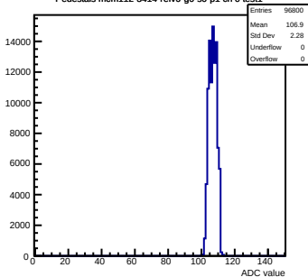
Pedestals mcm112-3414-rtv6-g0-s0-p1 ch 0 test1
