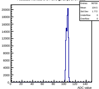
Pedestals mcm112-3414-rlv6-g0-s0-p1 ch 24 test1
