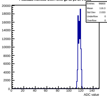
Pedestals mcm112-3414-rtv6-g0-s0-p1 ch 4 test1
