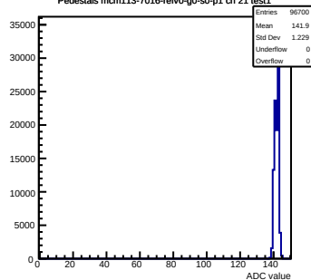
Pedestals mcm113-7016-rev0-g0-s0-p1 ch 21 test1
