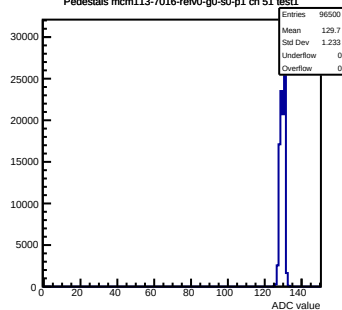
Pedestals mcm113-7016-rev0-g0-s0-p1 ch 51 test1
