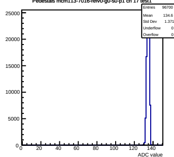
Pedestals mcm113-7016-rev0-g0-s0-p1 ch 17 test1
