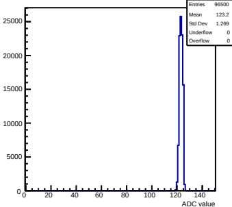
Pedestals mcm113-7016-refV0-g0-s0-p1 ch 123 test1
