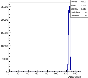
Pedestals mcm113-7016-refV0-g0-s0-p1 ch 116 test1
