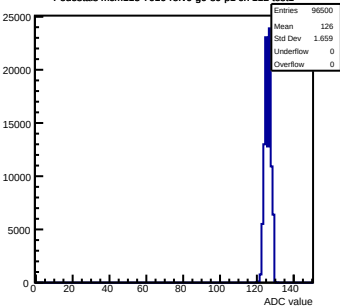
Pedestals mcm113-7016-refV0-g0-s0-p1 ch 112 test1
