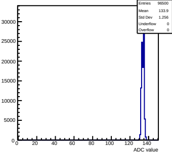
Pedestals mcm113-7016-refV0-g0-s0-p1 ch 120 test1
