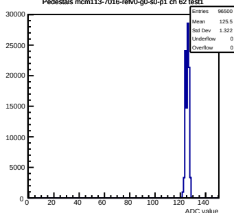
Pedestals mcm113-7016-rev0-g0-s0-p1 ch 62 test1
