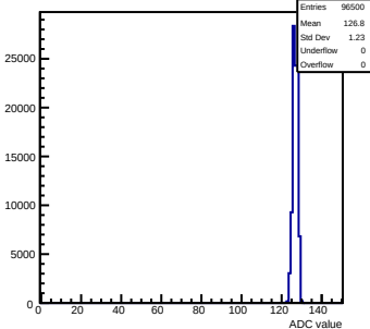
Pedestals mcm113-7016-refV0-g0-s0-p1 ch 126 test1
