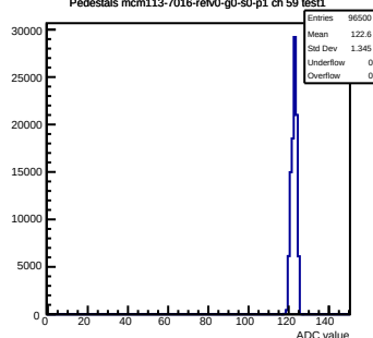
Pedestals mcm113-7016-rev0-g0-s0-p1 ch 59 test1
