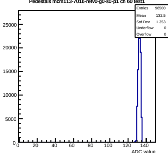
Pedestals mcm113-7016-rev0-g0-s0-p1 ch 60 test1
