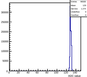
Pedestals mcm113-7016-refV0-g0-s0-p1 ch 127 test1
