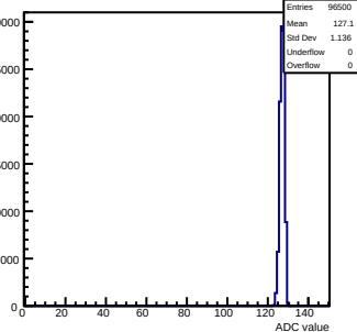
Pedestals mcm113-7016-refV0-g0-s0-p1 ch 121 test1
