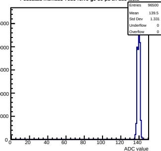
Pedestals mcm113-7016-refV0-g0-s0-p1 ch 113 test1
