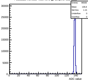
Pedestals mcm113-7016-refV0-g0-s0-p1 ch 115 test1
