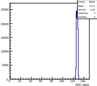
Pedestals mcm113-7016-refV0-g0-s0-p1 ch 124 test1
