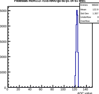
Pedestals mcm113-7016-rev0-g0-s0-p1 ch 61 test1
