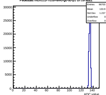
Pedestals mcm113-7016-rev0-g0-s0-p1 ch 29 test1
