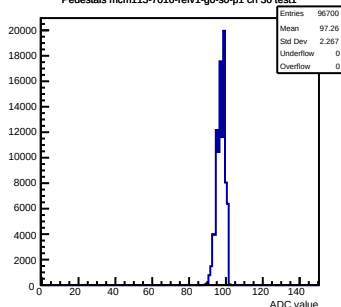
Pedestals mcm113-7016-rlv1-g0-s0-p1 ch 30 test1
