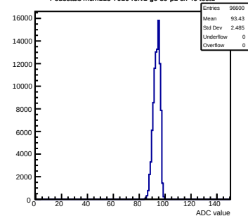
Pedestals mcm113-7016-rvf1-g0-s0-p1 ch 40 test1
