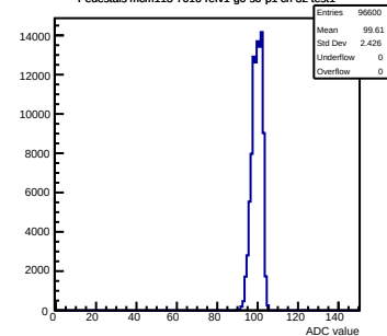
Pedestals mcm113-7016-rvf1-g0-s0-p1 ch 32 test1
