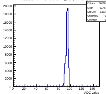
Pedestals mcm113-7016-rv1-g0-s0-p1 ch 55 test1
