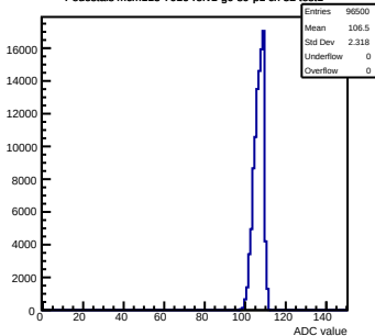
Pedestals mcm113-7016-rv1-g0-s0-p1 ch 52 test1
