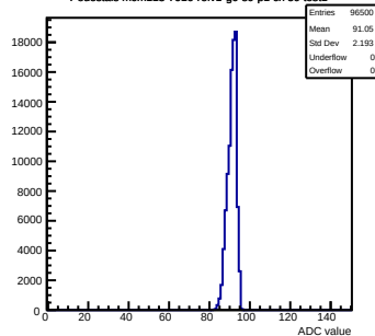
Pedestals mcm113-7016-rv1-g0-s0-p1 ch 59 test1
