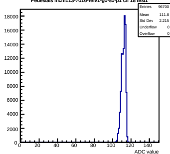
Pedestals mcm113-7016-rlv1-g0-s0-p1 ch 18 test1
