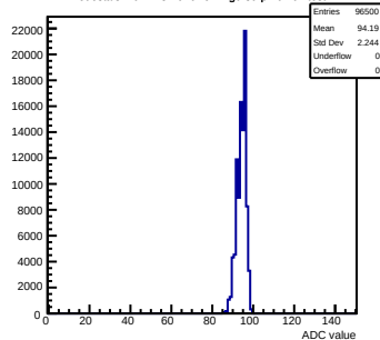
Pedestals mcm113-7016-rv1-g0-s0-p1 ch 62 test1
