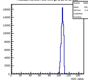
Pedestals mcm113-7016-rvf1-g0-s0-p1 ch 35 test1
