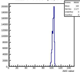
Pedestals mcm113-7016-rv1-g0-s0-p1 ch 60 test1
