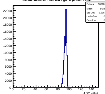
Pedestals mcm113-7016-rlv1-g0-s0-p1 ch 31 test1
