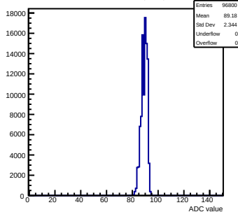
Pedestals mcm113-7016-refv1-g0-s0-p1 ch 71 test1
