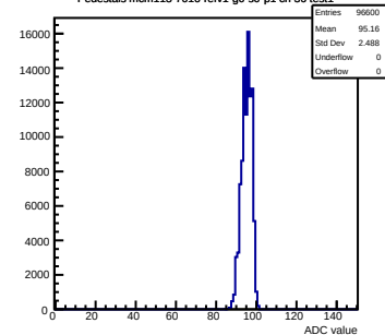
Pedestals mcm113-7016-rvf1-g0-s0-p1 ch 36 test1
