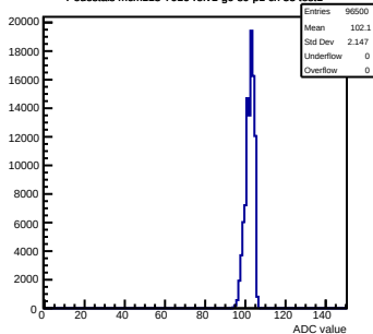
Pedestals mcm113-7016-rv1-g0-s0-p1 ch 53 test1
