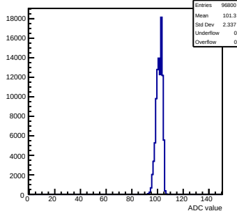
Pedestals mcm113-7016-refv1-g0-s0-p1 ch 77 test1
