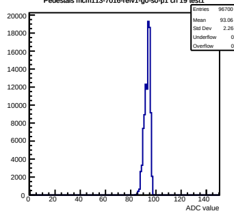
Pedestals mcm113-7016-rlv1-g0-s0-p1 ch 19 test1
