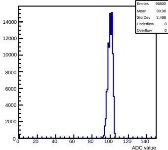
Pedestals mcm113-7016-refv1-g0-s0-p1 ch 68 test1
