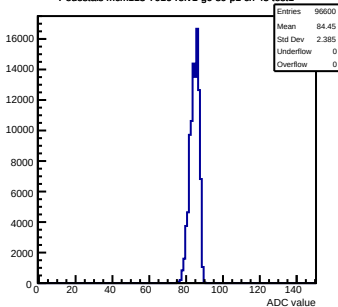
Pedestals mcm113-7016-rvf1-g0-s0-p1 ch 45 test1
