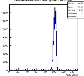
Pedestals mcm113-7016-rlv1-g0-s0-p1 ch 16 test1
