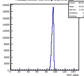
Pedestals mcm113-7016-rlv1-g0-s0-p1 ch 23 test1
