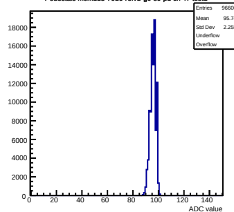
Pedestals mcm113-7016-rvf1-g0-s0-p1 ch 47 test1
