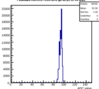
Pedestals mcm113-7016-rlv1-g0-s0-p1 ch 24 test1
