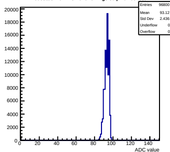
Pedestals mcm113-7016-refv1-g0-s0-p1 ch 65 test1
