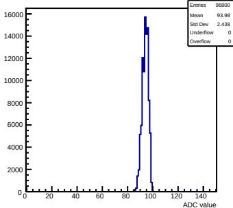
Pedestals mcm113-7016-refv1-g0-s0-p1 ch 76 test1
