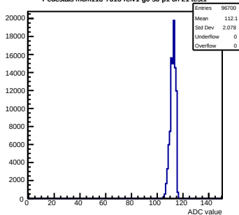
Pedestals mcm113-7016-rlv1-g0-s0-p1 ch 21 test1
