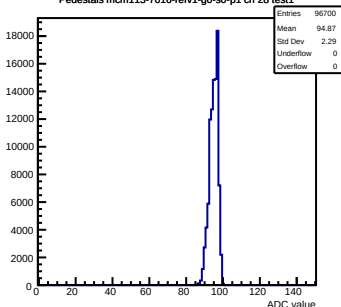
Pedestals mcm113-7016-rlv1-g0-s0-p1 ch 28 test1
