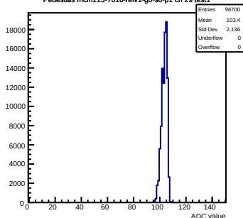
Pedestals mcm113-7016-rlv1-g0-s0-p1 ch 29 test1
