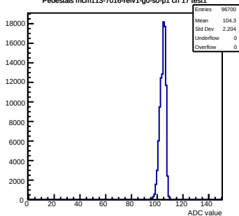
Pedestals mcm113-7016-rlv1-g0-s0-p1 ch 17 test1
