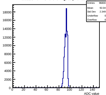
Pedestals mcm113-7016-refv1-g0-s0-p1 ch 66 test1
