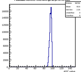
Pedestals mcm113-7016-rlv1-g0-s0-p1 ch 25 test1
