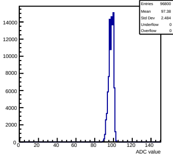
Pedestals mcm113-7016-refv1-g0-s0-p1 ch 72 test1
