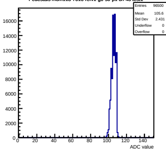
Pedestals mcm113-7016-rv1-g0-s0-p1 ch 48 test1
