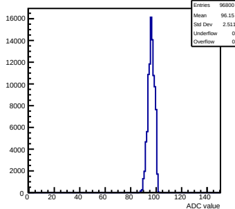
Pedestals mcm113-7016-refv1-g0-s0-p1 ch 74 test1
