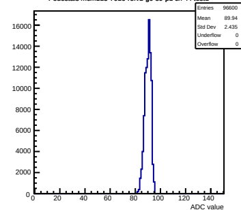
Pedestals mcm113-7016-rvf1-g0-s0-p1 ch 44 test1
