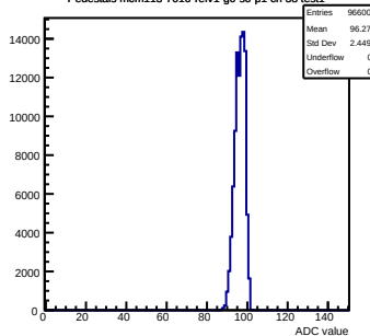
Pedestals mcm113-7016-rvf1-g0-s0-p1 ch 38 test1
