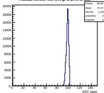
Pedestals mcm113-7016-rlv1-g0-s0-p1 ch 22 test1
