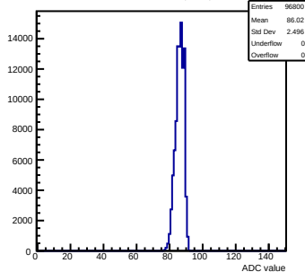
Pedestals mcm113-7016-refv1-g0-s0-p1 ch 70 test1
