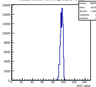
Pedestals mcm113-7016-rvf1-g0-s0-p1 ch 42 test1
