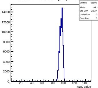
Pedestals mcm113-7016-refv1-g0-s0-p1 ch 64 test1
