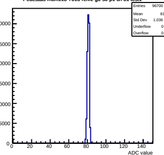
Pedestals mcm113-7016-ref2-g0-s0-p1 ch 81 test1
