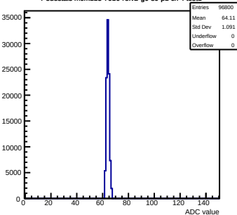
Pedestals mcm113-7016-refv2-g0-s0-p1 ch 4 test1
