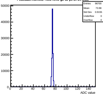
Pedestals mcm113-7016-ref2-g0-s0-p1 ch 84 test1
