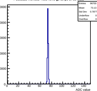
Pedestals mcm113-7016-ref2-g0-s0-p1 ch 89 test1
