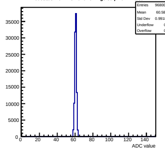
Pedestals mcm113-7016-refv2-g0-s0-p1 ch 11 test1
