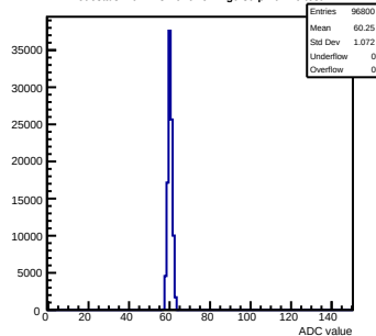
Pedestals mcm113-7016-refv2-g0-s0-p1 ch 10 test1
