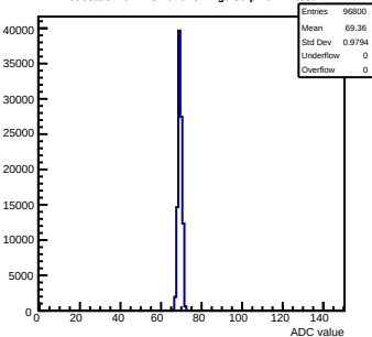
Pedestals mcm113-7016-refv2-g0-s0-p1 ch 12 test1
