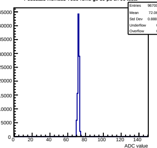
Pedestals mcm113-7016-ref2-g0-s0-p1 ch 90 test1
