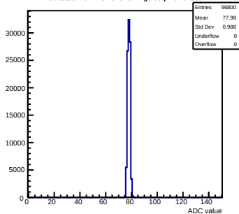
Pedestals mcm113-7016-refv2-g0-s0-p1 ch 9 test1
