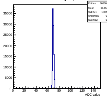
Pedestals mcm113-7016-refv2-g0-s0-p1 ch 14 test1
