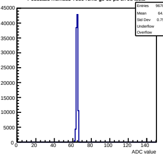
Pedestals mcm113-7016-ref2-g0-s0-p1 ch 91 test1
