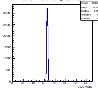
Pedestals mcm113-7016-refv2-g0-s0-p1 ch 3 test1
