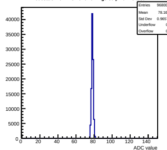
Pedestals mcm113-7016-refv2-g0-s0-p1 ch 15 test1
