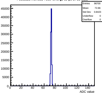
Pedestals mcm113-7016-ref2-g0-s0-p1 ch 88 test1
