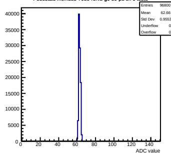
Pedestals mcm113-7016-refv2-g0-s0-p1 ch 6 test1
