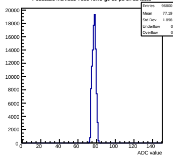
Pedestals mcm113-7016-refv5-g0-s0-p1 ch 11 test1
