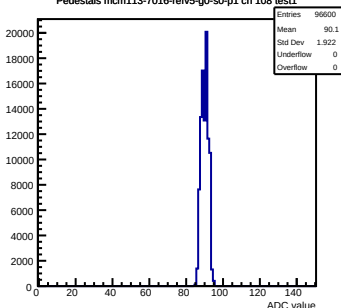
Pedestals mcm113-7016-refV5-g0-s0-p1 ch 108 test1
