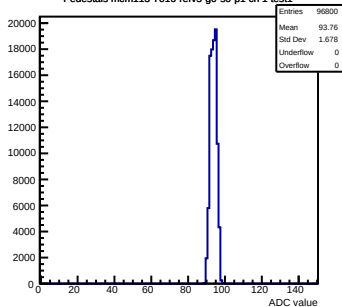
Pedestals mcm113-7016-refv5-g0-s0-p1 ch 1 test1
