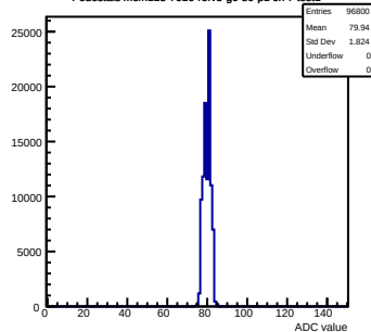
Pedestals mcm113-7016-refv5-g0-s0-p1 ch 7 test1
