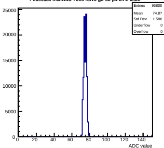
Pedestals mcm113-7016-refv5-g0-s0-p1 ch 2 test1
