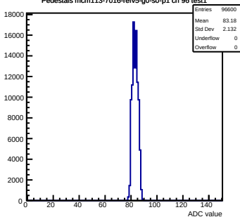
Pedestals mcm113-7016-refV5-g0-s0-p1 ch 96 test1
