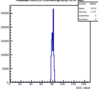
Pedestals mcm113-7016-refV5-g0-s0-p1 ch 97 test1
