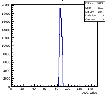
Pedestals mcm113-7016-refv5-g0-s0-p1 ch 12 test1
