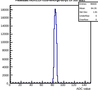
Pedestals mcm113-7016-refV5-g0-s0-p1 ch 102 test1
