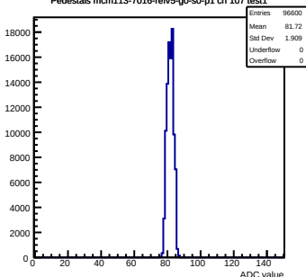
Pedestals mcm113-7016-refV5-g0-s0-p1 ch 107 test1
