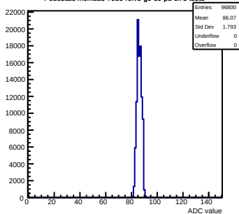
Pedestals mcm113-7016-refv5-g0-s0-p1 ch 5 test1
