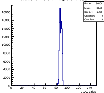
Pedestals mcm113-7016-refv5-g0-s0-p1 ch 8 test1
