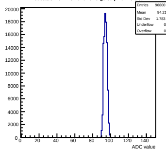
Pedestals mcm113-7016-refv5-g0-s0-p1 ch 15 test1
