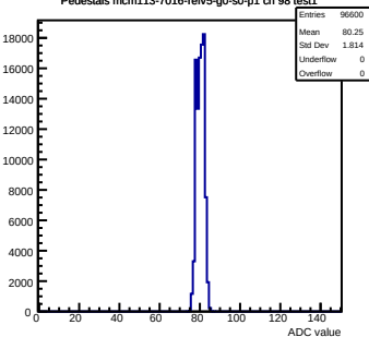
Pedestals mcm113-7016-refV5-g0-s0-p1 ch 98 test1
