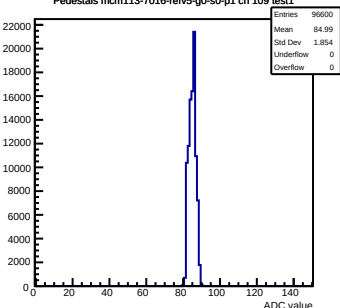
Pedestals mcm113-7016-refV5-g0-s0-p1 ch 109 test1
