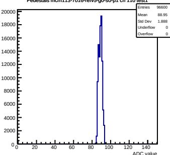
Pedestals mcm113-7016-refV5-g0-s0-p1 ch 110 test1
