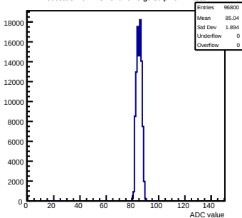
Pedestals mcm113-7016-refv5-g0-s0-p1 ch 14 test1
