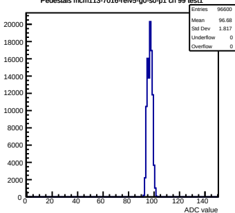
Pedestals mcm113-7016-refV5-g0-s0-p1 ch 99 test1
