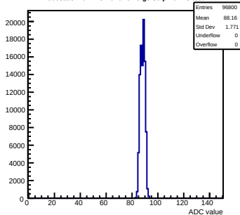
Pedestals mcm113-7016-refv5-g0-s0-p1 ch 13 test1
