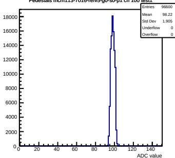
Pedestals mcm113-7016-refV5-g0-s0-p1 ch 100 test1
