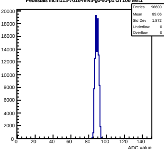
Pedestals mcm113-7016-refV5-g0-s0-p1 ch 106 test1
