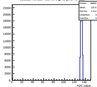
Pedestals mcm113-7016-relv6-g0-s0-p1 ch 73 test1
