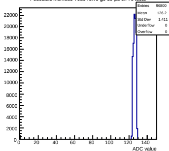
Pedestals mcm113-7016-relv6-g0-s0-p1 ch 76 test1
