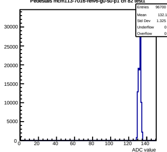
Pedestals mcm113-7016-relv6-g0-s0-p1 ch 82 test1
