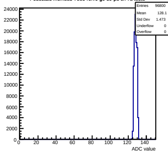
Pedestals mcm113-7016-relv6-g0-s0-p1 ch 72 test1
