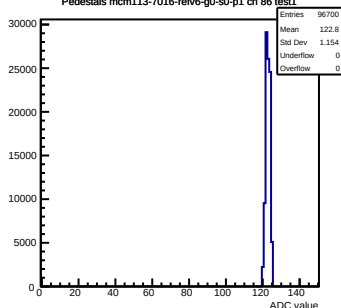
Pedestals mcm113-7016-relv6-g0-s0-p1 ch 86 test1
