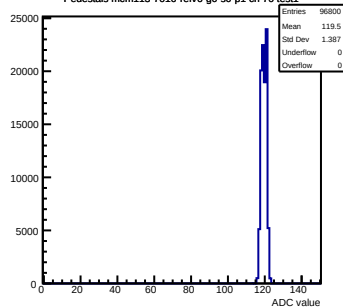
Pedestals mcm113-7016-relv6-g0-s0-p1 ch 70 test1
