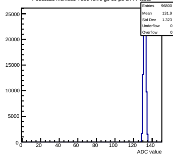
Pedestals mcm113-7016-relv6-g0-s0-p1 ch 77 test1
