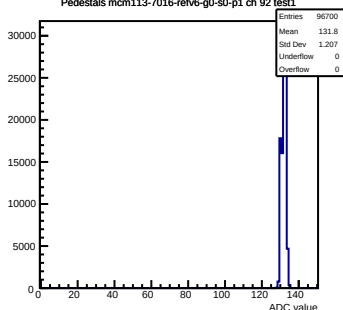
Pedestals mcm113-7016-relv6-g0-s0-p1 ch 92 test1
