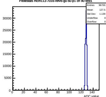
Pedestals mcm113-7016-relv6-g0-s0-p1 ch 90 test1
