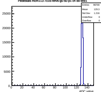
Pedestals mcm113-7016-relv6-g0-s0-p1 ch 88 test1
