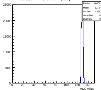
Pedestals mcm113-7016-relv6-g0-s0-p1 ch 74 test1
