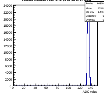
Pedestals mcm113-7016-relv6-g0-s0-p1 ch 67 test1
