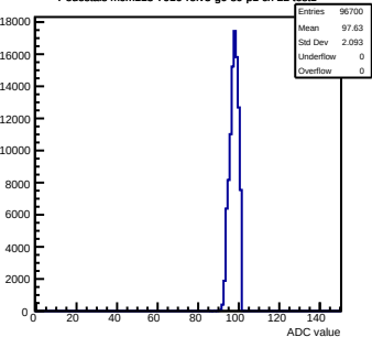
Pedestals mcm113-7016-rvf5-g0-s0-p1 ch 22 test1
