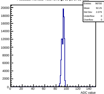
Pedestals mcm113-7016-rvf5-g0-s0-p1 ch 25 test1
