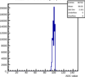
Pedestals mcm113-7016-rvf5-g0-s0-p1 ch 30 test1
