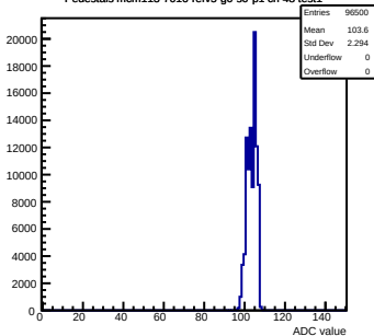
Pedestals mcm113-7016-refv5-g0-s0-p1 ch 48 test1
