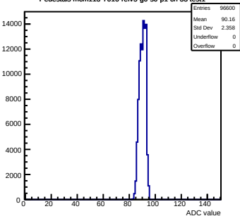
Pedestals mcm113-7016-rv5-g0-s0-p1 ch 33 test1
