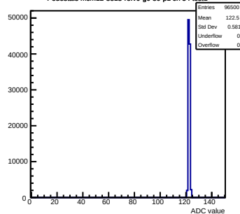
Pedestals mcm12-8815-refV0-g0-s0-p1 ch 54 test1
