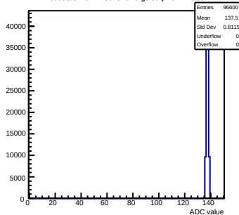
Pedestals mcm12-8815-refV0-g0-s0-p1 ch 42 test1
