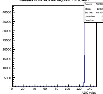
Pedestals mcm12-8815-refV0-g0-s0-p1 ch 98 test1
