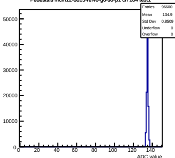
Pedestals mcm12-8815-refV0-g0-s0-p1 ch 104 test1
