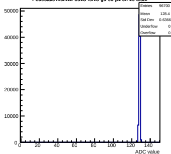
Pedestals mcm12-8815-refV0-g0-s0-p1 ch 19 test1
