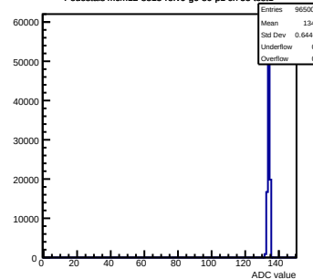
Pedestals mcm12-8815-refV0-g0-s0-p1 ch 55 test1
