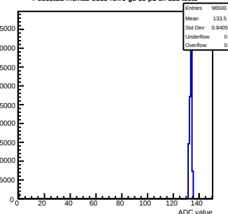
Pedestals mcm12-8815-refV0-g0-s0-p1 ch 121 test1
