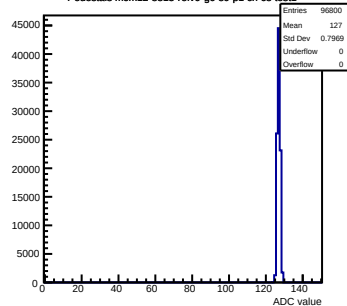
Pedestals mcm12-8815-refV0-g0-s0-p1 ch 68 test1
