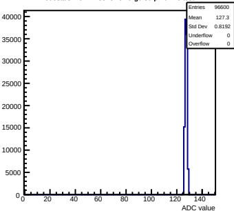
Pedestals mcm12-8815-refV0-g0-s0-p1 ch 40 test1
