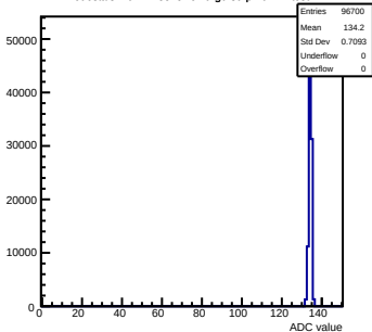
Pedestals mcm12-8815-refV0-g0-s0-p1 ch 24 test1
