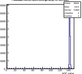
Pedestals mcm12-8815-refV0-g0-s0-p1 ch 105 test1
