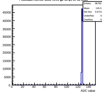
Pedestals mcm12-8815-refV0-g0-s0-p1 ch 18 test1
