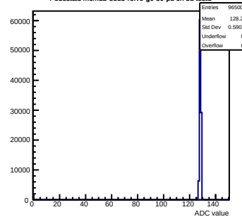
Pedestals mcm12-8815-refV0-g0-s0-p1 ch 51 test1
