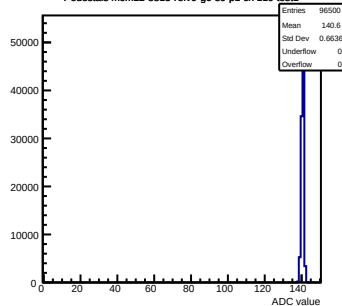
Pedestals mcm12-8815-refV0-g0-s0-p1 ch 119 test1
