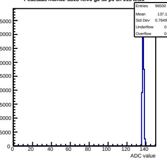
Pedestals mcm12-8815-refV0-g0-s0-p1 ch 113 test1
