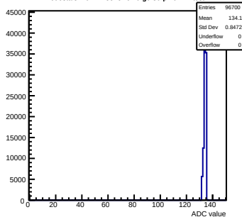
Pedestals mcm12-8815-refV0-g0-s0-p1 ch 27 test1
