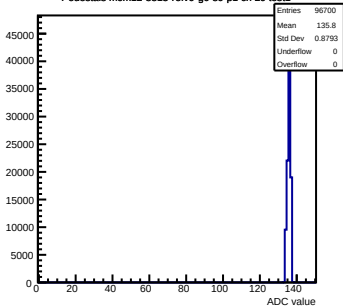
Pedestals mcm12-8815-refV0-g0-s0-p1 ch 20 test1
