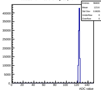
Pedestals mcm12-8815-refv0-g0-s0-p1 ch 10 test1
