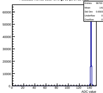
Pedestals mcm12-8815-refV0-g0-s0-p1 ch 22 test1
