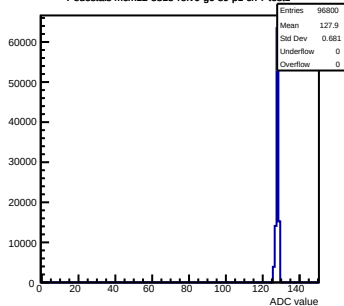
Pedestals mcm12-8815-refv0-g0-s0-p1 ch 7 test1
