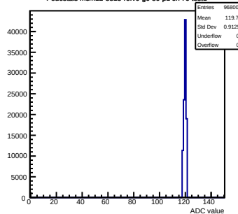
Pedestals mcm12-8815-refV0-g0-s0-p1 ch 70 test1
