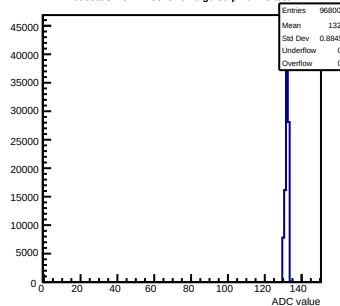
Pedestals mcm12-8815-refV0-g0-s0-p1 ch 78 test1
