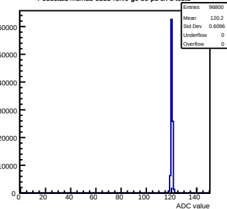
Pedestals mcm12-8815-refv0-g0-s0-p1 ch 1 test1
