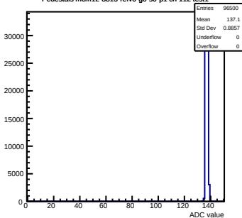
Pedestals mcm12-8815-refV0-g0-s0-p1 ch 112 test1
