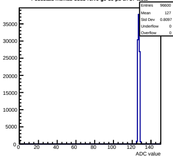
Pedestals mcm12-8815-refV0-g0-s0-p1 ch 37 test1
