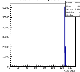
Pedestals mcm12-8815-refV0-g0-s0-p1 ch 74 test1
