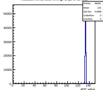
Pedestals mcm12-8815-refV0-g0-s0-p1 ch 56 test1
