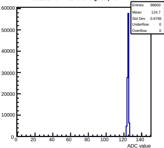
Pedestals mcm12-8815-refV0-g0-s0-p1 ch 44 test1
