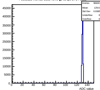
Pedestals mcm12-8815-refV0-g0-s0-p1 ch 34 test1
