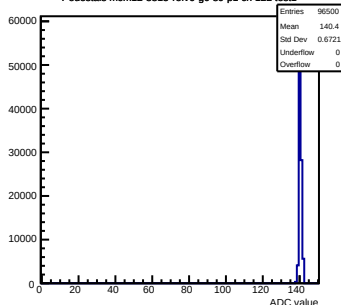
Pedestals mcm12-8815-refV0-g0-s0-p1 ch 122 test1
