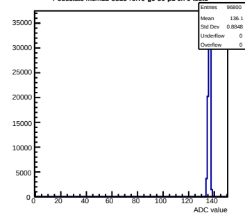
Pedestals mcm12-8815-refv0-g0-s0-p1 ch 0 test1
