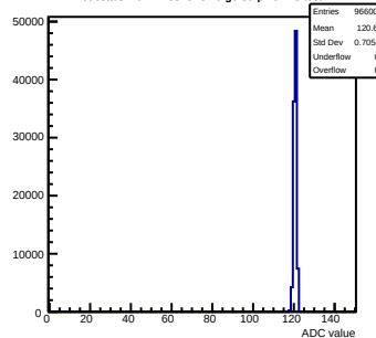
Pedestals mcm12-8815-refV0-g0-s0-p1 ch 43 test1
