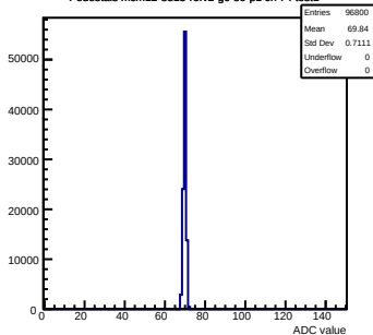
Pedestals mcm12-8815-refv2-g0-s0-p1 ch 74 test1
