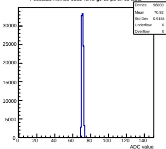
Pedestals mcm12-8815-refv2-g0-s0-p1 ch 68 test1
