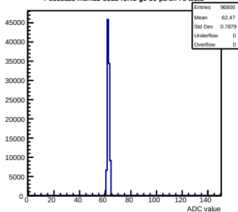
Pedestals mcm12-8815-refv2-g0-s0-p1 ch 70 test1
