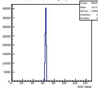
Pedestals mcm12-8815-refv2-g0-s0-p1 ch 43 test1
