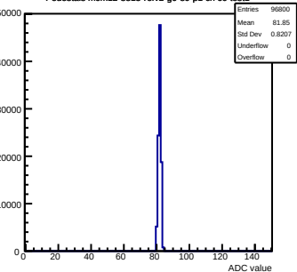
Pedestals mcm12-8815-refv2-g0-s0-p1 ch 69 test1
