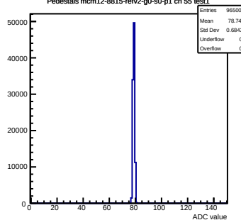
Pedestals mcm12-8815-refv2-g0-s0-p1 ch 51 test1
