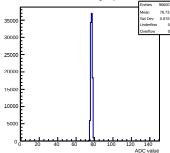
Pedestals mcm12-8815-refv2-g0-s0-p1 ch 110 test1
