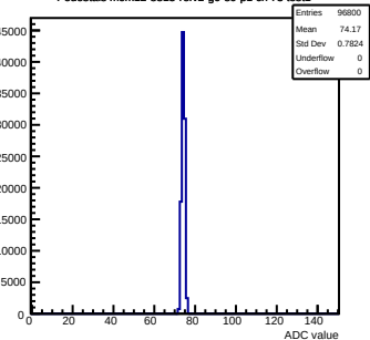
Pedestals mcm12-8815-refv2-g0-s0-p1 ch 73 test1
