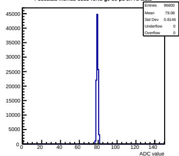
Pedestals mcm12-8815-refv2-g0-s0-p1 ch 71 test1
