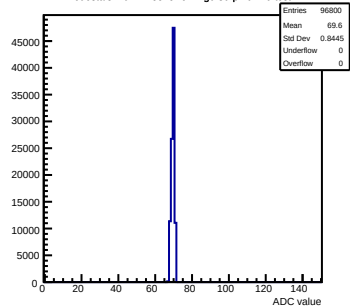
Pedestals mcm12-8815-refv2-g0-s0-p1 ch 79 test1
