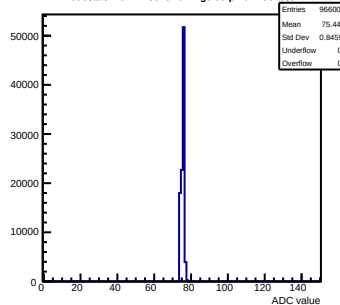
Pedestals mcm12-8815-refv2-g0-s0-p1 ch 103 test1
