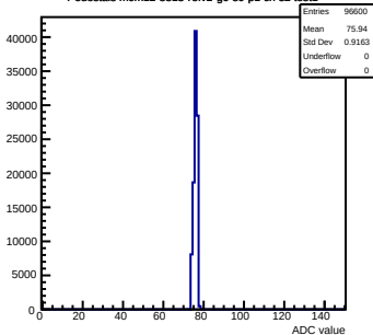
Pedestals mcm12-8815-refv2-g0-s0-p1 ch 32 test1
