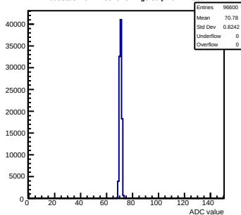
Pedestals mcm12-8815-refv2-g0-s0-p1 ch 41 test1
