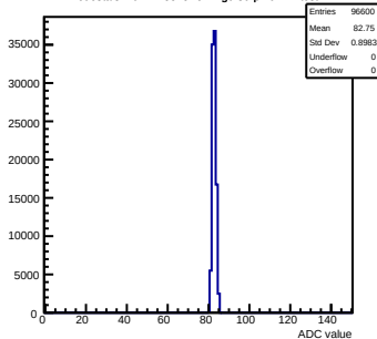
Pedestals mcm12-8815-refv2-g0-s0-p1 ch 42 test1
