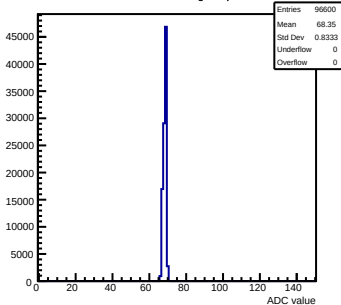
Pedestals mcm12-8815-refv2-g0-s0-p1 ch 44 test1
