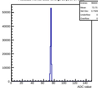
Pedestals mcm12-8815-refv2-g0-s0-p1 ch 34 test1
