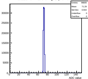
Pedestals mcm12-8815-refv2-g0-s0-p1 ch 40 test1
