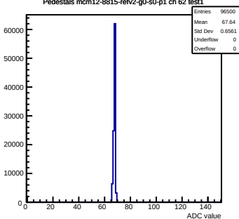
Pedestals mcm12-8815-refv2-g0-s0-p1 ch 62 test1
