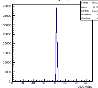
Pedestals mcm12-8815-refv2-g0-s0-p1 ch 99 test1
