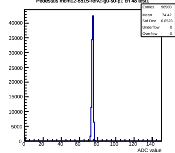
Pedestals mcm12-8815-refv2-g0-s0-p1 ch 48 test1
