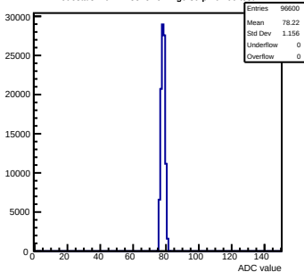
Pedestals mcm12-8815-refv2-g0-s0-p1 ch 96 test1
