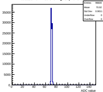
Pedestals mcm12-8815-refv2-g0-s0-p1 ch 37 test1
