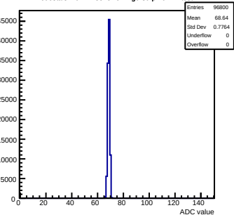
Pedestals mcm12-8815-refv2-g0-s0-p1 ch 77 test1
