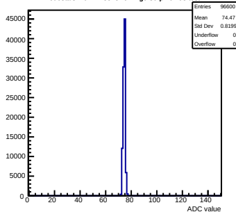
Pedestals mcm12-8815-refv2-g0-s0-p1 ch 98 test1
