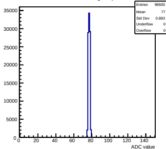
Pedestals mcm12-8815-refv2-g0-s0-p1 ch 46 test1
