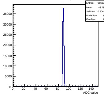
Pedestals mcm12-8815-refv2-g0-s0-p1 ch 107 test1
