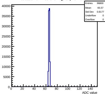
Pedestals mcm12-8815-refv2-g0-s0-p1 ch 76 test1
