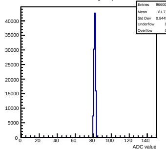
Pedestals mcm12-8815-refv2-g0-s0-p1 ch 111 test1
