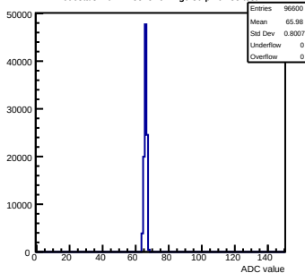
Pedestals mcm12-8815-refv2-g0-s0-p1 ch 38 test1
