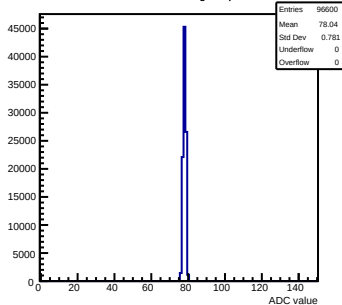
Pedestals mcm12-8815-refv2-g0-s0-p1 ch 45 test1
