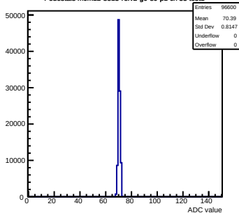
Pedestals mcm12-8815-refv2-g0-s0-p1 ch 33 test1
