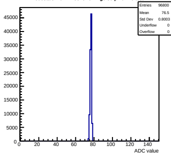
Pedestals mcm12-8815-refv2-g0-s0-p1 ch 78 test1
