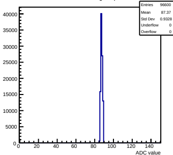
Pedestals mcm12-8815-refv2-g0-s0-p1 ch 109 test1
