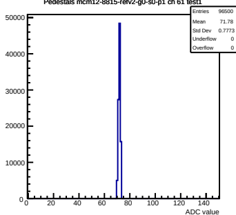
Pedestals mcm12-8815-refv2-g0-s0-p1 ch 61 test1
