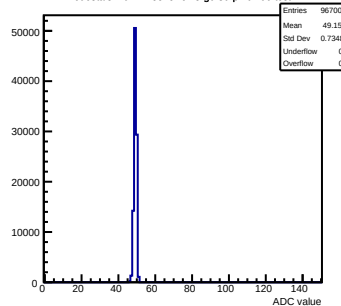
Pedestals mcm12-8815-refv3-g0-s0-p1 ch 90 test1
