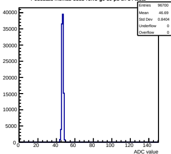
Pedestals mcm12-8815-refv3-g0-s0-p1 ch 84 test1
