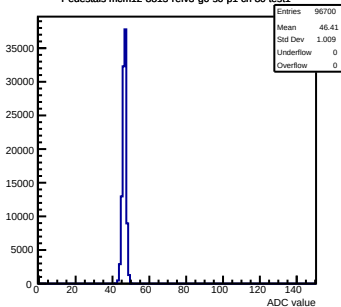
Pedestals mcm12-8815-refv3-g0-s0-p1 ch 80 test1
