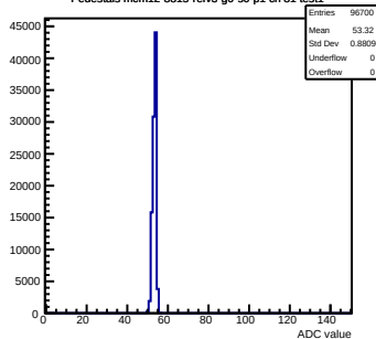
Pedestals mcm12-8815-refv3-g0-s0-p1 ch 81 test1
