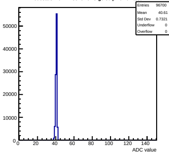
Pedestals mcm12-8815-refv3-g0-s0-p1 ch 92 test1
