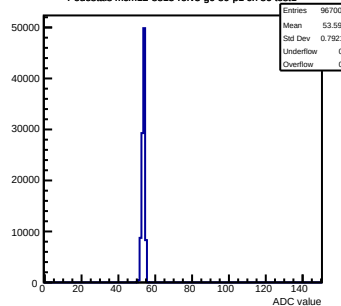
Pedestals mcm12-8815-refv3-g0-s0-p1 ch 86 test1
