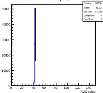
Pedestals mcm12-8815-refv3-g0-s0-p1 ch 88 test1
