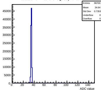
Pedestals mcm12-8815-refv3-g0-s0-p1 ch 89 test1
