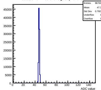
Pedestals mcm12-8815-refv3-g0-s0-p1 ch 94 test1
