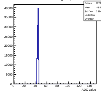
Pedestals mcm12-8815-refv3-g0-s0-p1 ch 95 test1
