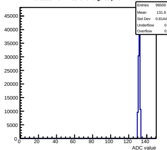
Pedestals mcm12-8815-rlv6-g0-s0-p1 ch 121 test1
