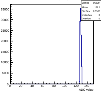
Pedestals mcm12-8815-refv6-g0-s0-p1 ch 72 test1
