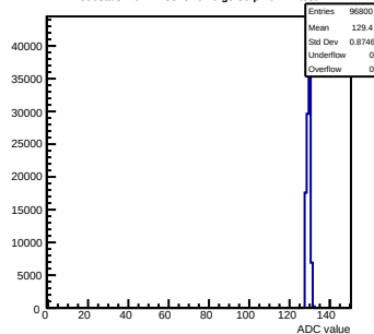
Pedestals mcm12-8815-rlfv6-g0-s0-p1 ch 14 test1
