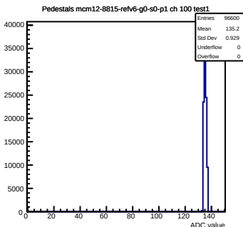
Pedestals mcm12-8815-rlv6-g0-s0-p1 ch 100 test1
