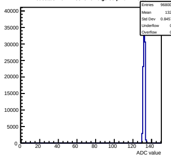
Pedestals mcm12-8815-refv6-g0-s0-p1 ch 71 test1
