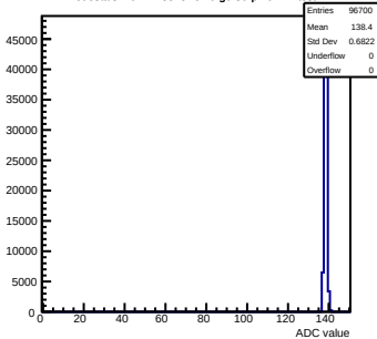
Pedestals mcm12-8815-refv6-g0-s0-p1 ch 22 test1
