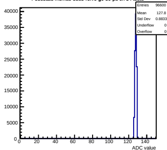
Pedestals mcm12-8815- refv6-g0-s0-p1 ch 34 test1
