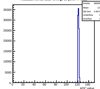
Pedestals mcm12-8815- refv6-g0-s0-p1 ch 47 test1
