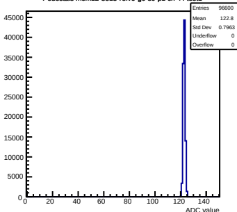
Pedestals mcm12-8815- refv6-g0-s0-p1 ch 44 test1
