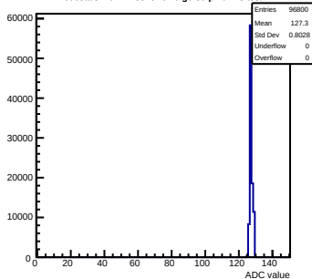
Pedestals mcm12-8815-rlfv6-g0-s0-p1 ch 13 test1
