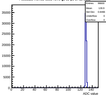
Pedestals mcm12-8815- refv6-g0-s0-p1 ch 32 test1
