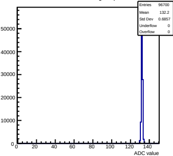
Pedestals mcm12-8815-refv6-g0-s0-p1 ch 27 test1
