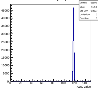
Pedestals mcm12-8815-refv6-g0-s0-p1 ch 70 test1
