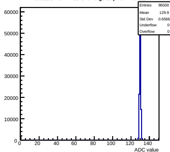
Pedestals mcm12-8815-rlv6-g0-s0-p1 ch 126 test1
