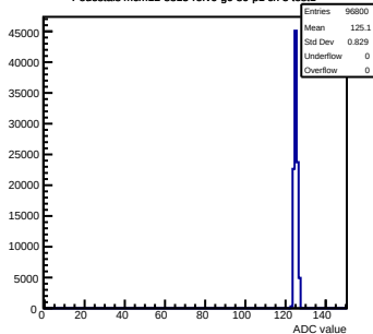
Pedestals mcm12-8815-rlfv6-g0-s0-p1 ch 5 test1
