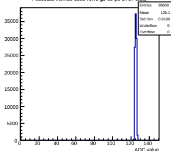
Pedestals mcm12-8815- refv6-g0-s0-p1 ch 37 test1
