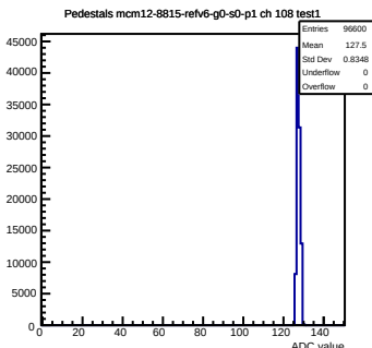
Pedestals mcm12-8815-rlv6-g0-s0-p1 ch 108 test1
