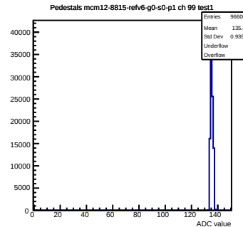
Pedestals mcm12-8815-rlv6-g0-s0-p1 ch 99 test1
