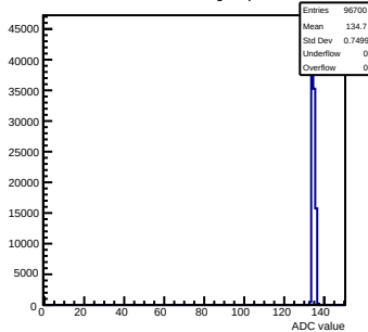
Pedestals mcm12-8815-refv6-g0-s0-p1 ch 29 test1
