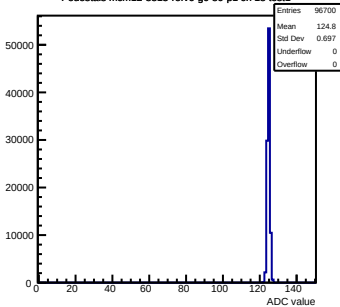
Pedestals mcm12-8815-refv6-g0-s0-p1 ch 18 test1
