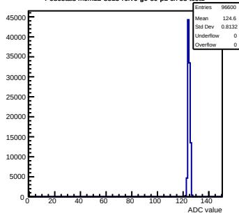
Pedestals mcm12-8815- refv6-g0-s0-p1 ch 33 test1
