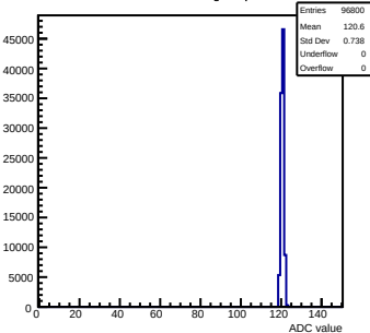
Pedestals mcm12-8815-refv6-g0-s0-p1 ch 76 test1
