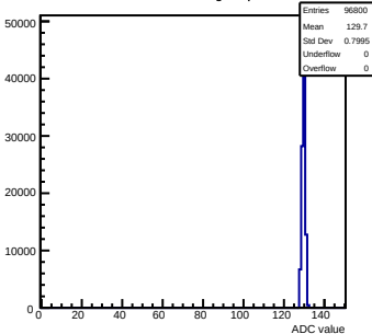
Pedestals mcm12-8815-refv6-g0-s0-p1 ch 78 test1
