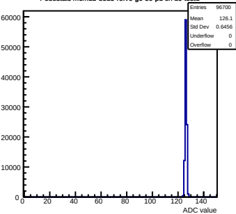
Pedestals mcm12-8815-refv6-g0-s0-p1 ch 19 test1
