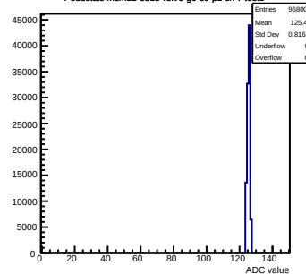
Pedestals mcm12-8815-rlfv6-g0-s0-p1 ch 7 test1
