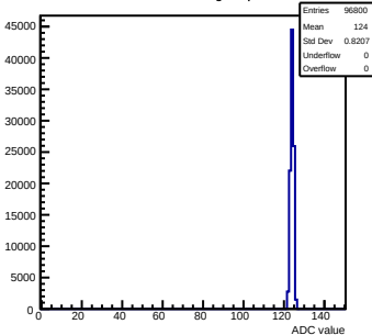
Pedestals mcm12-8815-refv6-g0-s0-p1 ch 74 test1
