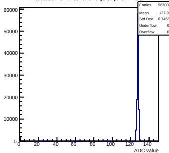
Pedestals mcm12-8815-refv6-g0-s0-p1 ch 17 test1
