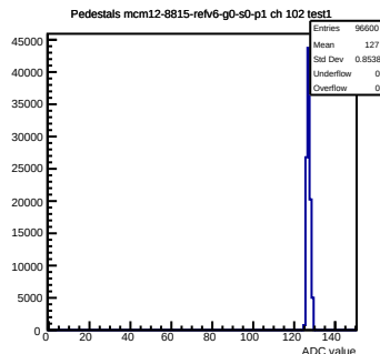
Pedestals mcm12-8815-rlv6-g0-s0-p1 ch 102 test1
