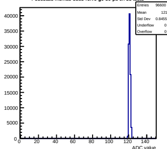
Pedestals mcm12-8815- refv6-g0-s0-p1 ch 38 test1
