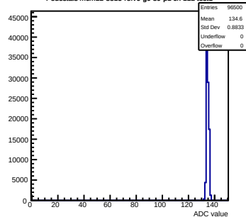
Pedestals mcm12-8815-rlv6-g0-s0-p1 ch 112 test1
