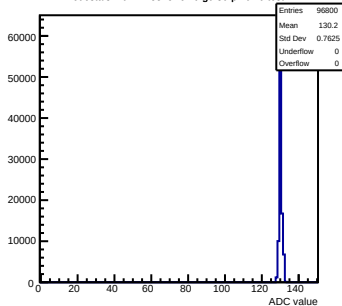
Pedestals mcm12-8815-rlfv6-g0-s0-p1 ch 9 test1
