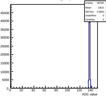
Pedestals mcm12-8815-refv6-g0-s0-p1 ch 31 test1
