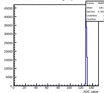
Pedestals mcm12-8815-rlfv6-g0-s0-p1 ch 11 test1
