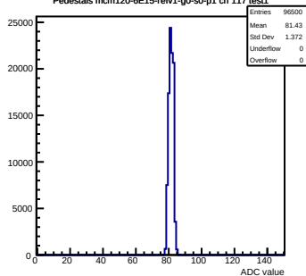
Pedestals mcm120-6E15-refv1-g0-s0-p1 ch 117 test1
