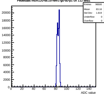
Pedestals mcm120-6E15-refv1-g0-s0-p1 ch 112 test1
