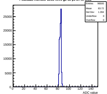
Pedestals mcm120-6E15-refv1-g0-s0-p1 ch 49 test1
