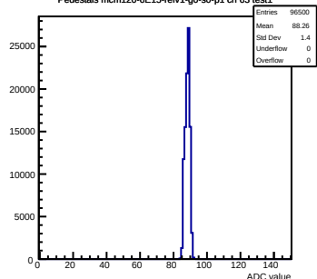
Pedestals mcm120-6E15-refv1-g0-s0-p1 ch 63 test1
