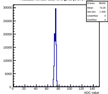
Pedestals mcm120-6E15-refv1-g0-s0-p1 ch 54 test1
