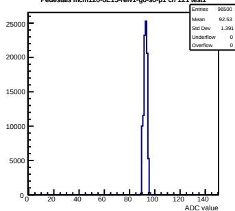
Pedestals mcm120-6E15-refv1-g0-s0-p1 ch 121 test1
