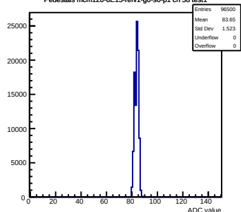
Pedestals mcm120-6E15-refv1-g0-s0-p1 ch 58 test1
