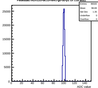
Pedestals mcm120-6E15-refv1-g0-s0-p1 ch 118 test1
