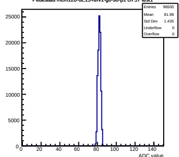
Pedestals mcm120-6E15-refv1-g0-s0-p1 ch 57 test1
