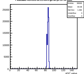
Pedestals mcm120-6E15-refv1-g0-s0-p1 ch 59 test1
