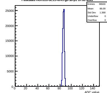
Pedestals mcm120-6E15-refv1-g0-s0-p1 ch 60 test1
