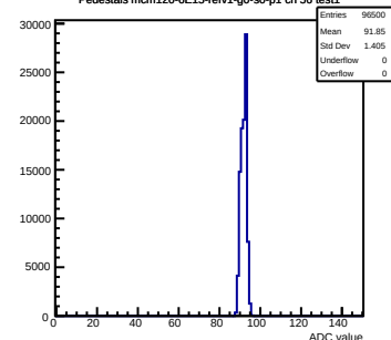
Pedestals mcm120-6E15-refv1-g0-s0-p1 ch 56 test1
