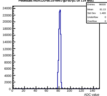
Pedestals mcm120-6E15-refv1-g0-s0-p1 ch 114 test1
