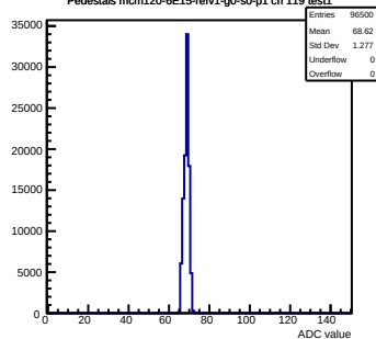
Pedestals mcm120-6E15-refv1-g0-s0-p1 ch 119 test1
