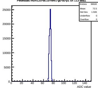
Pedestals mcm120-6E15-refv1-g0-s0-p1 ch 113 test1
