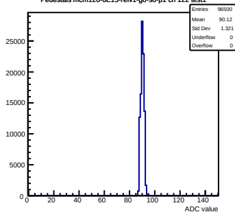
Pedestals mcm120-6E15-refv1-g0-s0-p1 ch 122 test1
