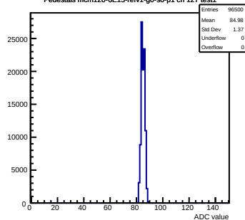
Pedestals mcm120-6E15-refv1-g0-s0-p1 ch 127 test1
