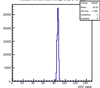
Pedestals mcm120-6E15-refv1-g0-s0-p1 ch 55 test1
