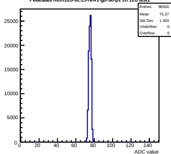
Pedestals mcm120-6E15-refv1-g0-s0-p1 ch 126 test1
