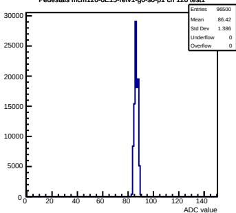
Pedestals mcm120-6E15-refv1-g0-s0-p1 ch 120 test1
