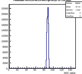
Pedestals mcm120-6E15-refv1-g0-s0-p1 ch 116 test1
