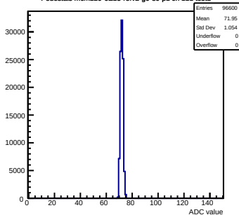
Pedestals mcm120-6E15-refv2-g0-s0-p1 ch 111 test1
