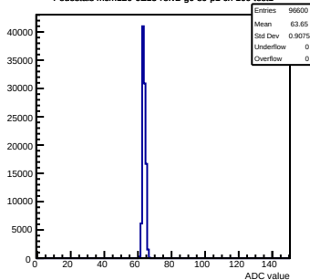
Pedestals mcm120-6E15-refv2-g0-s0-p1 ch 109 test1
