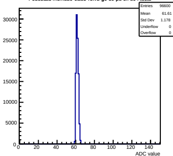
Pedestals mcm120-6E15-refv2-g0-s0-p1 ch 104 test1
