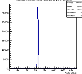
Pedestals mcm120-6E15-refv2-g0-s0-p1 ch 98 test1
