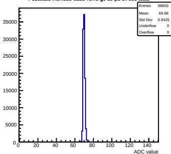
Pedestals mcm120-6E15-refv2-g0-s0-p1 ch 108 test1
