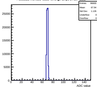
Pedestals mcm120-6E15-refv2-g0-s0-p1 ch 107 test1
