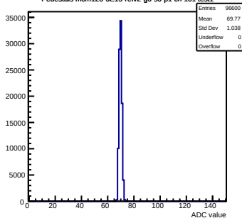
Pedestals mcm120-6E15-refv2-g0-s0-p1 ch 101 test1
