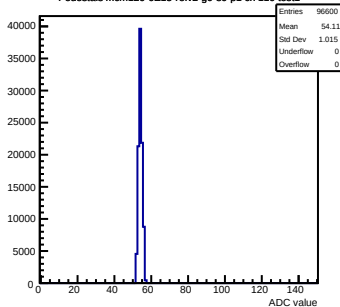
Pedestals mcm120-6E15-refv2-g0-s0-p1 ch 110 test1
