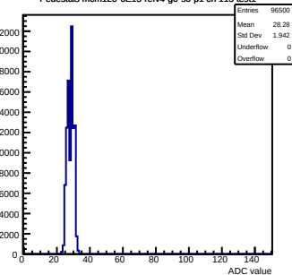
Pedestals mcm120-6E15-refV4-g0-s0-p1 ch 115 test1
