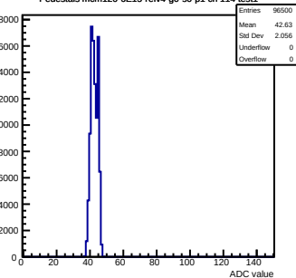
Pedestals mcm120-6E15-refV4-g0-s0-p1 ch 114 test1
