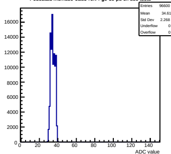
Pedestals mcm120-6E15-refv4-g0-s0-p1 ch 110 test1
