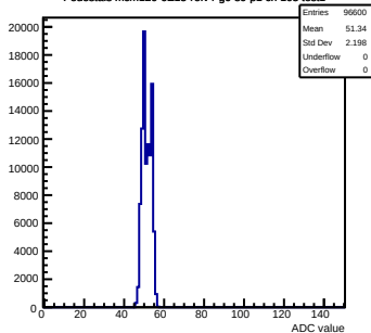
Pedestals mcm120-6E15-refv4-g0-s0-p1 ch 105 test1
