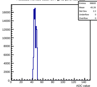
Pedestals mcm120-6E15-refv4-g0-s0-p1 ch 109 test1
