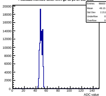
Pedestals mcm120-6E15-refv4-g0-s0-p1 ch 102 test1
