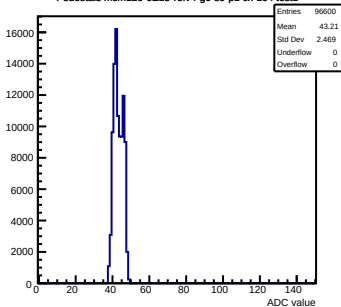
Pedestals mcm120-6E15-refv4-g0-s0-p1 ch 104 test1
