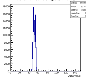
Pedestals mcm120-6E15-refv4-g0-s0-p1 ch 107 test1
