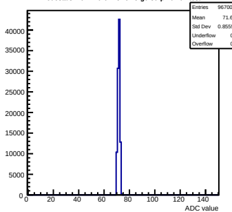
Pedestals mcm120-6E15-rfv5-g0-s0-p1 ch 91 test1
