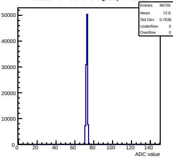
Pedestals mcm120-6E15-rfv5-g0-s0-p1 ch 88 test1
