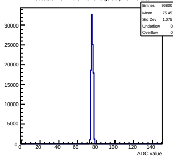
Pedestals mcm120-6E15-relv5-g0-s0-p1 ch 10 test1
