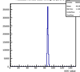
Pedestals mcm120-6E15-relv5-g0-s0-p1 ch 3 test1
