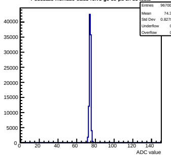
Pedestals mcm120-6E15-rfv5-g0-s0-p1 ch 83 test1
