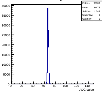
Pedestals mcm120-6E15-relv5-g0-s0-p1 ch 12 test1
