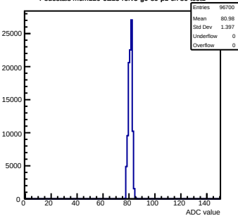
Pedestals mcm120-6E15-rfv5-g0-s0-p1 ch 80 test1
