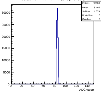
Pedestals mcm120-6E15-relv5-g0-s0-p1 ch 5 test1
