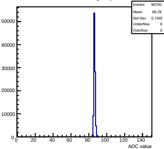
Pedestals mcm120-6E15-rfv5-g0-s0-p1 ch 92 test1
