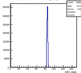
Pedestals mcm120-6E15-relv5-g0-s0-p1 ch 15 test1
