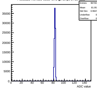
Pedestals mcm120-6E15-rfv5-g0-s0-p1 ch 82 test1
