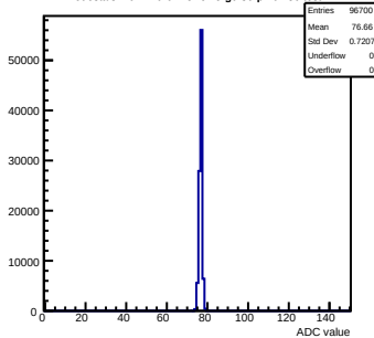
Pedestals mcm120-6E15-rfv5-g0-s0-p1 ch 86 test1
