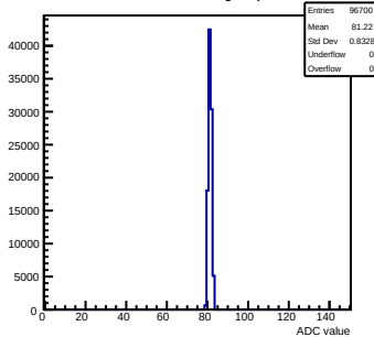
Pedestals mcm120-6E15-rfv5-g0-s0-p1 ch 94 test1
