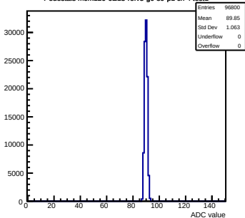
Pedestals mcm120-6E15-relv5-g0-s0-p1 ch 4 test1
