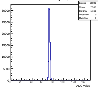
Pedestals mcm120-6E15-relv5-g0-s0-p1 ch 8 test1
