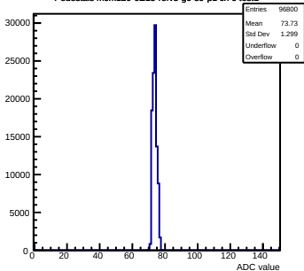
Pedestals mcm120-6E15-relv5-g0-s0-p1 ch 0 test1
