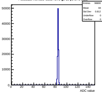
Pedestals mcm120-6E15-relv5-g0-s0-p1 ch 1 test1
