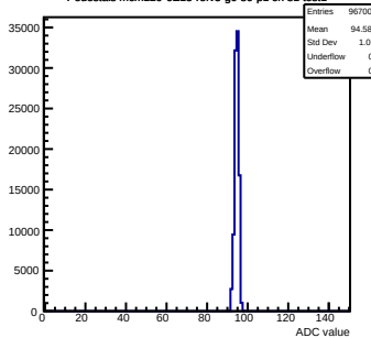
Pedestals mcm120-6E15-rfv5-g0-s0-p1 ch 81 test1
