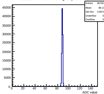
Pedestals mcm120-6E15-rfv5-g0-s0-p1 ch 90 test1
