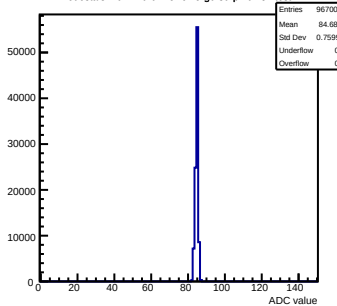
Pedestals mcm120-6E15-rfv5-g0-s0-p1 ch 87 test1
