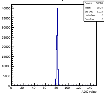
Pedestals mcm120-6E15-relv5-g0-s0-p1 ch 13 test1
