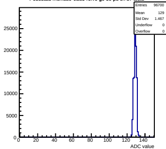
Pedestals mcm120-6E15-refv6-g0-s0-p1 ch 17 test1
