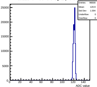
Pedestals mcm120-6E15-refv6-g0-s0-p1 ch 52 test1
