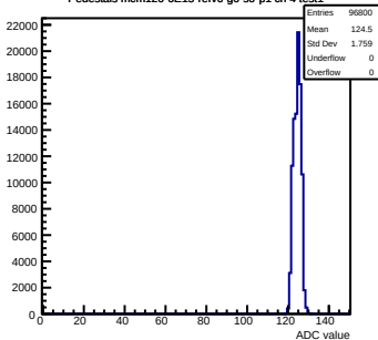
Pedestals mcm120-6E15-relv6-g0-s0-p1 ch 4 test1
