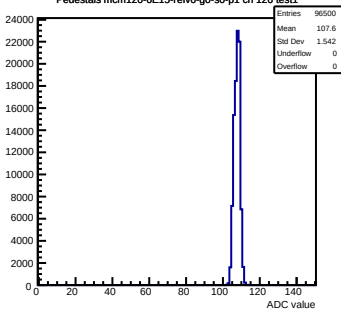
Pedestals mcm120-6E15-refv6-g0-s0-p1 ch 126 test1
