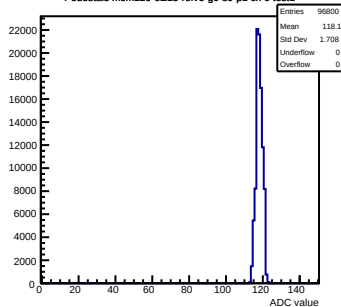
Pedestals mcm120-6E15-relv6-g0-s0-p1 ch 9 test1
