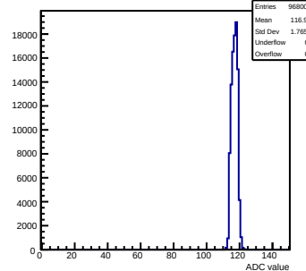
Pedestals mcm120-6E15-refv6-g0-s0-p1 ch 79 test1
