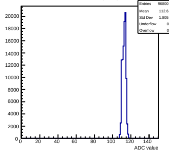
Pedestals mcm120-6E15-refv6-g0-s0-p1 ch 70 test1
