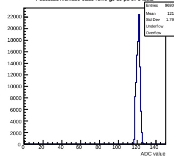
Pedestals mcm120-6E15-relv6-g0-s0-p1 ch 3 test1
