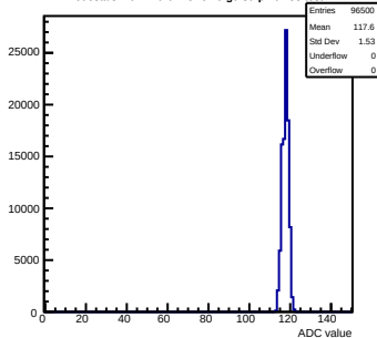
Pedestals mcm120-6E15-refv6-g0-s0-p1 ch 55 test1
