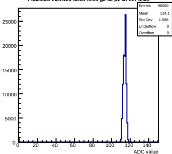
Pedestals mcm120-6E15-refv6-g0-s0-p1 ch 117 test1
