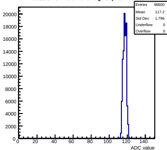
Pedestals mcm120-6E15-refv6-g0-s0-p1 ch 100 test1
