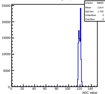
Pedestals mcm120-6E15-refv6-g0-s0-p1 ch 108 test1
