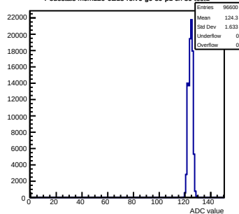
Pedestals mcm120-6E15-refv6-g0-s0-p1 ch 39 test1
