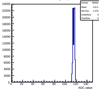
Pedestals mcm120-6E15-refv6-g0-s0-p1 ch 59 test1
