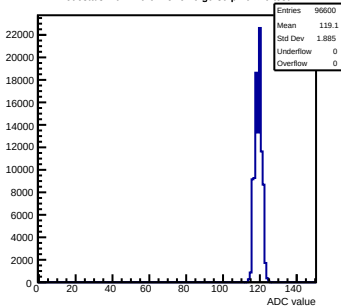
Pedestals mcm120-6E15-refv6-g0-s0-p1 ch 40 test1
