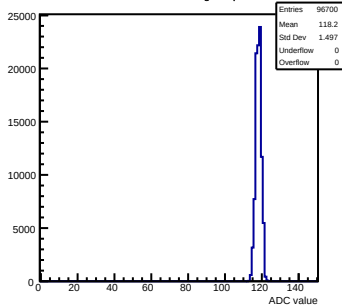
Pedestals mcm120-6E15-refv6-g0-s0-p1 ch 25 test1
