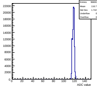
Pedestals mcm120-6E15-refv6-g0-s0-p1 ch 78 test1
