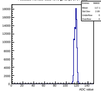
Pedestals mcm120-6E15-refv6-g0-s0-p1 ch 64 test1
