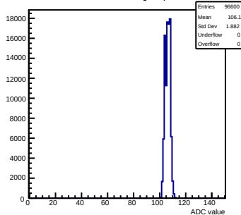
Pedestals mcm120-6E15-refv6-g0-s0-p1 ch 110 test1
