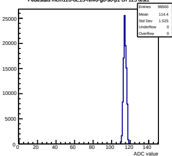
Pedestals mcm120-6E15-refv6-g0-s0-p1 ch 125 test1
