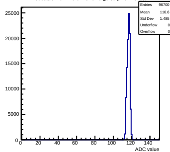
Pedestals mcm120-6E15-refv6-g0-s0-p1 ch 23 test1
