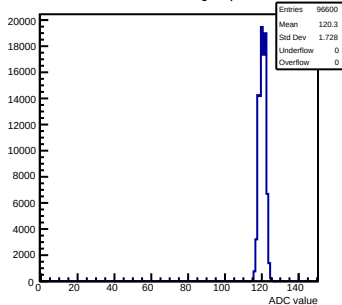
Pedestals mcm120-6E15-refv6-g0-s0-p1 ch 105 test1
