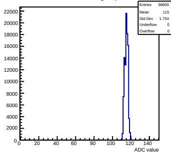
Pedestals mcm120-6E15-refv6-g0-s0-p1 ch 109 test1
