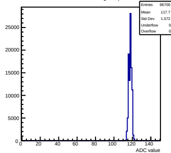
Pedestals mcm120-6E15-refv6-g0-s0-p1 ch 27 test1
