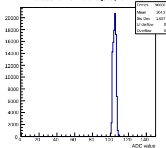
Pedestals mcm120-6E15-refv6-g0-s0-p1 ch 47 test1
