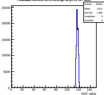
Pedestals mcm120-6E15-refv6-g0-s0-p1 ch 127 test1
