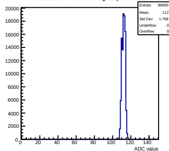
Pedestals mcm120-6E15-refv6-g0-s0-p1 ch 43 test1
