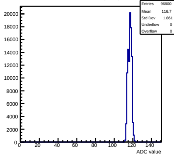
Pedestals mcm120-6E15-refv6-g0-s0-p1 ch 68 test1
