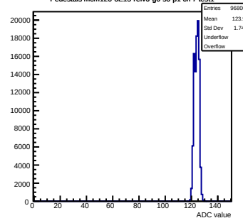
Pedestals mcm120-6E15-relv6-g0-s0-p1 ch 7 test1
