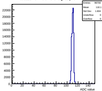
Pedestals mcm120-6E15-refv6-g0-s0-p1 ch 21 test1
