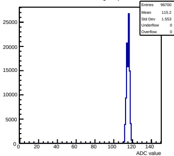
Pedestals mcm120-6E15-refv6-g0-s0-p1 ch 28 test1
