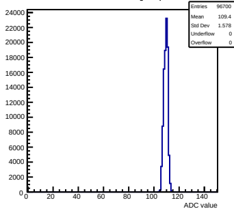
Pedestals mcm120-6E15-refv6-g0-s0-p1 ch 29 test1
