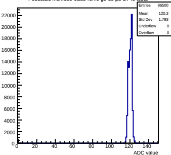
Pedestals mcm120-6E15-refv6-g0-s0-p1 ch 48 test1
