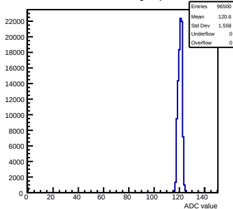
Pedestals mcm120-6E15-refv6-g0-s0-p1 ch 63 test1
