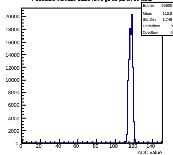
Pedestals mcm120-6E15-refv6-g0-s0-p1 ch 99 test1
