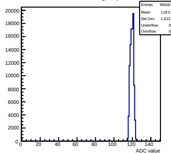
Pedestals mcm120-6E15-refv6-g0-s0-p1 ch 107 test1
