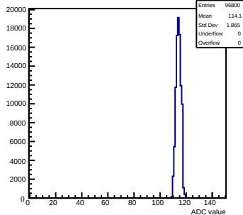
Pedestals mcm120-6E15-refv6-g0-s0-p1 ch 77 test1
