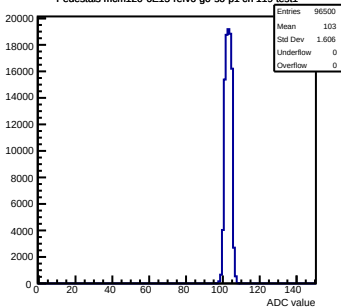
Pedestals mcm120-6E15-refv6-g0-s0-p1 ch 119 test1
