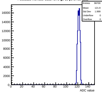
Pedestals mcm120-6E15-refv6-g0-s0-p1 ch 16 test1
