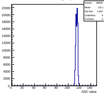
Pedestals mcm120-6E15-refv6-g0-s0-p1 ch 57 test1
