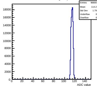
Pedestals mcm120-6E15-refv6-g0-s0-p1 ch 74 test1
