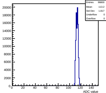
Pedestals mcm120-6E15-refv6-g0-s0-p1 ch 76 test1
