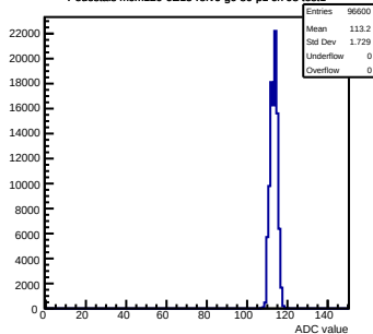
Pedestals mcm120-6E15-refv6-g0-s0-p1 ch 98 test1
