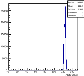
Pedestals mcm120-6E15-refv6-g0-s0-p1 ch 56 test1
