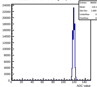
Pedestals mcm120-6E15-refv6-g0-s0-p1 ch 102 test1
