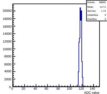
Pedestals mcm120-6E15-refv6-g0-s0-p1 ch 69 test1
