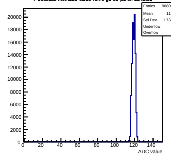
Pedestals mcm120-6E15-relv6-g0-s0-p1 ch 11 test1
