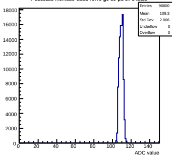
Pedestals mcm120-6E15-relv6-g0-s0-p1 ch 8 test1
