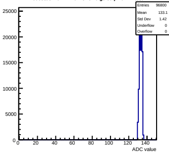
Pedestals mcm121-6413-rev0-g0-s0-p1 ch 74 test1
