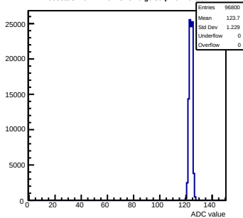
Pedestals mcm121-6413-rev0-g0-s0-p1 ch 79 test1
