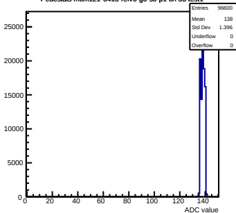
Pedestals mcm121-6413-rev0-g0-s0-p1 ch 33 test1
