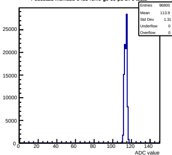
Pedestals mcm121-6413-refv0-g0-s0-p1 ch 6 test1
