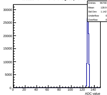
Pedestals mcm121-6413-rev0-g0-s0-p1 ch 23 test1
