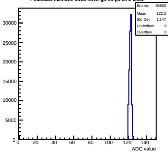
Pedestals mcm121-6413-refv0-g0-s0-p1 ch 2 test1
