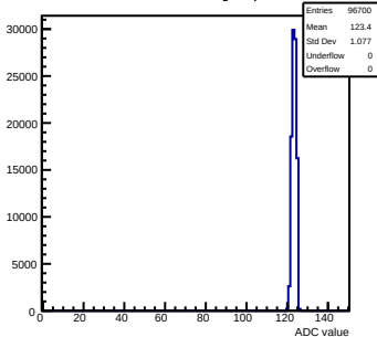
Pedestals mcm121-6413-rev0-g0-s0-p1 ch 25 test1
