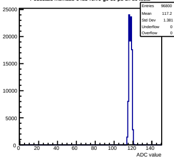
Pedestals mcm121-6413-refv0-g0-s0-p1 ch 10 test1
