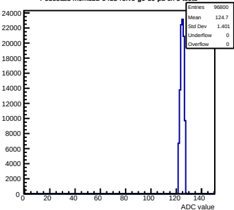
Pedestals mcm121-6413-refv0-g0-s0-p1 ch 5 test1
