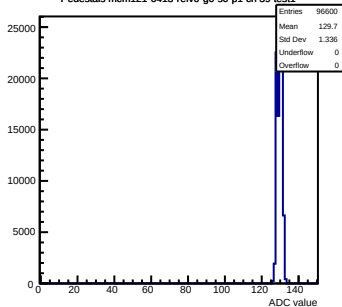
Pedestals mcm121-6413-rev0-g0-s0-p1 ch 39 test1
