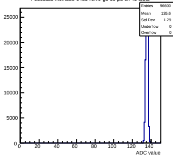
Pedestals mcm121-6413-rev0-g0-s0-p1 ch 43 test1
