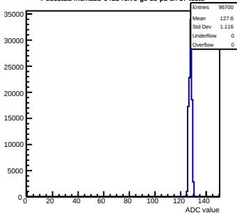
Pedestals mcm121-6413-rev0-g0-s0-p1 ch 17 test1
