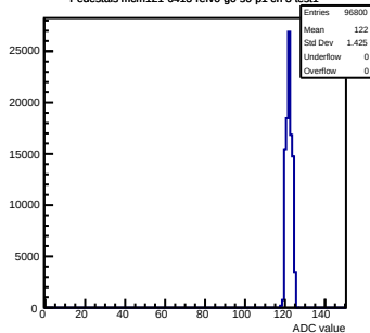
Pedestals mcm121-6413-refv0-g0-s0-p1 ch 3 test1
