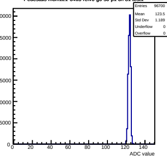
Pedestals mcm121-6413-rev0-g0-s0-p1 ch 81 test1
