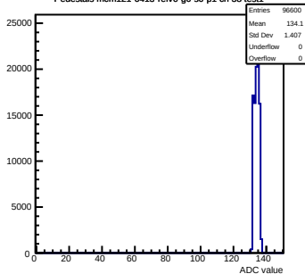
Pedestals mcm121-6413-rev0-g0-s0-p1 ch 38 test1
