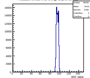
Pedestals mcm121-6413-rlv1-g0-s0-p1 ch 20 test1
