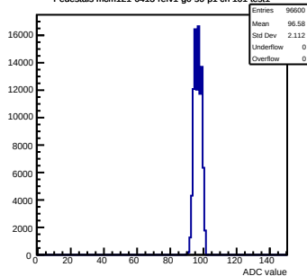
Pedestals mcm121-6413-refv1-g0-s0-p1 ch 101 test1
