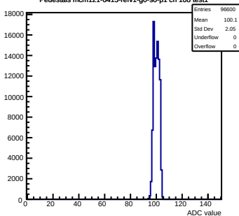
Pedestals mcm121-6413-refv1-g0-s0-p1 ch 108 test1
