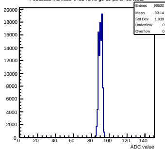
Pedestals mcm121-6413-rlv1-g0-s0-p1 ch 61 test1
