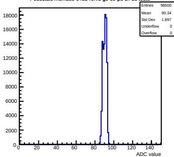
Pedestals mcm121-6413-rlv1-g0-s0-p1 ch 52 test1
