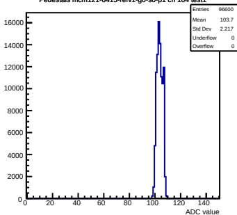
Pedestals mcm121-6413-refv1-g0-s0-p1 ch 104 test1
