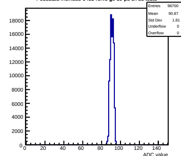
Pedestals mcm121-6413-rlv1-g0-s0-p1 ch 28 test1
