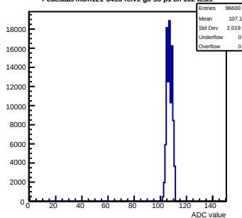
Pedestals mcm121-6413-refv1-g0-s0-p1 ch 102 test1
