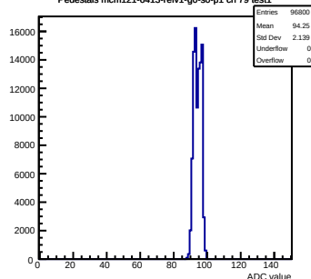
Pedestals mcm121-6413-rlv1-g0-s0-p1 ch 79 test1
