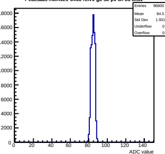
Pedestals mcm121-6413-rlv1-g0-s0-p1 ch 66 test1
