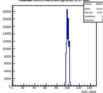
Pedestals mcm121-6413-refv1-g0-s0-p1 ch 97 test1
