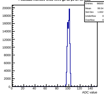
Pedestals mcm121-6413-rlv1-g0-s0-p1 ch 49 test1
