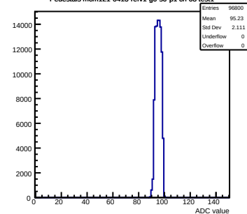
Pedestals mcm121-6413-rlv1-g0-s0-p1 ch 68 test1
