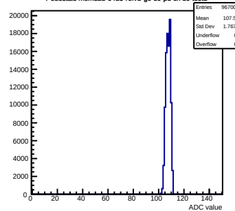
Pedestals mcm121-6413-rlv1-g0-s0-p1 ch 19 test1
