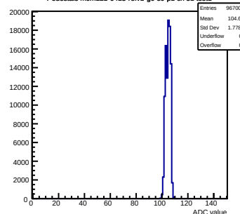
Pedestals mcm121-6413-rlv1-g0-s0-p1 ch 31 test1
