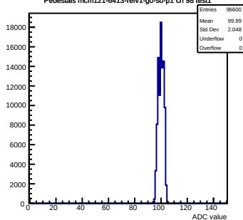
Pedestals mcm121-6413-refv1-g0-s0-p1 ch 98 test1
