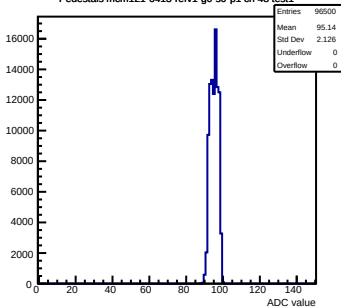
Pedestals mcm121-6413-rlv1-g0-s0-p1 ch 48 test1
