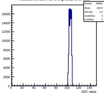
Pedestals mcm121-6413-rlv1-g0-s0-p1 ch 56 test1
