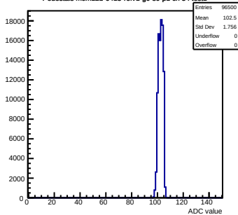
Pedestals mcm121-6413-rlv1-g0-s0-p1 ch 54 test1
