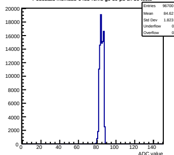
Pedestals mcm121-6413-rlv1-g0-s0-p1 ch 30 test1
