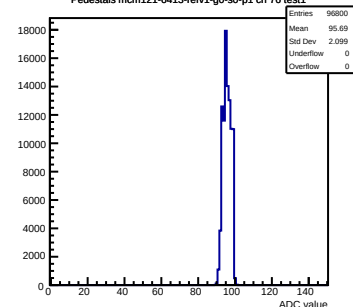
Pedestals mcm121-6413-rlv1-g0-s0-p1 ch 76 test1
