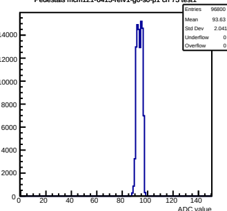
Pedestals mcm121-6413-rlv1-g0-s0-p1 ch 73 test1
