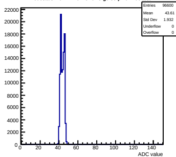
Pedestals mcm121-6413-refv3-g0-s0-p1 ch 106 test1
