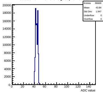
Pedestals mcm121-6413-refv3-g0-s0-p1 ch 107 test1
