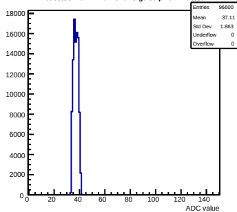
Pedestals mcm121-6413-refv3-g0-s0-p1 ch 110 test1
