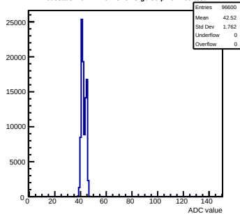
Pedestals mcm121-6413-refv3-g0-s0-p1 ch 109 test1
