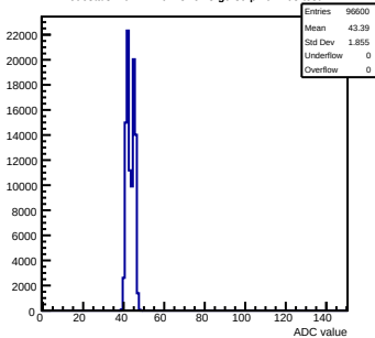
Pedestals mcm121-6413-refv3-g0-s0-p1 ch 108 test1
