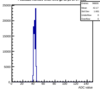
Pedestals mcm121-6413-refv3-g0-s0-p1 ch 97 test1
