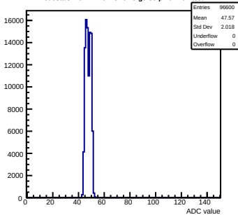
Pedestals mcm121-6413-refv3-g0-s0-p1 ch 104 test1
