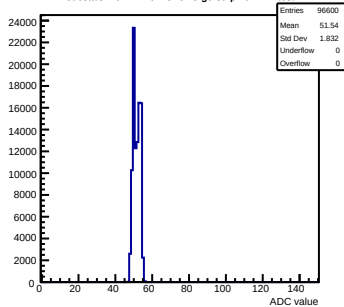
Pedestals mcm121-6413-refv3-g0-s0-p1 ch 111 test1
