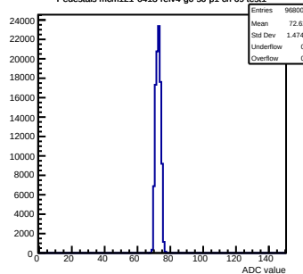
Pedestals mcm121-6413-rtv4-g0-s0-p1 ch 69 test1
