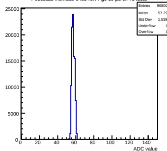
Pedestals mcm121-6413-rtv4-g0-s0-p1 ch 73 test1
