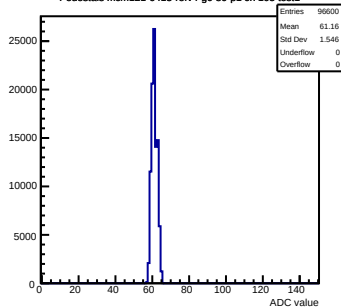
Pedestals mcm121-6413-refv4-g0-s0-p1 ch 105 test1
