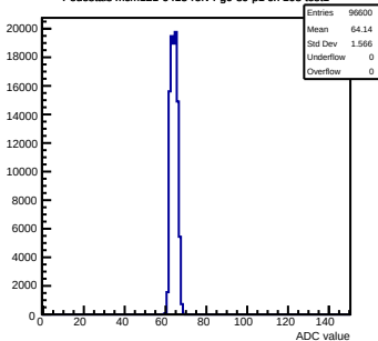
Pedestals mcm121-6413-refv4-g0-s0-p1 ch 108 test1
