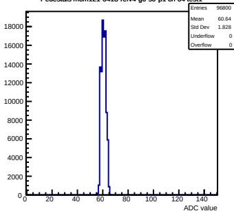
Pedestals mcm121-6413-rtv4-g0-s0-p1 ch 64 test1
