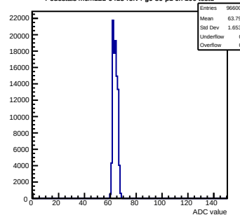
Pedestals mcm121-6413-refv4-g0-s0-p1 ch 106 test1
