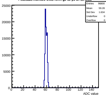
Pedestals mcm121-6413-rtv4-g0-s0-p1 ch 68 test1
