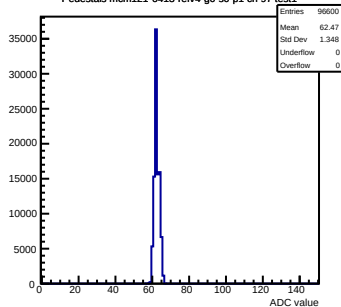
Pedestals mcm121-6413-refv4-g0-s0-p1 ch 97 test1
