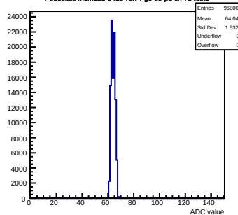
Pedestals mcm121-6413-rtv4-g0-s0-p1 ch 78 test1
