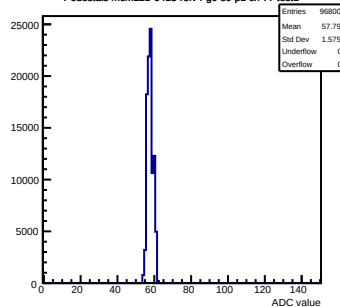
Pedestals mcm121-6413-rtv4-g0-s0-p1 ch 77 test1
