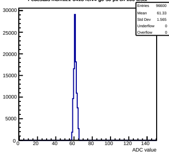
Pedestals mcm121-6413-refv4-g0-s0-p1 ch 100 test1
