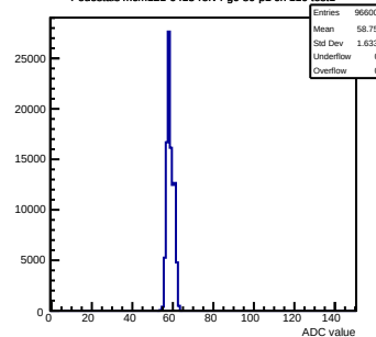
Pedestals mcm121-6413-refv4-g0-s0-p1 ch 110 test1
