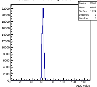
Pedestals mcm121-6413-rtv4-g0-s0-p1 ch 72 test1
