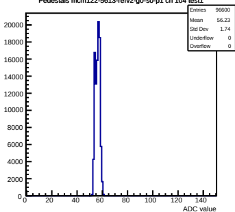
Pedestals mcm122-5613-refv2-g0-s0-p1 ch 104 test1
