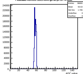
Pedestals mcm122-5613-refv2-g0-s0-p1 ch 74 test1
