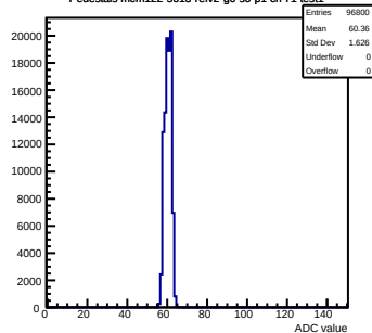
Pedestals mcm122-5613-refv2-g0-s0-p1 ch 71 test1
