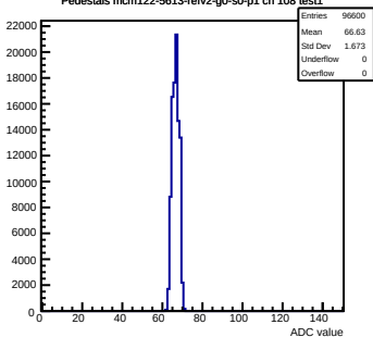
Pedestals mcm122-5613-refv2-g0-s0-p1 ch 108 test1
