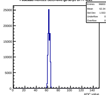
Pedestals mcm122-5613-refv2-g0-s0-p1 ch 77 test1
