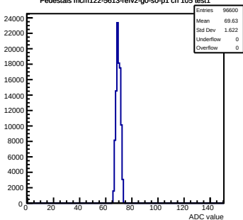
Pedestals mcm122-5613-refv2-g0-s0-p1 ch 105 test1
