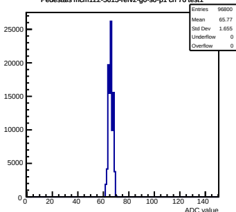
Pedestals mcm122-5613-refv2-g0-s0-p1 ch 76 test1
