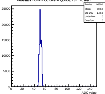
Pedestals mcm122-5613-refv2-g0-s0-p1 ch 110 test1
