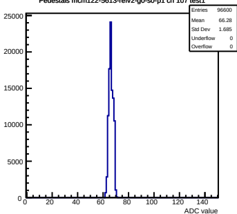
Pedestals mcm122-5613-refv2-g0-s0-p1 ch 107 test1
