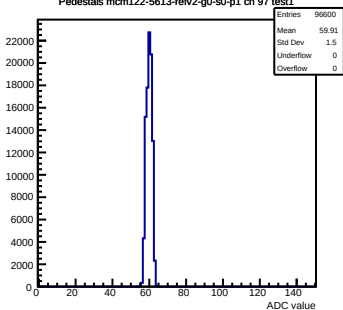
Pedestals mcm122-5613-refv2-g0-s0-p1 ch 97 test1
