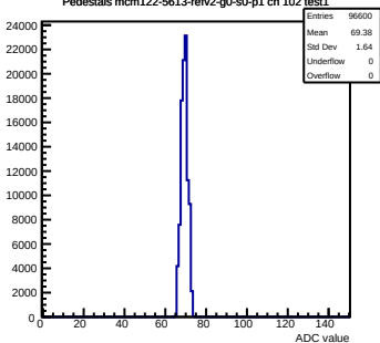
Pedestals mcm122-5613-refv2-g0-s0-p1 ch 102 test1
