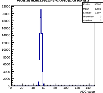
Pedestals mcm122-5613-refv2-g0-s0-p1 ch 100 test1
