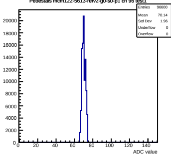
Pedestals mcm122-5613-refv2-g0-s0-p1 ch 96 test1
