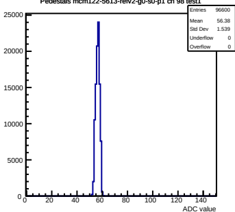
Pedestals mcm122-5613-refv2-g0-s0-p1 ch 98 test1
