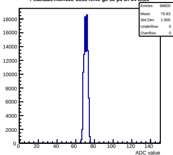
Pedestals mcm122-5613-refv2-g0-s0-p1 ch 64 test1
