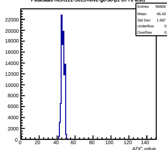
Pedestals mcm122-5613-refv2-g0-s0-p1 ch 79 test1
