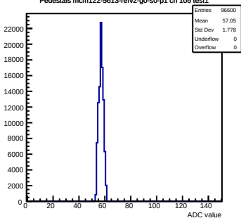
Pedestals mcm122-5613-refv2-g0-s0-p1 ch 106 test1
