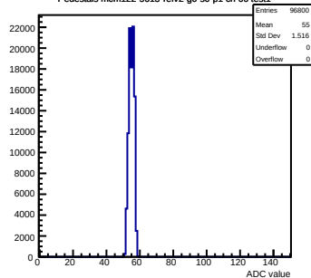
Pedestals mcm122-5613-refv2-g0-s0-p1 ch 66 test1
