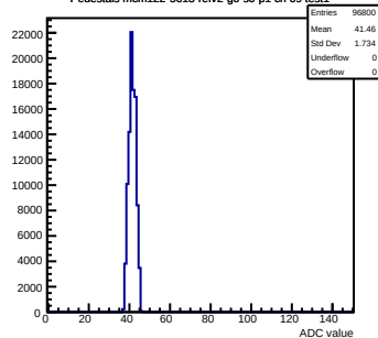
Pedestals mcm122-5613-refv2-g0-s0-p1 ch 69 test1
