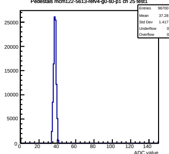
Pedestals mcm122-5613-refv4-g0-s0-p1 ch 25 test1
