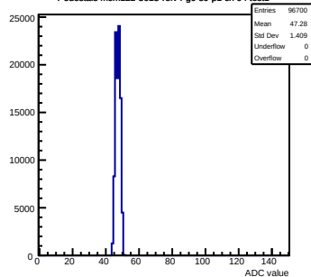
Pedestals mcm122-5613-recv4-g0-s0-p1 ch 94 test1
