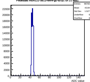
Pedestals mcm122-5613-refv4-g0-s0-p1 ch 21 test1
