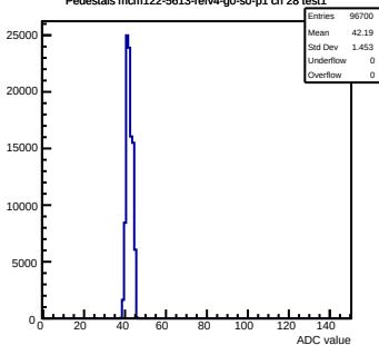
Pedestals mcm122-5613-refv4-g0-s0-p1 ch 28 test1
