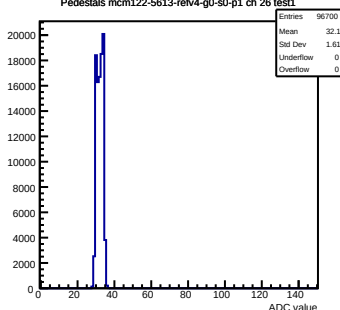
Pedestals mcm122-5613-refv4-g0-s0-p1 ch 26 test1
