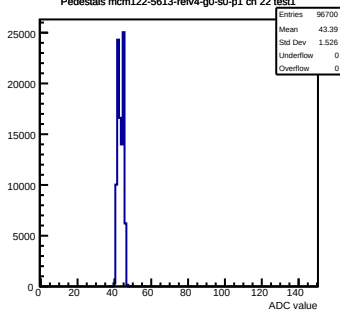
Pedestals mcm122-5613-refv4-g0-s0-p1 ch 22 test1
