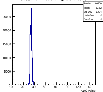
Pedestals mcm122-5613-recv4-g0-s0-p1 ch 93 test1
