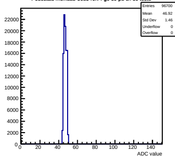
Pedestals mcm122-5613-recv4-g0-s0-p1 ch 89 test1
