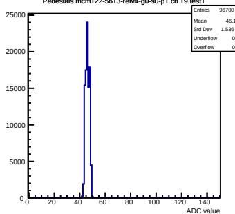
Pedestals mcm122-5613-refv4-g0-s0-p1 ch 19 test1
