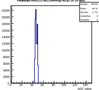
Pedestals mcm122-5613-refv4-g0-s0-p1 ch 20 test1
