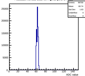
Pedestals mcm122-5613-recv4-g0-s0-p1 ch 84 test1
