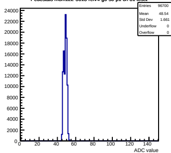
Pedestals mcm122-5613-recv4-g0-s0-p1 ch 81 test1
