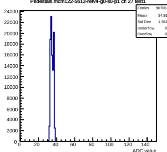
Pedestals mcm122-5613-refv4-g0-s0-p1 ch 27 test1
