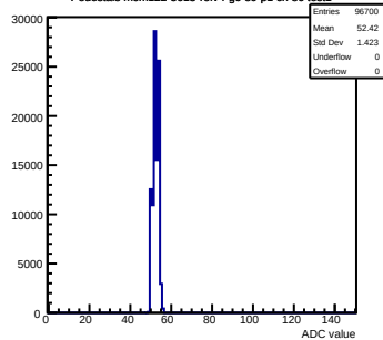
Pedestals mcm122-5613-recv4-g0-s0-p1 ch 86 test1
