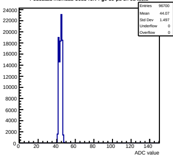
Pedestals mcm122-5613-recv4-g0-s0-p1 ch 92 test1
