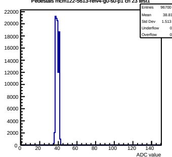
Pedestals mcm122-5613-refv4-g0-s0-p1 ch 23 test1
