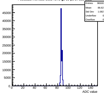
Pedestals mcm122-5613-refv5-g0-s0-p1 ch 118 test1
