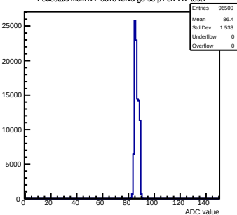
Pedestals mcm122-5613-refv5-g0-s0-p1 ch 112 test1
