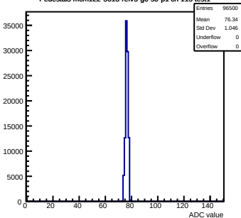
Pedestals mcm122-5613-refv5-g0-s0-p1 ch 115 test1
