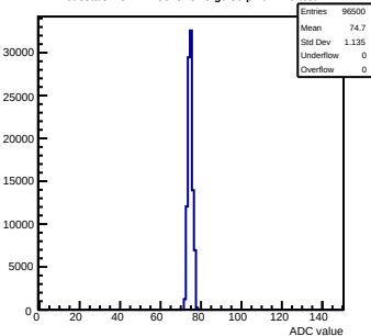
Pedestals mcm122-5613-refv5-g0-s0-p1 ch 125 test1
