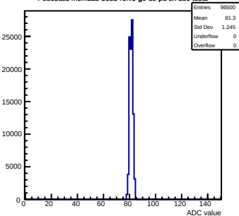
Pedestals mcm122-5613-refv5-g0-s0-p1 ch 116 test1
