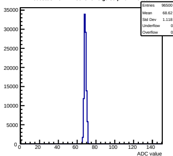
Pedestals mcm122-5613-refv5-g0-s0-p1 ch 126 test1
