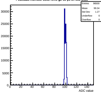
Pedestals mcm122-5613-refv5-g0-s0-p1 ch 113 test1
