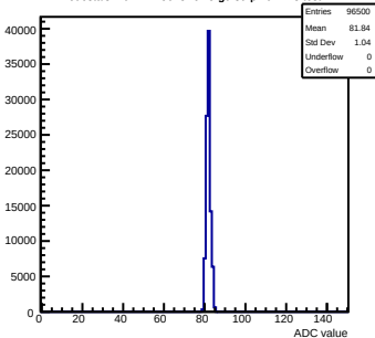
Pedestals mcm122-5613-refv5-g0-s0-p1 ch 123 test1
