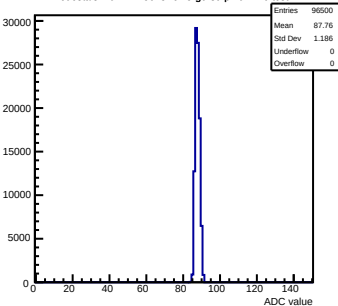
Pedestals mcm122-5613-refv5-g0-s0-p1 ch 120 test1
