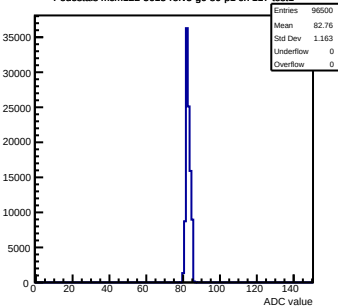
Pedestals mcm122-5613-refv5-g0-s0-p1 ch 117 test1
