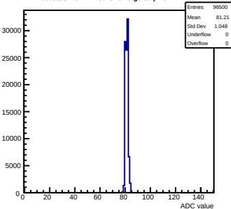
Pedestals mcm122-5613-refv5-g0-s0-p1 ch 124 test1
