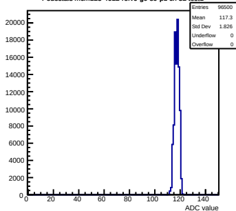
Pedestals mcm123-4612-refv0-g0-s0-p1 ch 52 test1
