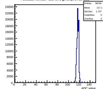
Pedestals mcm123-4612-refv0-g0-s0-p1 ch 92 test1
