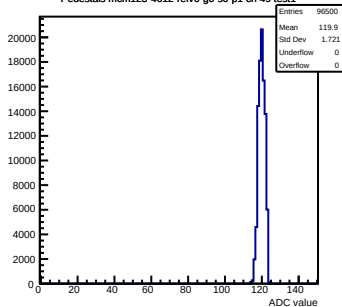
Pedestals mcm123-4612-refv0-g0-s0-p1 ch 49 test1
