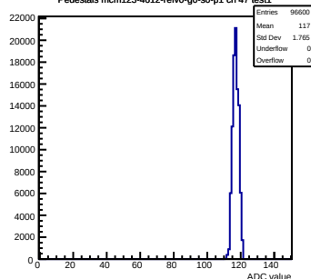
Pedestals mcm123-4612-refv0-g0-s0-p1 ch 47 test1
