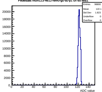
Pedestals mcm123-4612-refv0-g0-s0-p1 ch 65 test1
