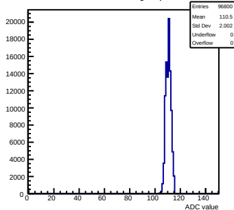
Pedestals mcm123-4612-refV0-g0-s0-p1 ch 10 test1
