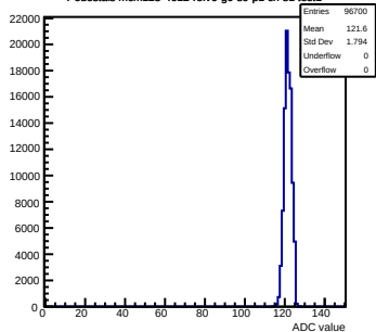
Pedestals mcm123-4612-refv0-g0-s0-p1 ch 81 test1
