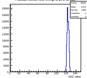
Pedestals mcm123-4612-refv0-g0-s0-p1 ch 33 test1
