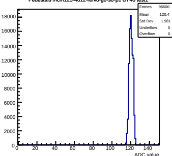
Pedestals mcm123-4612-refv0-g0-s0-p1 ch 40 test1
