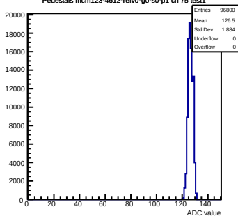
Pedestals mcm123-4612-refv0-g0-s0-p1 ch 75 test1
