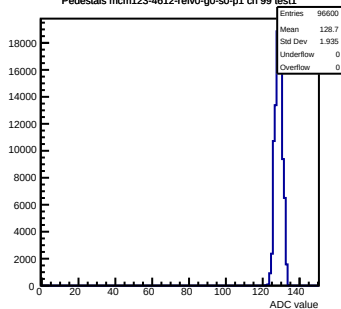
Pedestals mcm123-4612-refV0-g0-s0-p1 ch 99 test1
