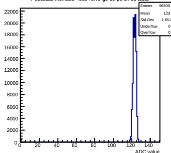
Pedestals mcm123-4612-refv0-g0-s0-p1 ch 58 test1
