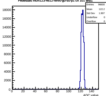
Pedestals mcm123-4612-refV0-g0-s0-p1 ch 101 test1
