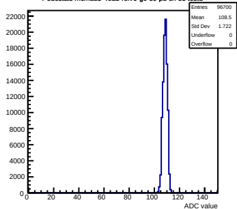
Pedestals mcm123-4612-refv0-g0-s0-p1 ch 85 test1
