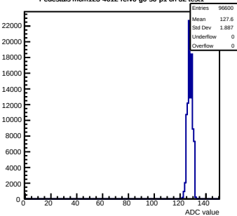
Pedestals mcm123-4612-refv0-g0-s0-p1 ch 32 test1
