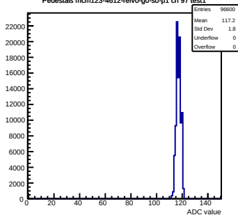
Pedestals mcm123-4612-refV0-g0-s0-p1 ch 97 test1
