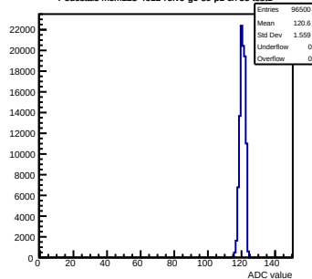
Pedestals mcm123-4612-refv0-g0-s0-p1 ch 55 test1
