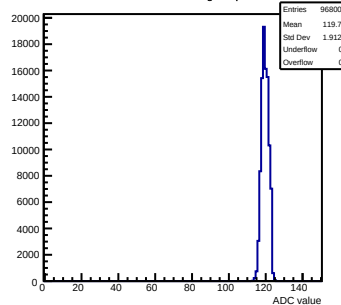
Pedestals mcm123-4612-refV0-g0-s0-p1 ch 15 test1
