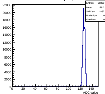
Pedestals mcm123-4612-refV0-g0-s0-p1 ch 6 test1
