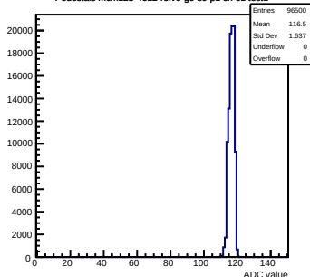
Pedestals mcm123-4612-refv0-g0-s0-p1 ch 61 test1
