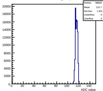
Pedestals mcm123-4612-refV0-g0-s0-p1 ch 13 test1
