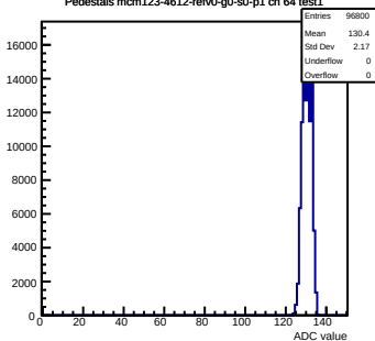
Pedestals mcm123-4612-refv0-g0-s0-p1 ch 64 test1
