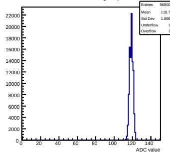
Pedestals mcm123-4612-refV0-g0-s0-p1 ch 11 test1
