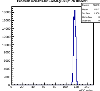
Pedestals mcm123-4612-refV0-g0-s0-p1 ch 106 test1
