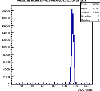
Pedestals mcm123-4612-refv0-g0-s0-p1 ch 68 test1
