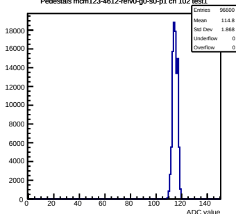
Pedestals mcm123-4612-refV0-g0-s0-p1 ch 102 test1
