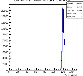
Pedestals mcm123-4612-refv0-g0-s0-p1 ch 76 test1
