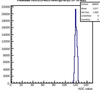
Pedestals mcm123-4612-refv0-g0-s0-p1 ch 78 test1
