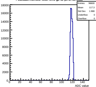
Pedestals mcm123-4612-refv0-g0-s0-p1 ch 36 test1
