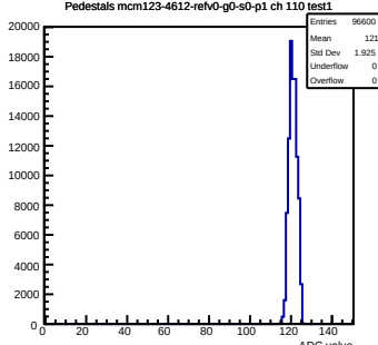
Pedestals mcm123-4612-refV0-g0-s0-p1 ch 110 test1
