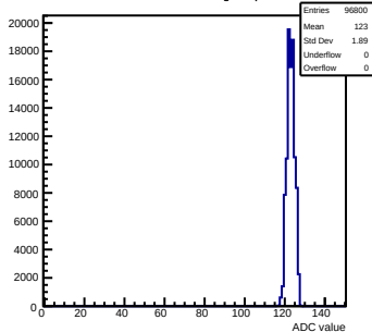
Pedestals mcm123-4612-refV0-g0-s0-p1 ch 9 test1
