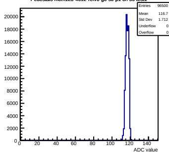
Pedestals mcm123-4612-refv0-g0-s0-p1 ch 50 test1
