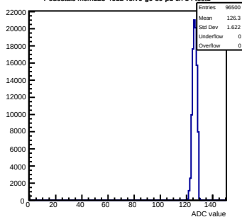
Pedestals mcm123-4612-refv0-g0-s0-p1 ch 54 test1
