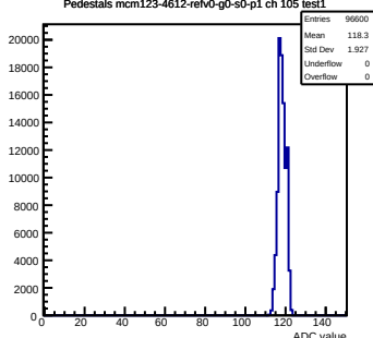
Pedestals mcm123-4612-refV0-g0-s0-p1 ch 105 test1
