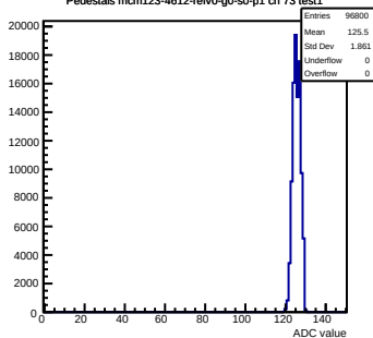
Pedestals mcm123-4612-refv0-g0-s0-p1 ch 73 test1
