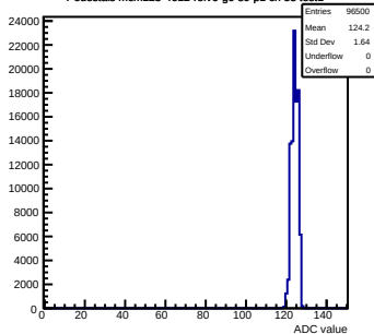
Pedestals mcm123-4612-refv0-g0-s0-p1 ch 53 test1
