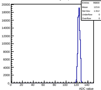
Pedestals mcm123-4612-refV0-g0-s0-p1 ch 12 test1
