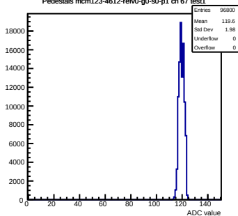
Pedestals mcm123-4612-refv0-g0-s0-p1 ch 67 test1
