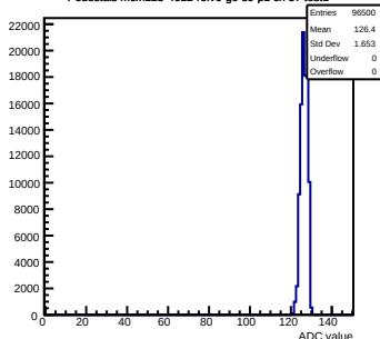
Pedestals mcm123-4612-refv0-g0-s0-p1 ch 57 test1
