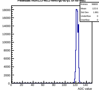
Pedestals mcm123-4612-refv0-g0-s0-p1 ch 69 test1
