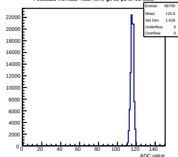
Pedestals mcm123-4612-refv0-g0-s0-p1 ch 91 test1
