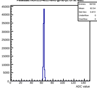
Pedestals mcm123-4612-refv2-g0-s0-p1 ch 92 test1
