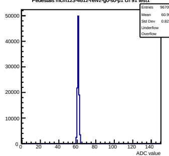
Pedestals mcm123-4612-refv2-g0-s0-p1 ch 91 test1
