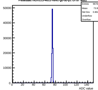
Pedestals mcm123-4612-refv2-g0-s0-p1 ch 87 test1
