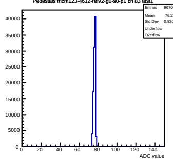
Pedestals mcm123-4612-refv2-g0-s0-p1 ch 83 test1
