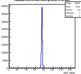
Pedestals mcm123-4612-refv2-g0-s0-p1 ch 84 test1
