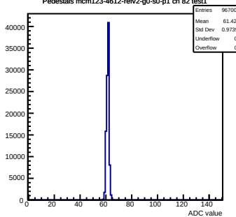
Pedestals mcm123-4612-refv2-g0-s0-p1 ch 82 test1
