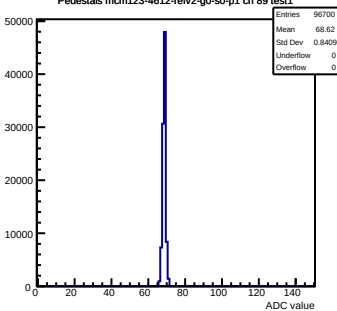
Pedestals mcm123-4612-refv2-g0-s0-p1 ch 89 test1
