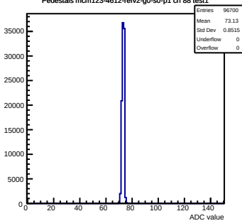
Pedestals mcm123-4612-refv2-g0-s0-p1 ch 88 test1
