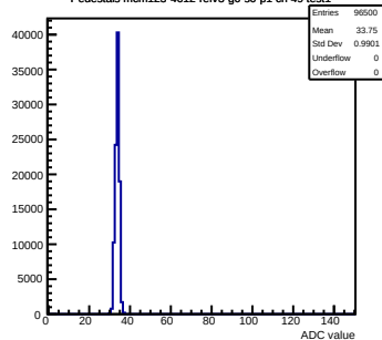
Pedestals mcm123-4612-refv3-g0-s0-p1 ch 49 test1
