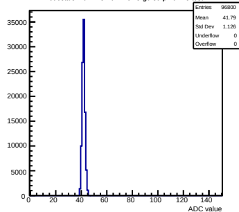
Pedestals mcm123-4612-refv3-g0-s0-p1 ch 75 test1
