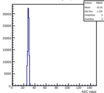
Pedestals mcm123-4612-refv3-g0-s0-p1 ch 77 test1
