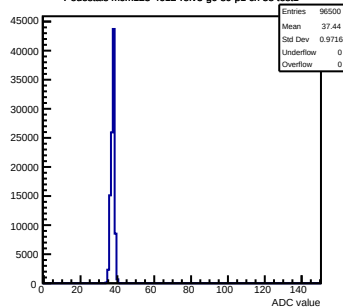
Pedestals mcm123-4612-refv3-g0-s0-p1 ch 58 test1
