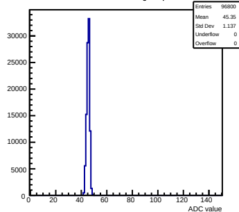
Pedestals mcm123-4612-refv3-g0-s0-p1 ch 79 test1
