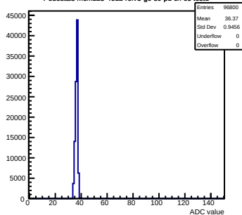
Pedestals mcm123-4612-refv3-g0-s0-p1 ch 65 test1
