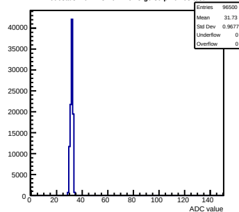
Pedestals mcm123-4612-refv3-g0-s0-p1 ch 63 test1
