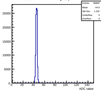
Pedestals mcm123-4612-refv3-g0-s0-p1 ch 74 test1
