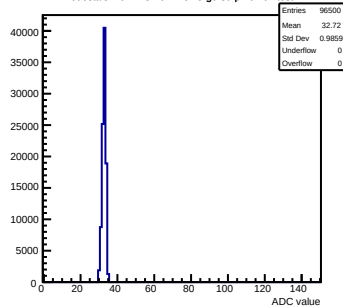
Pedestals mcm123-4612-refv3-g0-s0-p1 ch 62 test1
