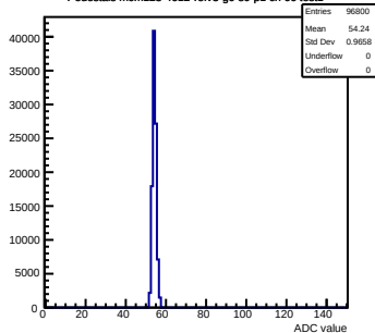
Pedestals mcm123-4612-refv3-g0-s0-p1 ch 66 test1
