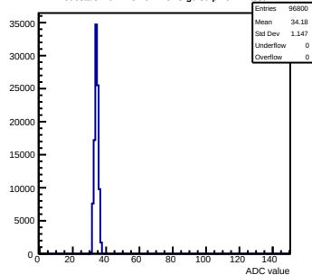
Pedestals mcm123-4612-refv3-g0-s0-p1 ch 71 test1
