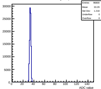
Pedestals mcm123-4612-refv3-g0-s0-p1 ch 78 test1
