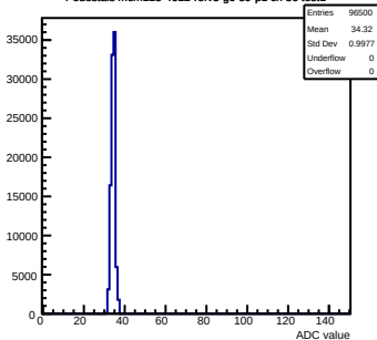
Pedestals mcm123-4612-refv3-g0-s0-p1 ch 56 test1
