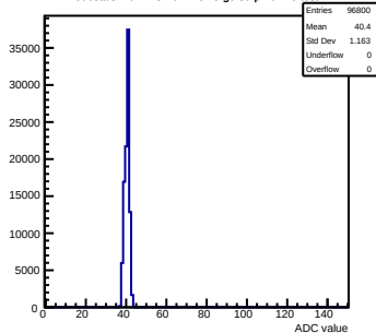
Pedestals mcm123-4612-refv3-g0-s0-p1 ch 70 test1
