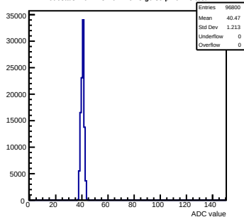
Pedestals mcm123-4612-refv3-g0-s0-p1 ch 73 test1
