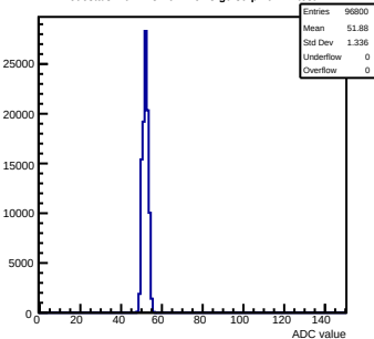
Pedestals mcm123-4612-refv3-g0-s0-p1 ch 72 test1
