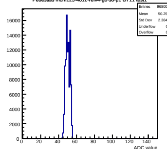
Pedestals mcm123-4612-refv4-g0-s0-p1 ch 11 test1
