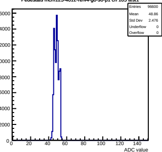
Pedestals mcm123-4612-refv4-g0-s0-p1 ch 105 test1
