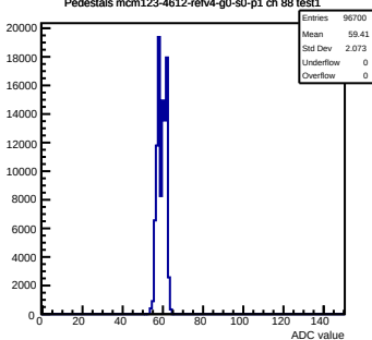
Pedestals mcm123-4612-refv4-g0-s0-p1 ch 88 test1
