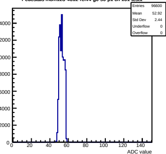
Pedestals mcm123-4612-refv4-g0-s0-p1 ch 101 test1
