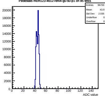
Pedestals mcm123-4612-refv4-g0-s0-p1 ch 95 test1
