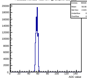
Pedestals mcm123-4612-refv4-g0-s0-p1 ch 123 test1
