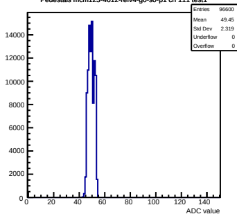
Pedestals mcm123-4612-refv4-g0-s0-p1 ch 111 test1
