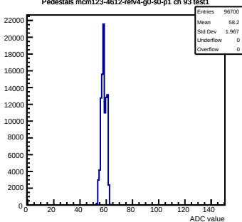
Pedestals mcm123-4612-refv4-g0-s0-p1 ch 93 test1
