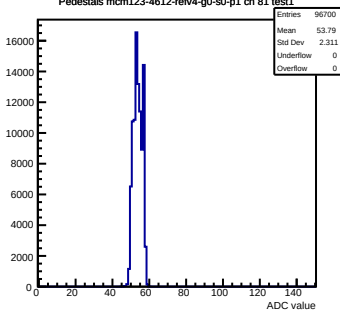
Pedestals mcm123-4612-refv4-g0-s0-p1 ch 81 test1
