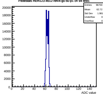
Pedestals mcm123-4612-refv4-g0-s0-p1 ch 94 test1
