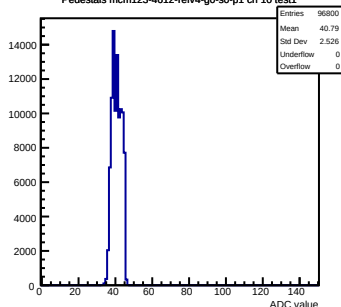
Pedestals mcm123-4612-refv4-g0-s0-p1 ch 10 test1
