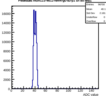
Pedestals mcm123-4612-refv4-g0-s0-p1 ch 85 test1
