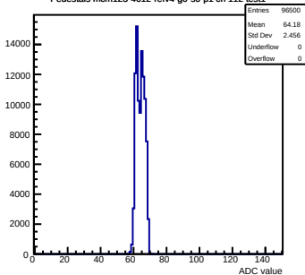
Pedestals mcm123-4612-refv4-g0-s0-p1 ch 112 test1
