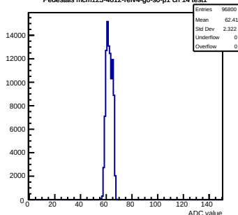
Pedestals mcm123-4612-refv4-g0-s0-p1 ch 14 test1
