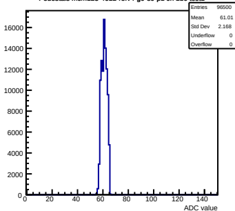
Pedestals mcm123-4612-refv4-g0-s0-p1 ch 116 test1
