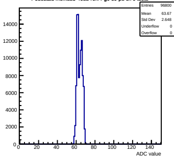
Pedestals mcm123-4612-refv4-g0-s0-p1 ch 0 test1
