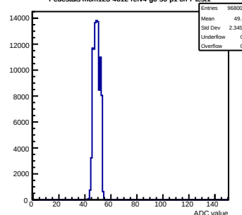
Pedestals mcm123-4612-refv4-g0-s0-p1 ch 7 test1
