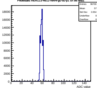
Pedestals mcm123-4612-refv4-g0-s0-p1 ch 86 test1
