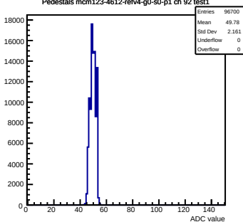
Pedestals mcm123-4612-refv4-g0-s0-p1 ch 92 test1
