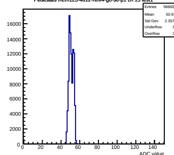
Pedestals mcm123-4612-refv4-g0-s0-p1 ch 15 test1
