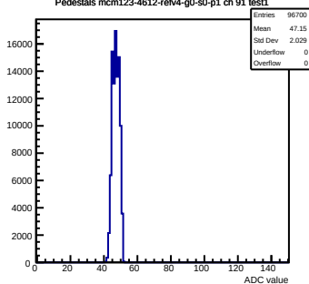
Pedestals mcm123-4612-refv4-g0-s0-p1 ch 91 test1
