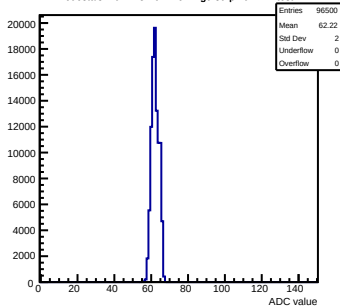
Pedestals mcm123-4612-refv4-g0-s0-p1 ch 127 test1
