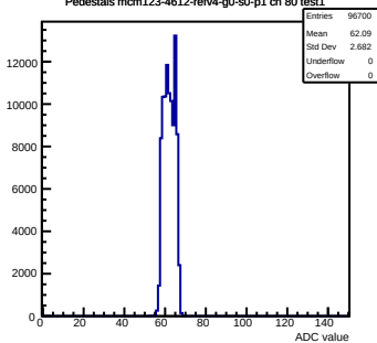
Pedestals mcm123-4612-refv4-g0-s0-p1 ch 80 test1
