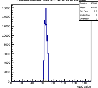
Pedestals mcm123-4612-refv4-g0-s0-p1 ch 103 test1
