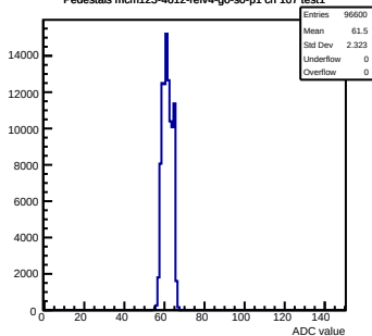
Pedestals mcm123-4612-refv4-g0-s0-p1 ch 107 test1
