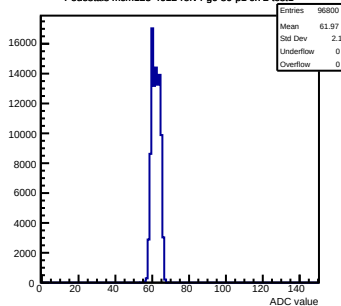
Pedestals mcm123-4612-refv4-g0-s0-p1 ch 2 test1
