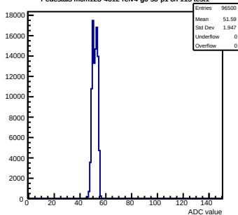
Pedestals mcm123-4612-refv4-g0-s0-p1 ch 115 test1
