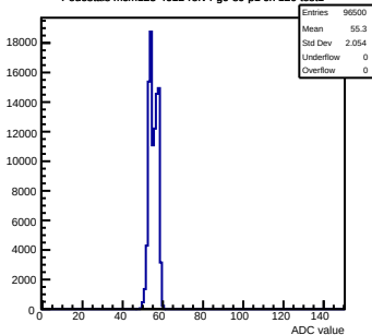
Pedestals mcm123-4612-refv4-g0-s0-p1 ch 120 test1
