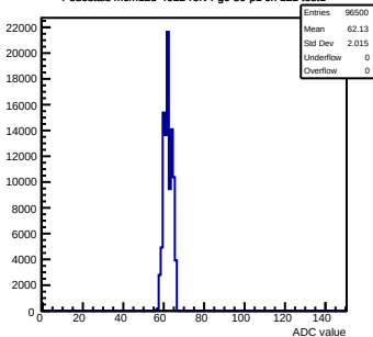
Pedestals mcm123-4612-refv4-g0-s0-p1 ch 122 test1
