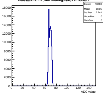
Pedestals mcm123-4612-refv4-g0-s0-p1 ch 98 test1
