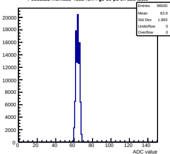
Pedestals mcm123-4612-refv4-g0-s0-p1 ch 121 test1
