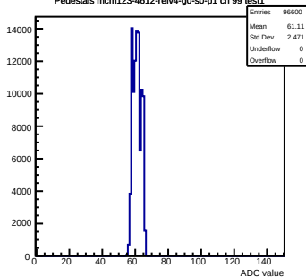
Pedestals mcm123-4612-refv4-g0-s0-p1 ch 99 test1
