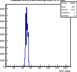
Pedestals mcm123-4612-refv4-g0-s0-p1 ch 97 test1
