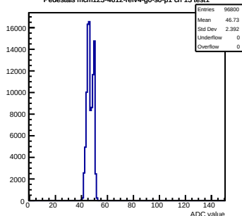
Pedestals mcm123-4612-refv4-g0-s0-p1 ch 13 test1
