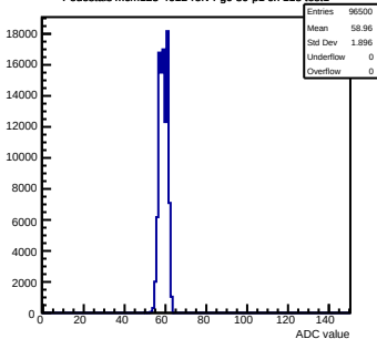
Pedestals mcm123-4612-refv4-g0-s0-p1 ch 118 test1
