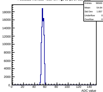
Pedestals mcm123-4612-refv4-g0-s0-p1 ch 119 test1
