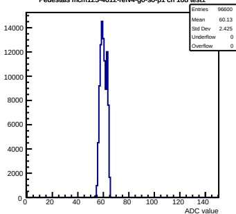
Pedestals mcm123-4612-refv4-g0-s0-p1 ch 108 test1
