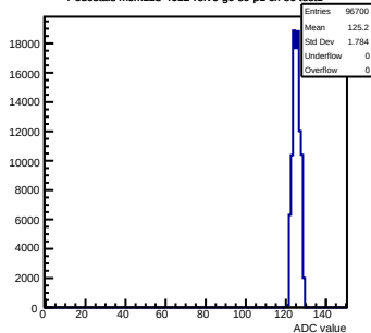
Pedestals mcm123-4612-rlv6-g0-s0-p1 ch 86 test1
