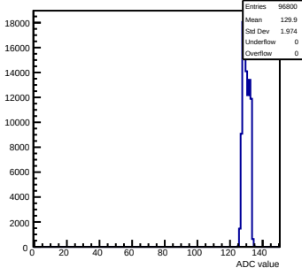
Pedestals mcm123-4612-rlv6-g0-s0-p1 ch 79 test1
