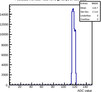
Pedestals mcm123-4612-refv6-g0-s0-p1 ch 106 test1
