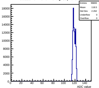
Pedestals mcm123-4612-rlv6-g0-s0-p1 ch 8 test1
