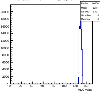
Pedestals mcm123-4612-refv6-g0-s0-p1 ch 126 test1
