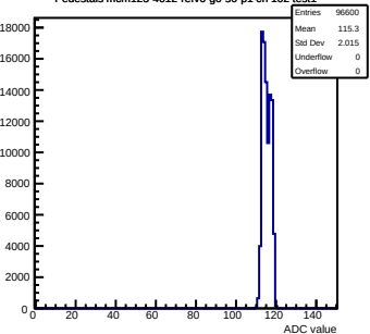
Pedestals mcm123-4612-refv6-g0-s0-p1 ch 102 test1
