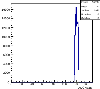
Pedestals mcm123-4612-rlv6-g0-s0-p1 ch 71 test1
