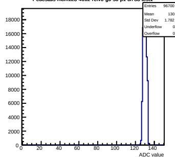
Pedestals mcm123-4612-rlv6-g0-s0-p1 ch 83 test1
