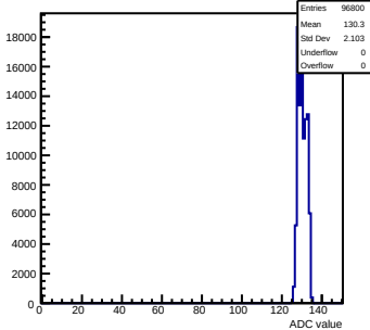
Pedestals mcm123-4612-rlv6-g0-s0-p1 ch 74 test1
