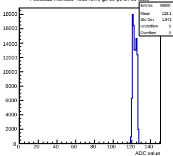
Pedestals mcm123-4612-rlv6-g0-s0-p1 ch 65 test1
