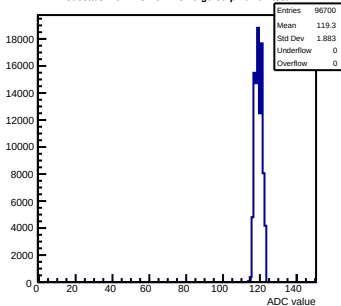
Pedestals mcm123-4612-rlv6-g0-s0-p1 ch 92 test1
