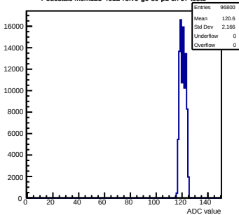
Pedestals mcm123-4612-rlv6-g0-s0-p1 ch 67 test1
