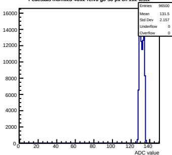
Pedestals mcm123-4612-refv6-g0-s0-p1 ch 112 test1
