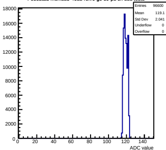
Pedestals mcm123-4612-refv6-g0-s0-p1 ch 111 test1
