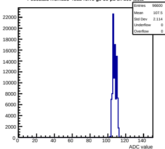
Pedestals mcm123-4612-refv6-g0-s0-p1 ch 109 test1
