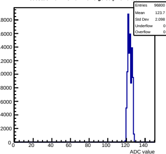
Pedestals mcm123-4612-rlv6-g0-s0-p1 ch 9 test1
