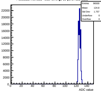
Pedestals mcm123-4612-refv6-g0-s0-p1 ch 123 test1
