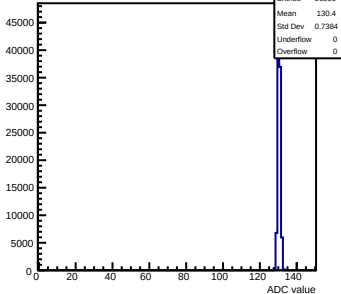
Pedestals mcm123-4612-refv0-g0-s0-p1 ch 120 test1
