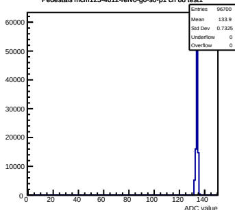
Pedestals mcm123-4612-relv0-g0-s0-p1 ch 88 test1
