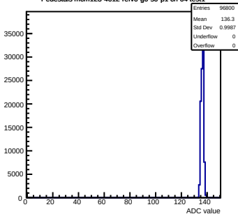
Pedestals mcm123-4612-refv0-g0-s0-p1 ch 64 test1
