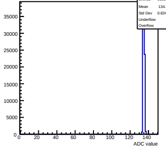
Pedestals mcm123-4612-refv0-g0-s0-p1 ch 122 test1
