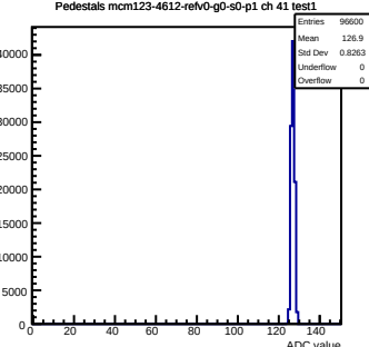
Pedestals mcm123-4612-refv0-g0-s0-p1 ch 41 test1
