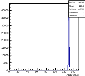
Pedestals mcm123-4612-refv0-g0-s0-p1 ch 24 test1
