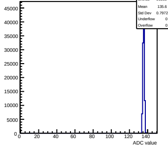
Pedestals mcm123-4612-refv0-g0-s0-p1 ch 127 test1
