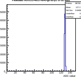
Pedestals mcm123-4612-relv0-g0-s0-p1 ch 82 test1
