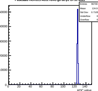
Pedestals mcm123-4612-relv0-g0-s0-p1 ch 91 test1
