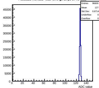
Pedestals mcm123-4612-refv0-g0-s0-p1 ch 78 test1
