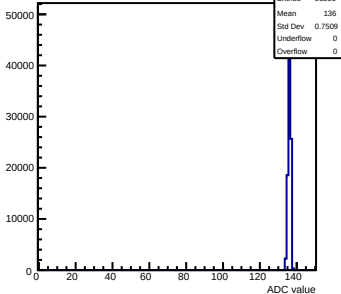
Pedestals mcm123-4612-refv0-g0-s0-p1 ch 124 test1
