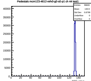
Pedestals mcm123-4612-refv0-g0-s0-p1 ch 44 test1
