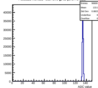
Pedestals mcm123-4612-refv0-g0-s0-p1 ch 75 test1
