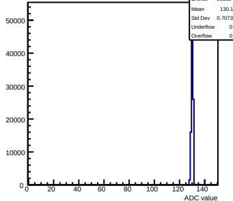
Pedestals mcm123-4612-refv0-g0-s0-p1 ch 119 test1
