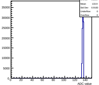
Pedestals mcm123-4612-refv0-g0-s0-p1 ch 116 test1
