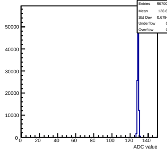
Pedestals mcm123-4612-refv0-g0-s0-p1 ch 30 test1
