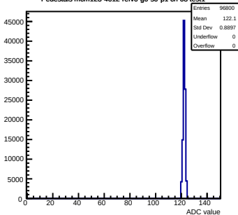
Pedestals mcm123-4612-refv0-g0-s0-p1 ch 68 test1
