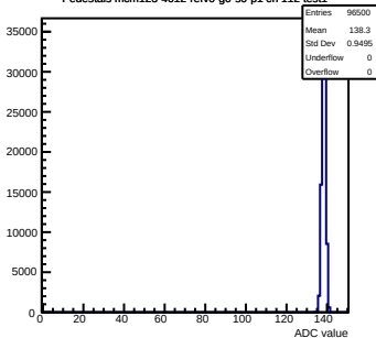
Pedestals mcm123-4612-refv0-g0-s0-p1 ch 112 test1
