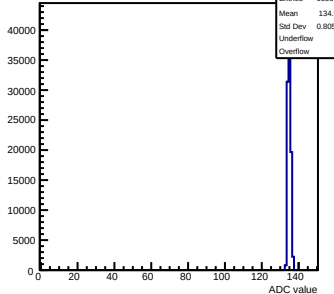
Pedestals mcm123-4612-refv0-g0-s0-p1 ch 126 test1
