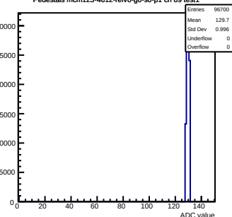
Pedestals mcm123-4612-relv0-g0-s0-p1 ch 89 test1
