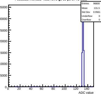
Pedestals mcm123-4612-refv0-g0-s0-p1 ch 73 test1
