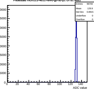
Pedestals mcm123-4612-relv0-g0-s0-p1 ch 81 test1
