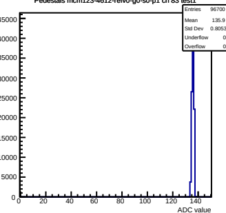
Pedestals mcm123-4612-relv0-g0-s0-p1 ch 83 test1
