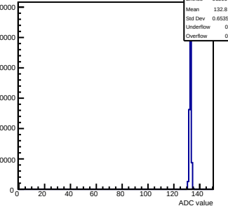
Pedestals mcm123-4612-refv0-g0-s0-p1 ch 125 test1
