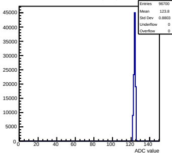
Pedestals mcm123-4612-refv0-g0-s0-p1 ch 20 test1
