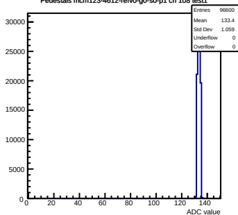
Pedestals mcm123-4612-refv0-g0-s0-p1 ch 108 test1
