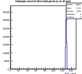
Pedestals mcm123-4612-refv0-g0-s0-p1 ch 40 test1
