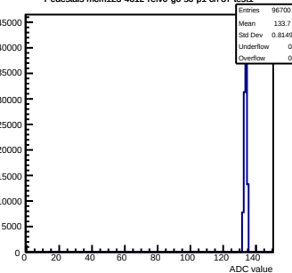
Pedestals mcm123-4612-relv0-g0-s0-p1 ch 87 test1
