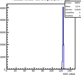
Pedestals mcm123-4612-refv0-g0-s0-p1 ch 77 test1
