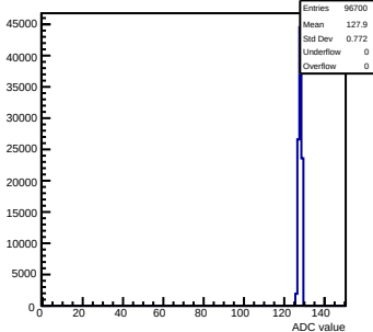
Pedestals mcm123-4612-refv0-g0-s0-p1 ch 28 test1
