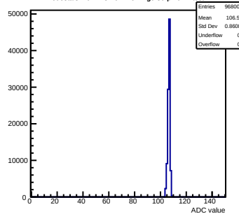
Pedestals mcm123-4612-refv1-g0-s0-p1 ch 2 test1
