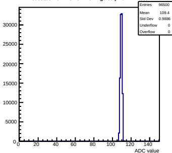
Pedestals mcm123-4612-refv1-g0-s0-p1 ch 112 test1
