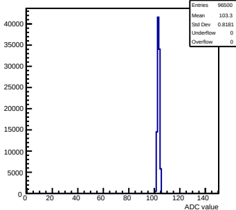
Pedestals mcm123-4612-refv1-g0-s0-p1 ch 125 test1
