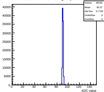
Pedestals mcm123-4612-rfv1-g0-s0-p1 ch 85 test1
