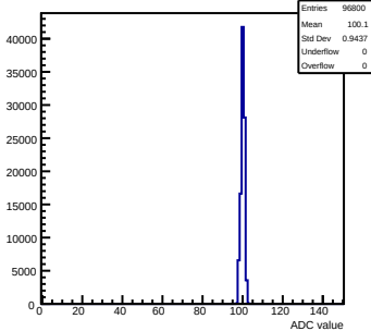
Pedestals mcm123-4612-refv1-g0-s0-p1 ch 12 test1
