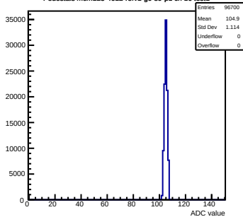
Pedestals mcm123-4612-rfv1-g0-s0-p1 ch 16 test1
