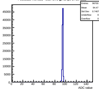
Pedestals mcm123-4612-rfv1-g0-s0-p1 ch 29 test1
