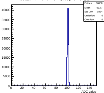
Pedestals mcm123-4612-refv1-g0-s0-p1 ch 100 test1
