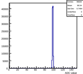
Pedestals mcm123-4612-refv1-g0-s0-p1 ch 117 test1
