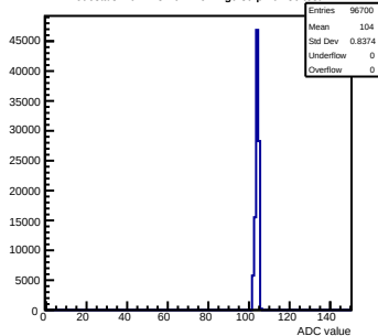
Pedestals mcm123-4612-rfv1-g0-s0-p1 ch 86 test1
