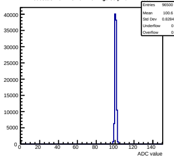
Pedestals mcm123-4612-refv1-g0-s0-p1 ch 114 test1
