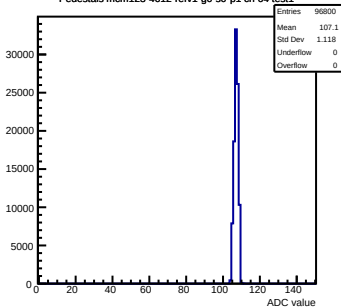
Pedestals mcm123-4612-rfv1-g0-s0-p1 ch 64 test1
