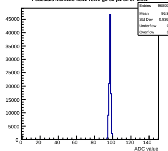
Pedestals mcm123-4612-rfv1-g0-s0-p1 ch 67 test1
