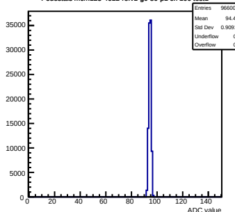
Pedestals mcm123-4612-refv1-g0-s0-p1 ch 106 test1
