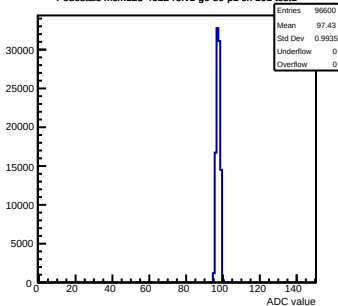
Pedestals mcm123-4612-refv1-g0-s0-p1 ch 101 test1
