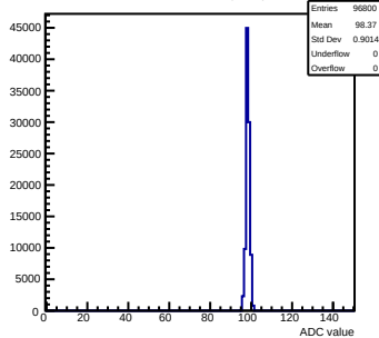
Pedestals mcm123-4612-refv1-g0-s0-p1 ch 5 test1
