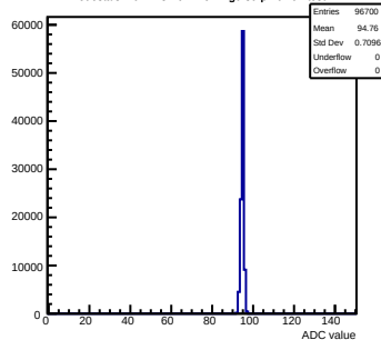
Pedestals mcm123-4612-rfv1-g0-s0-p1 ch 91 test1
