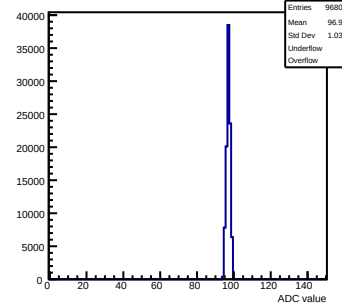
Pedestals mcm123-4612-refv1-g0-s0-p1 ch 11 test1
