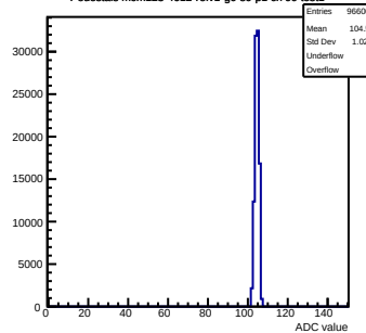
Pedestals mcm123-4612-refv1-g0-s0-p1 ch 99 test1
