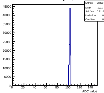
Pedestals mcm123-4612-refv1-g0-s0-p1 ch 1 test1
