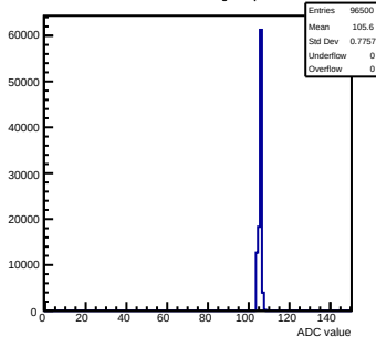
Pedestals mcm123-4612-refv1-g0-s0-p1 ch 122 test1
