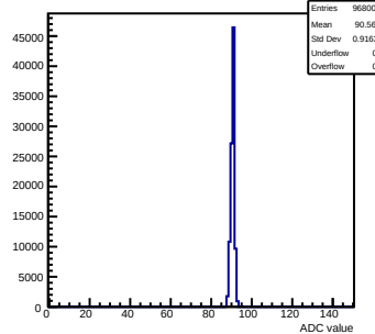
Pedestals mcm123-4612-refv1-g0-s0-p1 ch 10 test1
