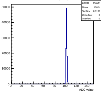
Pedestals mcm123-4612-refv1-g0-s0-p1 ch 120 test1
