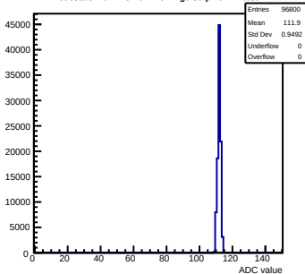
Pedestals mcm123-4612-rfv1-g0-s0-p1 ch 72 test1
