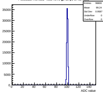
Pedestals mcm123-4612-rfv1-g0-s0-p1 ch 69 test1
