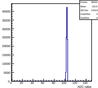
Pedestals mcm123-4612-refv1-g0-s0-p1 ch 118 test1
