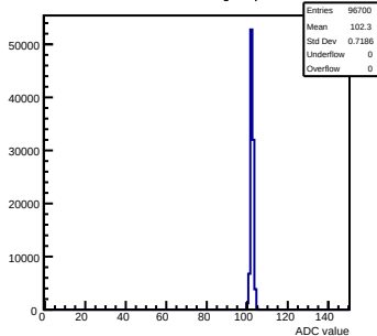
Pedestals mcm123-4612-rfv1-g0-s0-p1 ch 93 test1
