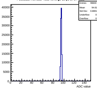
Pedestals mcm123-4612-refv1-g0-s0-p1 ch 97 test1
