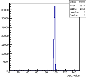
Pedestals mcm123-4612-refv1-g0-s0-p1 ch 8 test1
