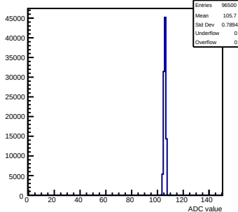
Pedestals mcm123-4612-refv1-g0-s0-p1 ch 126 test1
