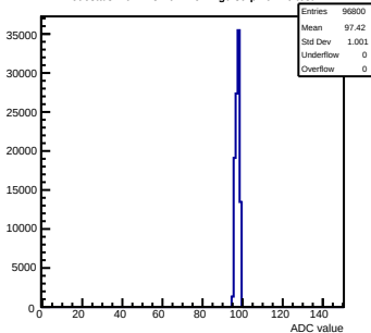
Pedestals mcm123-4612-rfv1-g0-s0-p1 ch 76 test1
