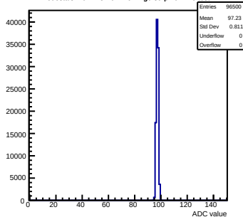
Pedestals mcm123-4612-refv1-g0-s0-p1 ch 115 test1
