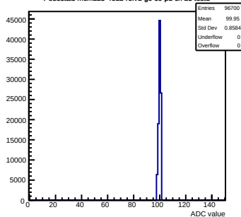
Pedestals mcm123-4612-rfv1-g0-s0-p1 ch 25 test1
