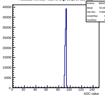
Pedestals mcm123-4612-refv1-g0-s0-p1 ch 102 test1
