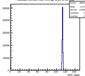
Pedestals mcm123-4612-rfv1-g0-s0-p1 ch 66 test1
