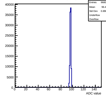
Pedestals mcm123-4612-refv1-g0-s0-p1 ch 7 test1
