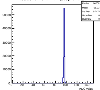
Pedestals mcm123-4612-rfv1-g0-s0-p1 ch 26 test1
