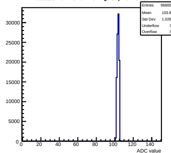
Pedestals mcm123-4612-rfv1-g0-s0-p1 ch 75 test1
