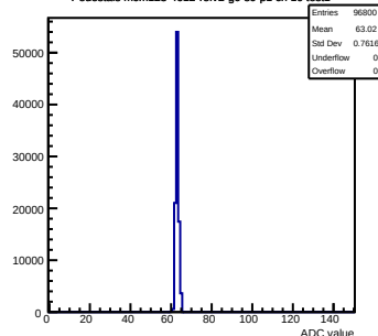
Pedestals mcm123-4612-ref2-g0-s0-p1 ch 10 test1
