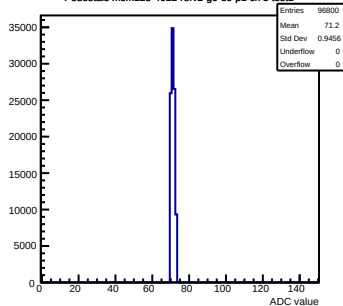
Pedestals mcm123-4612-ref2-g0-s0-p1 ch 5 test1
