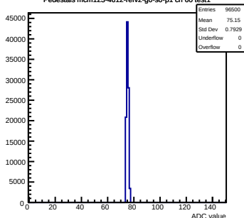
Pedestals mcm123-4612-refv2-g0-s0-p1 ch 60 test1
