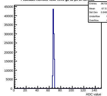
Pedestals mcm123-4612-ref2-g0-s0-p1 ch 18 test1
