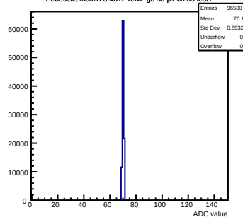
Pedestals mcm123-4612-refv2-g0-s0-p1 ch 55 test1
