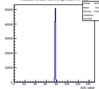
Pedestals mcm123-4612-ref2-g0-s0-p1 ch 27 test1
