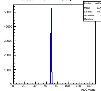
Pedestals mcm123-4612-ref2-g0-s0-p1 ch 26 test1
