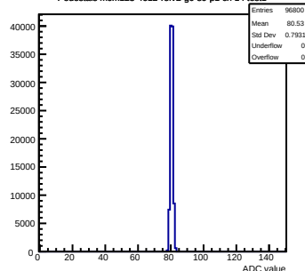
Pedestals mcm123-4612-ref2-g0-s0-p1 ch 14 test1
