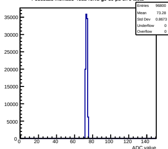
Pedestals mcm123-4612-ref2-g0-s0-p1 ch 9 test1
