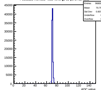
Pedestals mcm123-4612-ref2-g0-s0-p1 ch 15 test1
