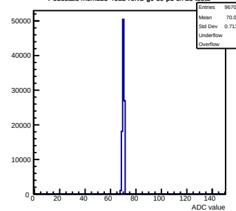
Pedestals mcm123-4612-ref2-g0-s0-p1 ch 23 test1
