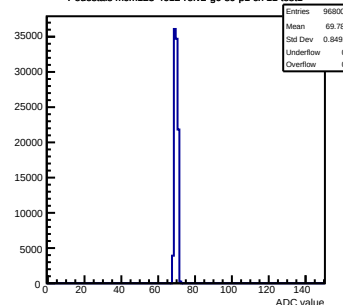
Pedestals mcm123-4612-ref2-g0-s0-p1 ch 11 test1
