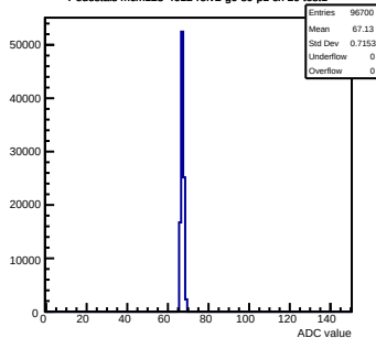
Pedestals mcm123-4612-ref2-g0-s0-p1 ch 29 test1
