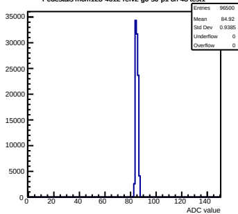
Pedestals mcm123-4612-refv2-g0-s0-p1 ch 48 test1
