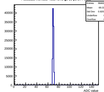
Pedestals mcm123-4612-ref2-g0-s0-p1 ch 7 test1
