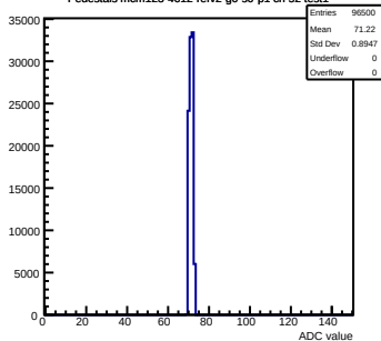
Pedestals mcm123-4612-refv2-g0-s0-p1 ch 52 test1
