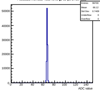
Pedestals mcm123-4612-ref2-g0-s0-p1 ch 20 test1
