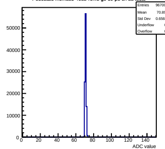
Pedestals mcm123-4612-ref2-g0-s0-p1 ch 22 test1
