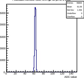
Pedestals mcm123-4612-refv4-g0-s0-p1 ch 5 test1
