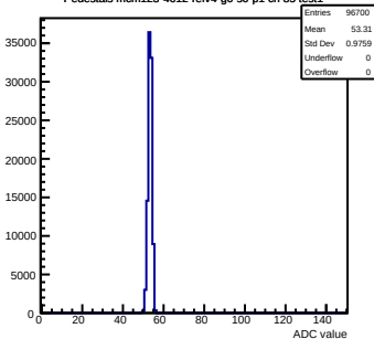
Pedestals mcm123-4612-rlv4-g0-s0-p1 ch 85 test1
