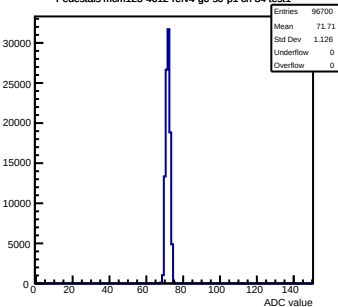
Pedestals mcm123-4612-rlv4-g0-s0-p1 ch 84 test1
