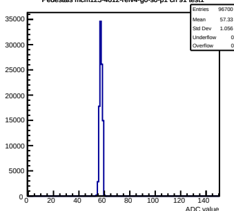
Pedestals mcm123-4612-rlv4-g0-s0-p1 ch 91 test1
