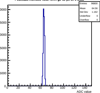
Pedestals mcm123-4612-refv4-g0-s0-p1 ch 1 test1
