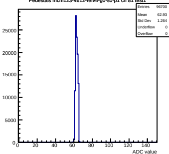
Pedestals mcm123-4612-rlv4-g0-s0-p1 ch 81 test1
