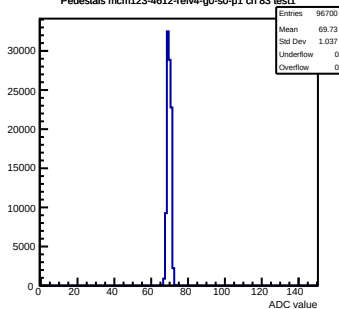
Pedestals mcm123-4612-rlv4-g0-s0-p1 ch 83 test1
