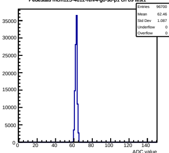
Pedestals mcm123-4612-rlv4-g0-s0-p1 ch 89 test1
