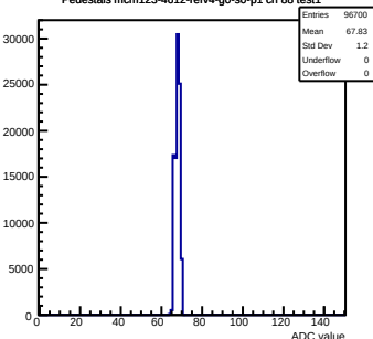
Pedestals mcm123-4612-rlv4-g0-s0-p1 ch 88 test1
