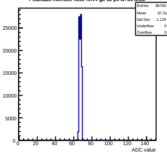
Pedestals mcm123-4612-rlv4-g0-s0-p1 ch 86 test1
