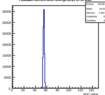
Pedestals mcm123-4612-rlv4-g0-s0-p1 ch 95 test1
