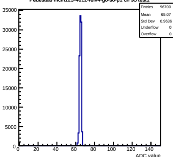
Pedestals mcm123-4612-rlv4-g0-s0-p1 ch 93 test1
