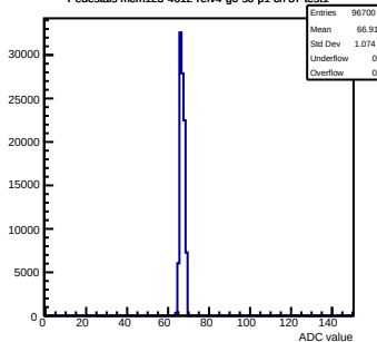
Pedestals mcm123-4612-rlv4-g0-s0-p1 ch 87 test1
