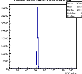
Pedestals mcm123-4612-rlv4-g0-s0-p1 ch 90 test1
