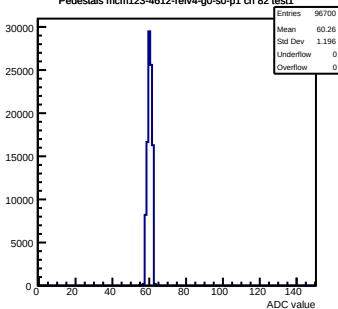
Pedestals mcm123-4612-rlv4-g0-s0-p1 ch 82 test1
