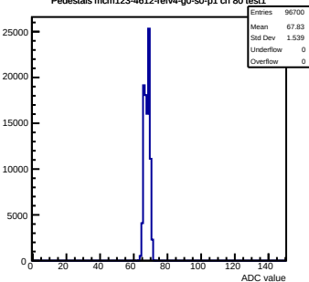
Pedestals mcm123-4612-rlv4-g0-s0-p1 ch 80 test1
