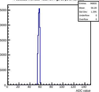
Pedestals mcm123-4612-refv4-g0-s0-p1 ch 13 test1
