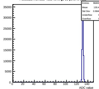
Pedestals mcm123-4612-rtv6-g0-s0-p1 ch 6 test1
