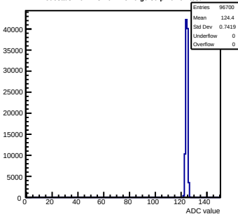
Pedestals mcm123-4612-relv6-g0-s0-p1 ch 91 test1
