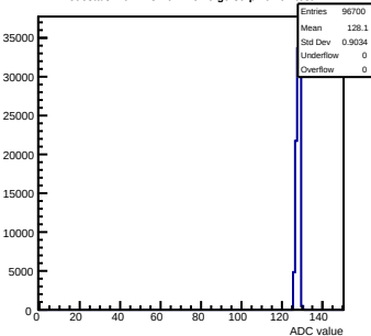
Pedestals mcm123-4612-relv6-g0-s0-p1 ch 92 test1
