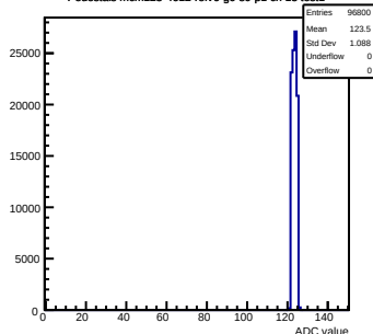
Pedestals mcm123-4612-rtv6-g0-s0-p1 ch 13 test1
