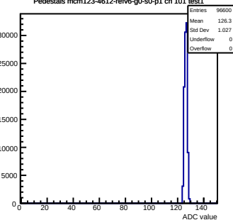
Pedestals mcm123-4612-refv6-g0-s0-p1 ch 101 test1
