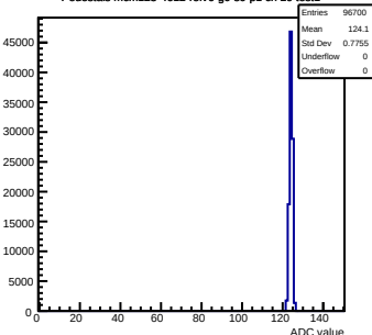
Pedestals mcm123-4612-relv6-g0-s0-p1 ch 29 test1
