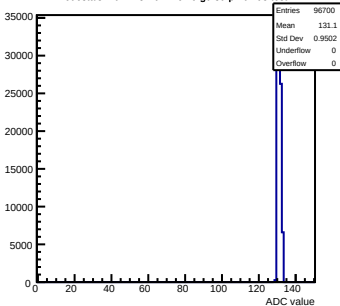
Pedestals mcm123-4612-relv6-g0-s0-p1 ch 93 test1
