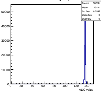
Pedestals mcm123-4612-relv6-g0-s0-p1 ch 94 test1
