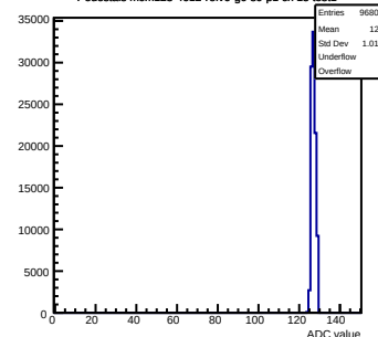
Pedestals mcm123-4612-rtv6-g0-s0-p1 ch 15 test1
