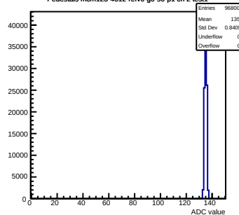
Pedestals mcm123-4612-rtv6-g0-s0-p1 ch 2 test1
