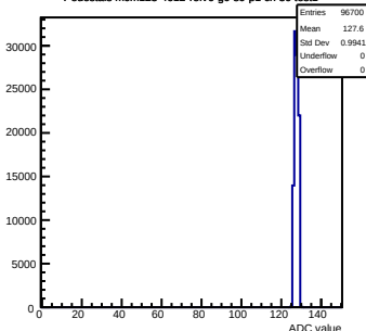
Pedestals mcm123-4612-relv6-g0-s0-p1 ch 30 test1
