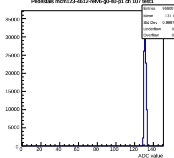
Pedestals mcm123-4612-refv6-g0-s0-p1 ch 107 test1
