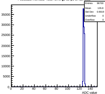
Pedestals mcm123-4612-relv6-g0-s0-p1 ch 82 test1
