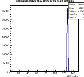
Pedestals mcm123-4612-refv6-g0-s0-p1 ch 110 test1
