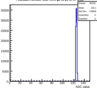
Pedestals mcm123-4612-relv6-g0-s0-p1 ch 17 test1
