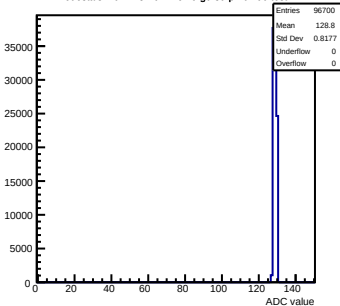
Pedestals mcm123-4612-relv6-g0-s0-p1 ch 90 test1
