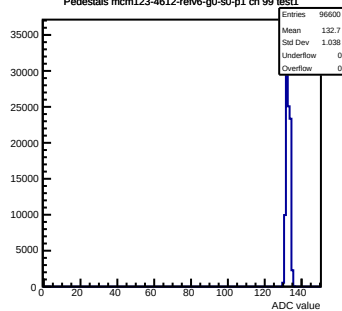
Pedestals mcm123-4612-refv6-g0-s0-p1 ch 99 test1
