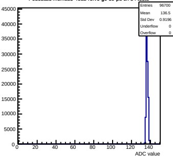
Pedestals mcm123-4612-relv6-g0-s0-p1 ch 84 test1
