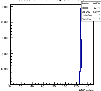
Pedestals mcm123-4612-relv6-g0-s0-p1 ch 28 test1
