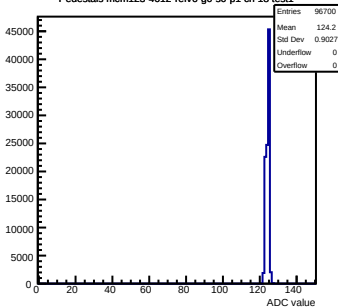
Pedestals mcm123-4612-relv6-g0-s0-p1 ch 18 test1
