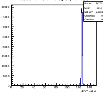
Pedestals mcm123-4612-relv6-g0-s0-p1 ch 26 test1
