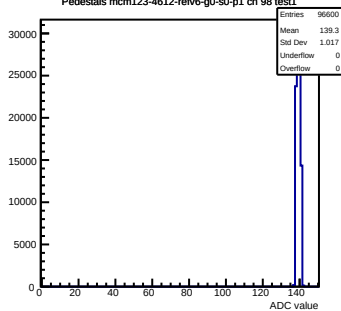
Pedestals mcm123-4612-refv6-g0-s0-p1 ch 98 test1
