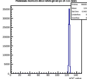
Pedestals mcm123-4612-refv6-g0-s0-p1 ch 111 test1
