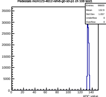
Pedestals mcm123-4612-refv6-g0-s0-p1 ch 108 test1
