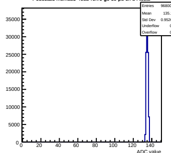
Pedestals mcm123-4612-rtv6-g0-s0-p1 ch 14 test1
