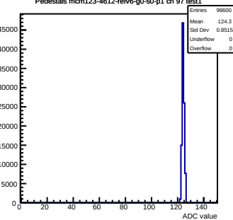
Pedestals mcm123-4612-refv6-g0-s0-p1 ch 97 test1
