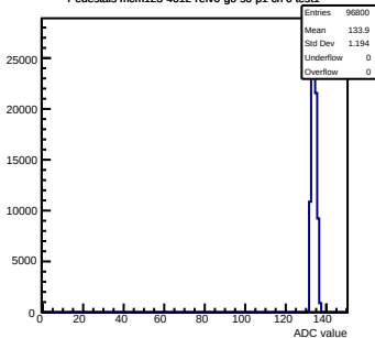
Pedestals mcm123-4612-rtv6-g0-s0-p1 ch 0 test1
