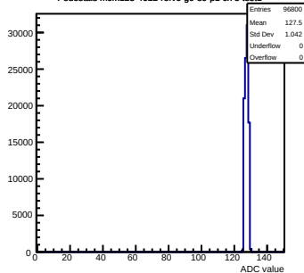
Pedestals mcm123-4612-rtv6-g0-s0-p1 ch 5 test1
