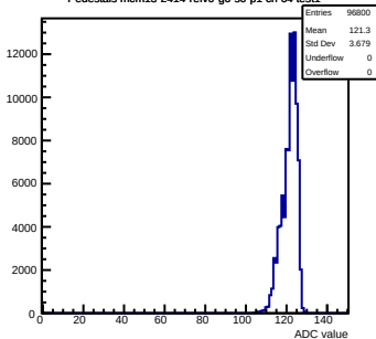
Pedestals mcm13-2414-refV0-g0-s0-p1 ch 64 test1
