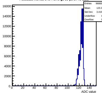
Pedestals mcm13-2414-refV0-g0-s0-p1 ch 75 test1
