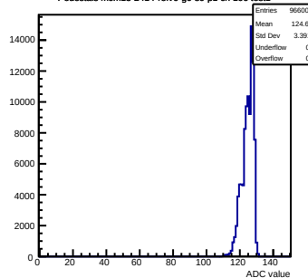
Pedestals mcm13-2414-refV0-g0-s0-p1 ch 106 test1
