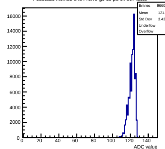
Pedestals mcm13-2414-refV0-g0-s0-p1 ch 107 test1
