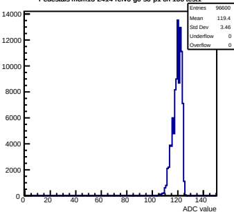
Pedestals mcm13-2414-refV0-g0-s0-p1 ch 100 test1
