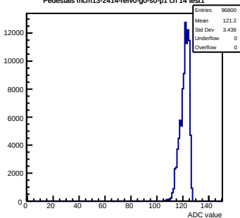
Pedestals mcm13-2414-refv0-g0-s0-p1 ch 14 test1
