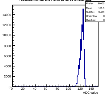
Pedestals mcm13-2414-refV0-g0-s0-p1 ch 101 test1
