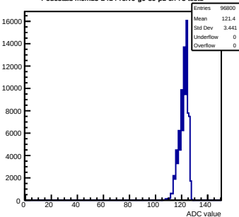
Pedestals mcm13-2414-refV0-g0-s0-p1 ch 73 test1
