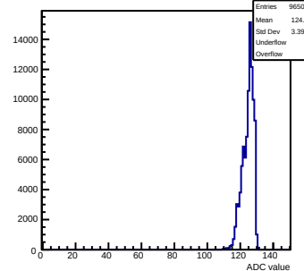
Pedestals mcm13-2414-rv0-g0-s0-p1 ch 63 test1
