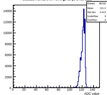
Pedestals mcm13-2414- \text{rev0} -g0-s0-p1 ch 26 test1
