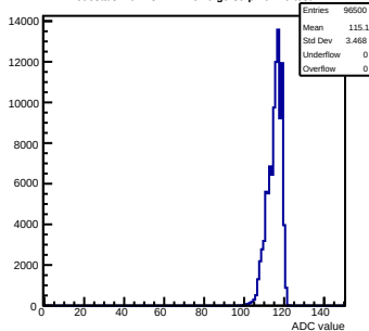
Pedestals mcm13-2414-rv0-g0-s0-p1 ch 49 test1
