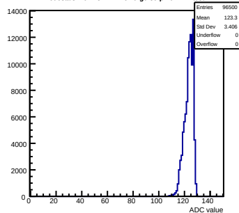
Pedestals mcm13-2414-refV0-g0-s0-p1 ch 127 test1
