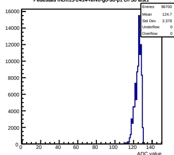
Pedestals mcm13-2414- \text{rev0} -g0-s0-p1 ch 30 test1
