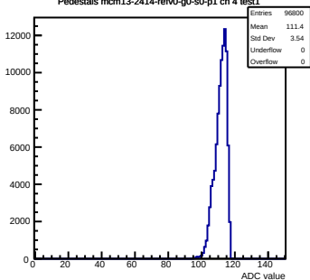
Pedestals mcm13-2414-refv0-g0-s0-p1 ch 4 test1
