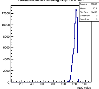
Pedestals mcm13-2414-refv0-g0-s0-p1 ch 12 test1
