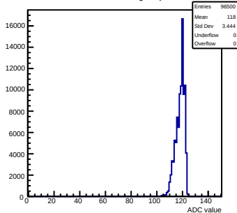
Pedestals mcm13-2414-rv0-g0-s0-p1 ch 57 test1
