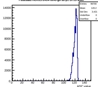
Pedestals mcm13-2414- \text{rev0} -g0-s0-p1 ch 29 test1
