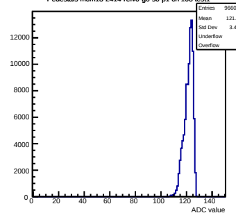
Pedestals mcm13-2414-refV0-g0-s0-p1 ch 103 test1
