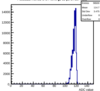
Pedestals mcm13-2414-refV0-g0-s0-p1 ch 117 test1
