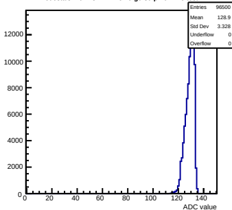
Pedestals mcm13-2414-refV0-g0-s0-p1 ch 125 test1
