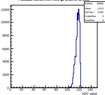
Pedestals mcm13-2414-refV0-g0-s0-p1 ch 96 test1
