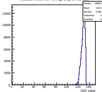
Pedestals mcm13-2414-refV0-g0-s0-p1 ch 109 test1
