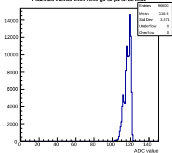
Pedestals mcm13-2414- \text{rev0} -g0-s0-p1 ch 33 test1
