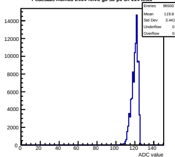
Pedestals mcm13-2414-refV0-g0-s0-p1 ch 114 test1
