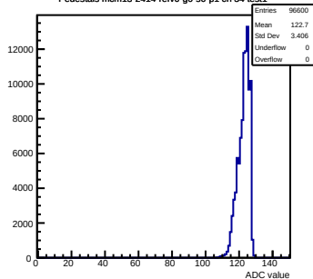
Pedestals mcm13-2414- \text{rev0} -g0-s0-p1 ch 34 test1
