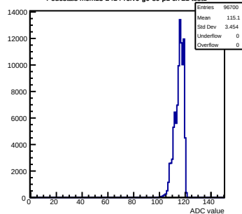
Pedestals mcm13-2414- \text{rev0} -g0-s0-p1 ch 21 test1
