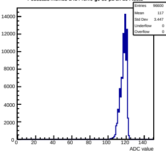
Pedestals mcm13-2414-refV0-g0-s0-p1 ch 104 test1
