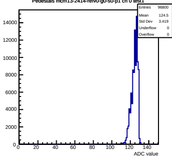
Pedestals mcm13-2414-refv0-g0-s0-p1 ch 0 test1
