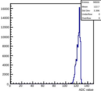
Pedestals mcm13-2414-rv0-g0-s0-p1 ch 60 test1
