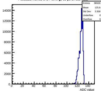
Pedestals mcm13-2414-refV0-g0-s0-p1 ch 118 test1
