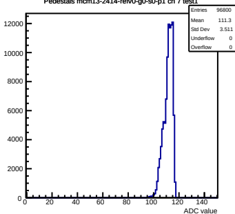
Pedestals mcm13-2414-refv0-g0-s0-p1 ch 7 test1
