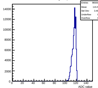
Pedestals mcm13-2414-rv0-g0-s0-p1 ch 58 test1
