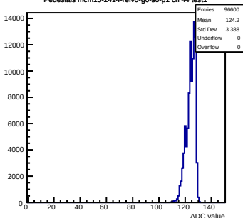
Pedestals mcm13-2414- \text{rev0} -g0-s0-p1 ch 44 test1
