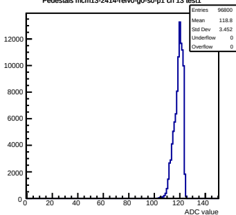
Pedestals mcm13-2414-refv0-g0-s0-p1 ch 13 test1
