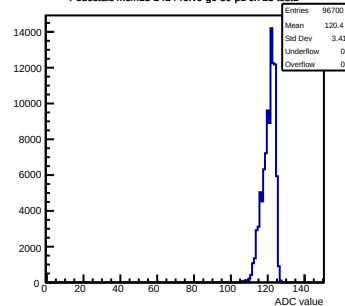
Pedestals mcm13-2414- \text{rev0} -g0-s0-p1 ch 23 test1
