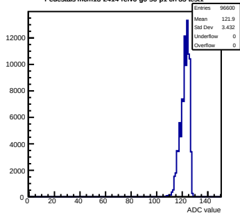
Pedestals mcm13-2414- \text{rev0} -g0-s0-p1 ch 35 test1
