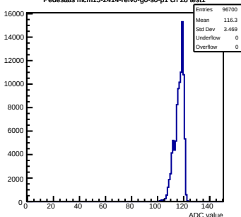
Pedestals mcm13-2414- \text{rev0} -g0-s0-p1 ch 28 test1
