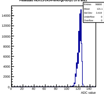
Pedestals mcm13-2414-refv0-g0-s0-p1 ch 8 test1
