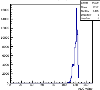
Pedestals mcm13-2414-rv0-g0-s0-p1 ch 56 test1
