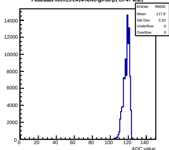
Pedestals mcm13-2414- \text{rev0} -g0-s0-p1 ch 47 test1
