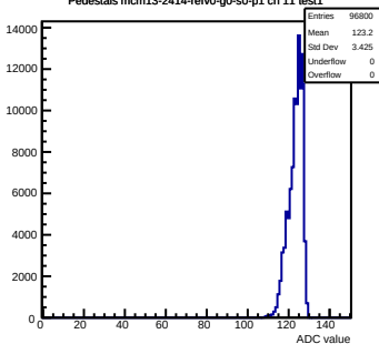
Pedestals mcm13-2414-refv0-g0-s0-p1 ch 11 test1
