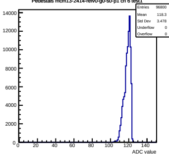
Pedestals mcm13-2414-refv0-g0-s0-p1 ch 6 test1
