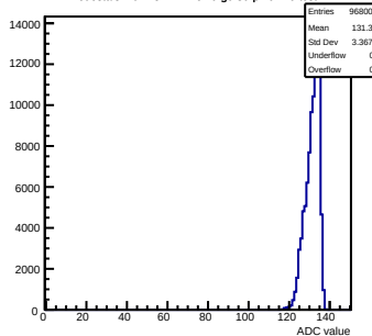
Pedestals mcm13-2414-refV0-g0-s0-p1 ch 79 test1
