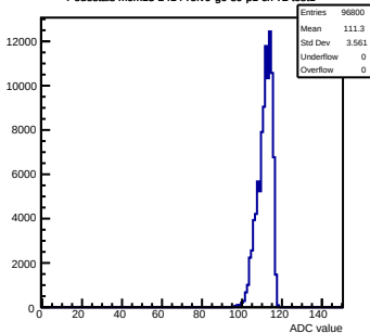
Pedestals mcm13-2414-refV0-g0-s0-p1 ch 72 test1
