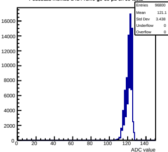
Pedestals mcm13-2414-refV0-g0-s0-p1 ch 69 test1
