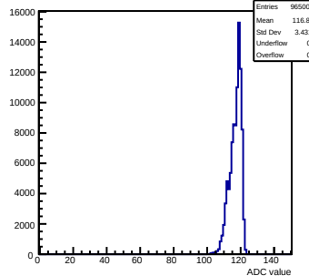
Pedestals mcm13-2414-rv0-g0-s0-p1 ch 62 test1
