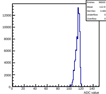
Pedestals mcm13-2414-rv0-g0-s0-p1 ch 61 test1
