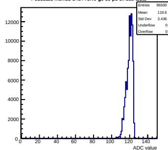
Pedestals mcm13-2414-refV0-g0-s0-p1 ch 119 test1
