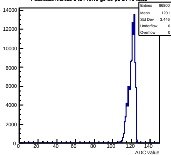
Pedestals mcm13-2414-refV0-g0-s0-p1 ch 70 test1
