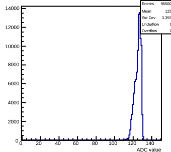
Pedestals mcm13-2414-rv0-g0-s0-p1 ch 54 test1
