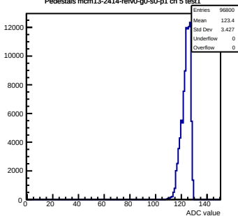
Pedestals mcm13-2414-refv0-g0-s0-p1 ch 5 test1
