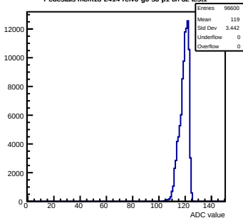
Pedestals mcm13-2414- \text{rev0} -g0-s0-p1 ch 32 test1
