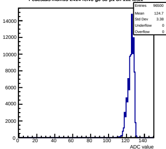
Pedestals mcm13-2414-refV0-g0-s0-p1 ch 112 test1
