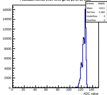
Pedestals mcm13-2414- \text{rev0} -g0-s0-p1 ch 39 test1
