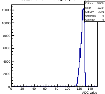
Pedestals mcm13-2414-refV0-g0-s0-p1 ch 116 test1
