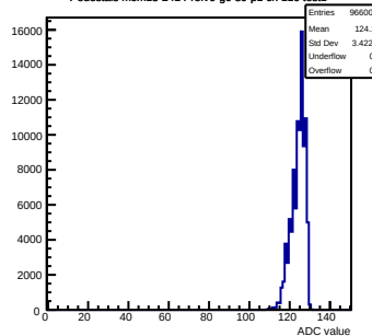
Pedestals mcm13-2414-refV0-g0-s0-p1 ch 110 test1
