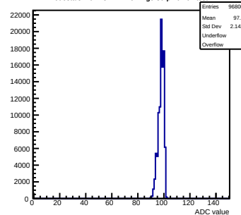
Pedestals mcm13-2414-refv1-g0-s0-p1 ch 67 test1
