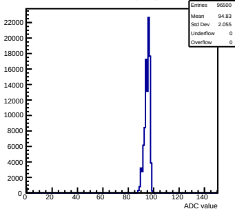
Pedestals mcm13-2414-refv1-g0-s0-p1 ch 112 test1
