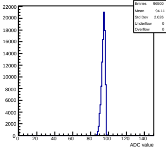
Pedestals mcm13-2414-refv1-g0-s0-p1 ch 120 test1
