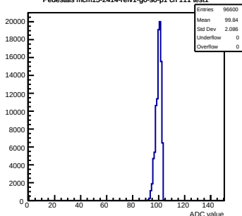
Pedestals mcm13-2414-refv1-g0-s0-p1 ch 111 test1
