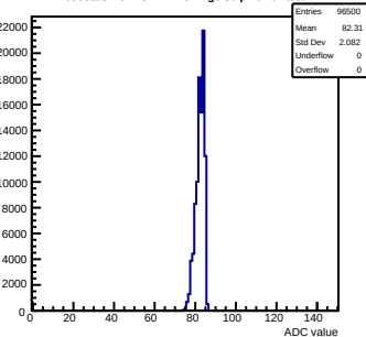
Pedestals mcm13-2414-refv1-g0-s0-p1 ch 61 test1
