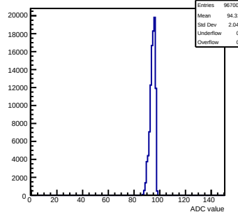
Pedestals mcm13-2414-refv1-g0-s0-p1 ch 94 test1
