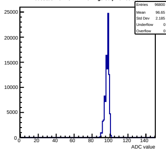
Pedestals mcm13-2414-refv1-g0-s0-p1 ch 65 test1
