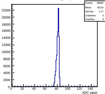
Pedestals mcm13-2414-refv1-g0-s0-p1 ch 72 test1
