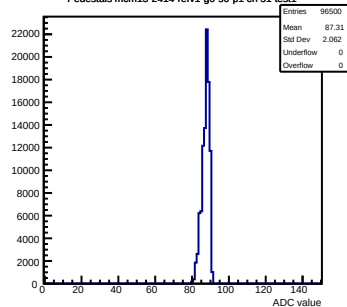
Pedestals mcm13-2414-refv1-g0-s0-p1 ch 51 test1
