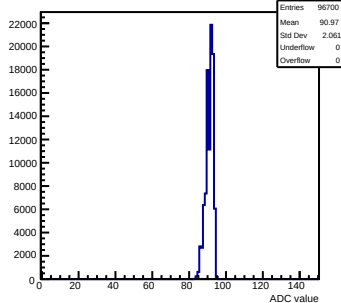
Pedestals mcm13-2414-refv1-g0-s0-p1 ch 93 test1
