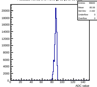
Pedestals mcm13-2414-refv1-g0-s0-p1 ch 96 test1
