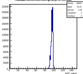
Pedestals mcm13-2414-refv1-g0-s0-p1 ch 110 test1
