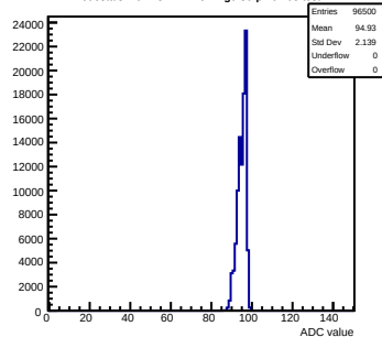
Pedestals mcm13-2414-refv1-g0-s0-p1 ch 63 test1
