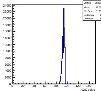
Pedestals mcm13-2414-refv1-g0-s0-p1 ch 74 test1
