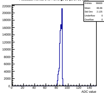
Pedestals mcm13-2414-refv1-g0-s0-p1 ch 99 test1
