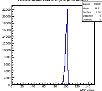
Pedestals mcm13-2414-refv1-g0-s0-p1 ch 109 test1
