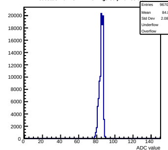
Pedestals mcm13-2414-refv1-g0-s0-p1 ch 83 test1
