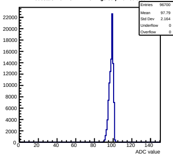
Pedestals mcm13-2414-refv1-g0-s0-p1 ch 80 test1
