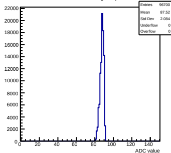
Pedestals mcm13-2414-refv1-g0-s0-p1 ch 89 test1
