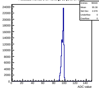
Pedestals mcm13-2414-refv1-g0-s0-p1 ch 54 test1
