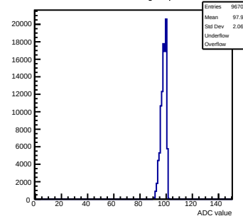
Pedestals mcm13-2414-refv1-g0-s0-p1 ch 91 test1
