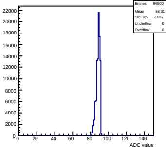
Pedestals mcm13-2414-refv1-g0-s0-p1 ch 113 test1
