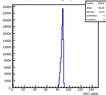
Pedestals mcm13-2414-refv1-g0-s0-p1 ch 62 test1
