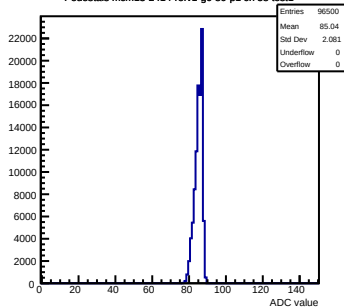
Pedestals mcm13-2414-refv1-g0-s0-p1 ch 58 test1
