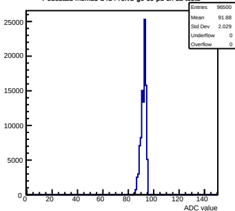
Pedestals mcm13-2414-refv1-g0-s0-p1 ch 52 test1
