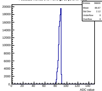
Pedestals mcm13-2414-refv1-g0-s0-p1 ch 97 test1
