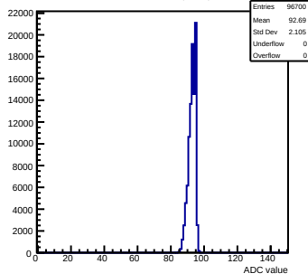
Pedestals mcm13-2414-refv1-g0-s0-p1 ch 85 test1
