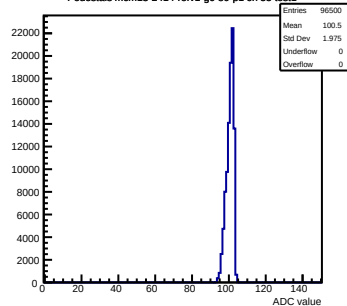
Pedestals mcm13-2414-refv1-g0-s0-p1 ch 55 test1
