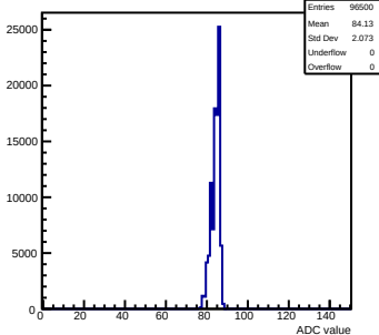
Pedestals mcm13-2414-refv1-g0-s0-p1 ch 117 test1
