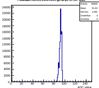
Pedestals mcm13-2414-refv1-g0-s0-p1 ch 107 test1
