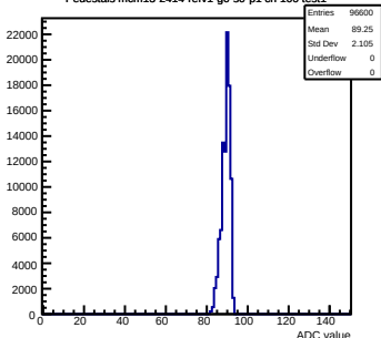
Pedestals mcm13-2414-refv1-g0-s0-p1 ch 100 test1
