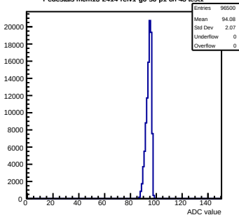
Pedestals mcm13-2414-refv1-g0-s0-p1 ch 48 test1
