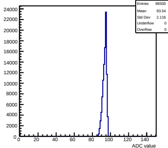
Pedestals mcm13-2414-refv1-g0-s0-p1 ch 127 test1
