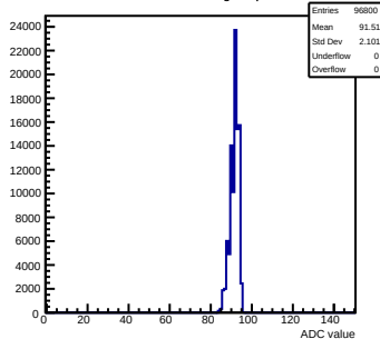
Pedestals mcm13-2414-refv1-g0-s0-p1 ch 73 test1
