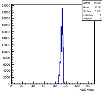
Pedestals mcm13-2414-refv1-g0-s0-p1 ch 88 test1
