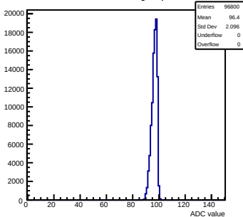
Pedestals mcm13-2414-refv1-g0-s0-p1 ch 76 test1
