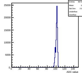
Pedestals mcm13-2414-refv1-g0-s0-p1 ch 87 test1
