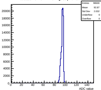
Pedestals mcm13-2414-refv1-g0-s0-p1 ch 60 test1
