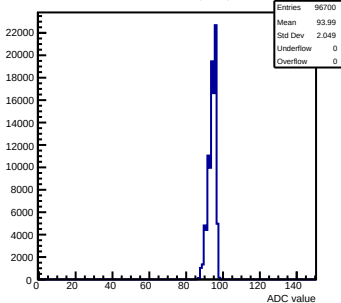
Pedestals mcm13-2414-refv1-g0-s0-p1 ch 84 test1
