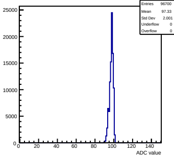
Pedestals mcm13-2414-refv1-g0-s0-p1 ch 92 test1
