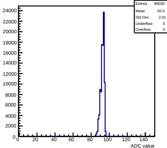
Pedestals mcm13-2414-refv1-g0-s0-p1 ch 121 test1
