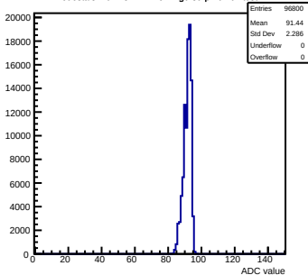
Pedestals mcm13-2414-refv1-g0-s0-p1 ch 64 test1
