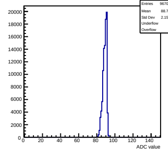
Pedestals mcm13-2414-refv1-g0-s0-p1 ch 95 test1
