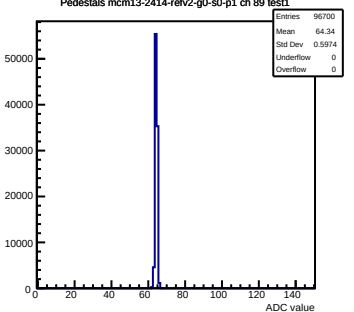
Pedestals mcm13-2414-refv2-g0-s0-p1 ch 89 test1
