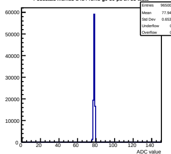
Pedestals mcm13-2414- rev2 -g0-s0-p1 ch 55 test1
