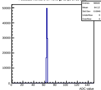
Pedestals mcm13-2414- rev2 -g0-s0-p1 ch 53 test1
