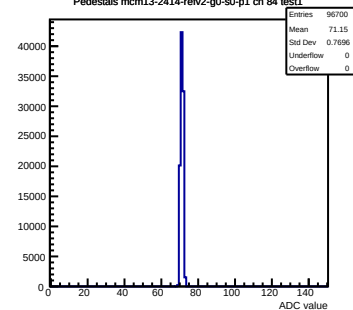
Pedestals mcm13-2414-refv2-g0-s0-p1 ch 84 test1
