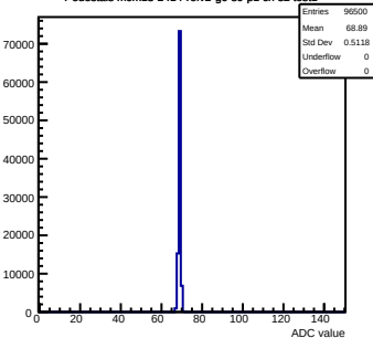
Pedestals mcm13-2414- rev2 -g0-s0-p1 ch 52 test1
