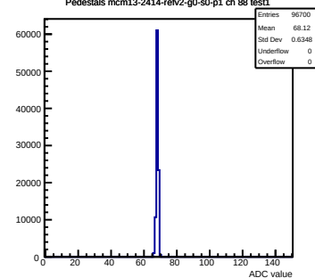
Pedestals mcm13-2414-refv2-g0-s0-p1 ch 88 test1
