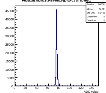
Pedestals mcm13-2414-refv2-g0-s0-p1 ch 80 test1
