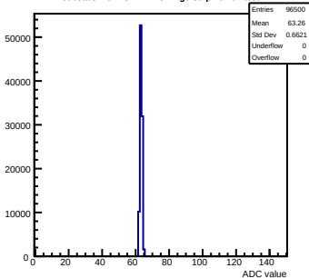
Pedestals mcm13-2414- rev2 -g0-s0-p1 ch 62 test1
