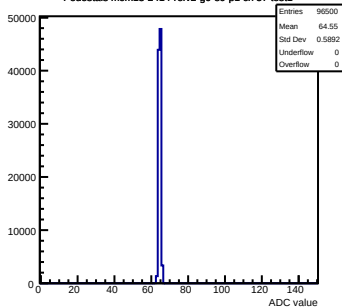
Pedestals mcm13-2414- rev2 -g0-s0-p1 ch 57 test1
