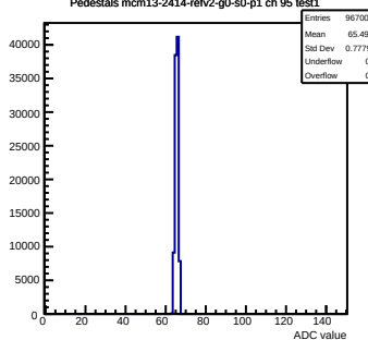
Pedestals mcm13-2414-refv2-g0-s0-p1 ch 95 test1
