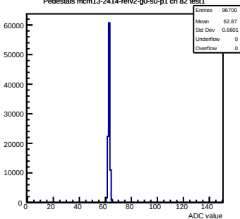
Pedestals mcm13-2414-refv2-g0-s0-p1 ch 82 test1
