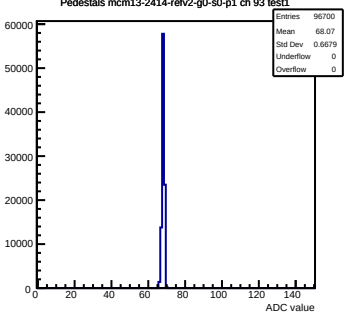
Pedestals mcm13-2414-refv2-g0-s0-p1 ch 93 test1
