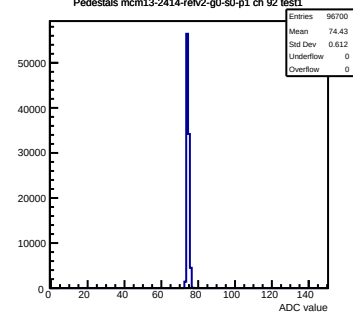
Pedestals mcm13-2414-refv2-g0-s0-p1 ch 92 test1
