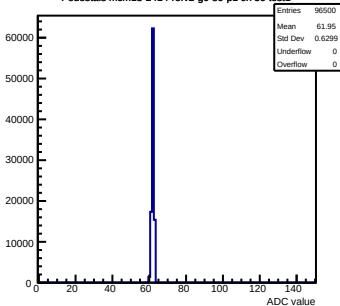
Pedestals mcm13-2414- rev2 -g0-s0-p1 ch 50 test1
