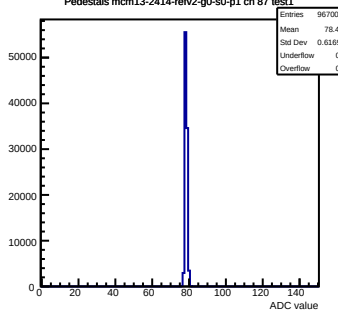
Pedestals mcm13-2414-refv2-g0-s0-p1 ch 87 test1
