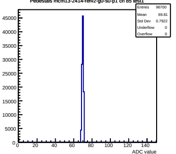
Pedestals mcm13-2414-refv2-g0-s0-p1 ch 85 test1
