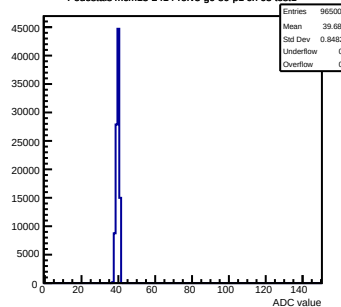
Pedestals mcm13-2414- rev3 -g0-s0-p1 ch 63 test1
