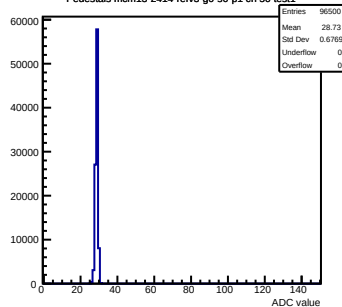
Pedestals mcm13-2414- rev3 -g0-s0-p1 ch 50 test1
