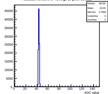
Pedestals mcm13-2414-rfv3-g0-s0-p1 ch 91 test1
