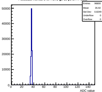
Pedestals mcm13-2414-refv3-g0-s0-p1 ch 77 test1
