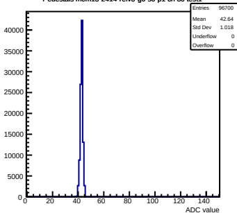
Pedestals mcm13-2414-rfv3-g0-s0-p1 ch 80 test1
