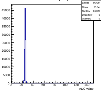
Pedestals mcm13-2414-rfv3-g0-s0-p1 ch 20 test1
