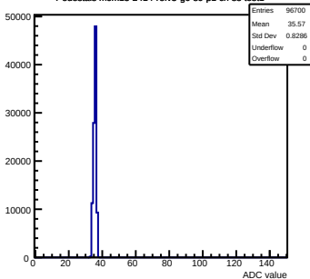
Pedestals mcm13-2414-rfv3-g0-s0-p1 ch 88 test1
