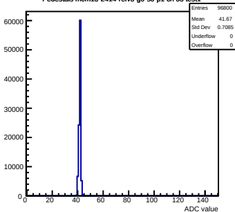
Pedestals mcm13-2414-refv3-g0-s0-p1 ch 65 test1
