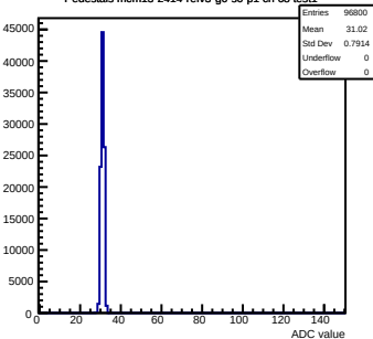
Pedestals mcm13-2414-refv3-g0-s0-p1 ch 68 test1
