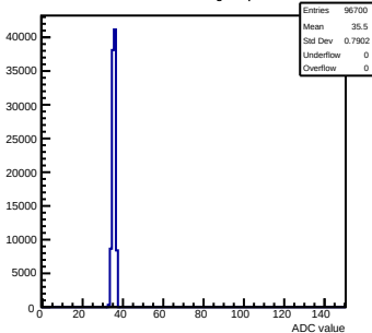
Pedestals mcm13-2414-rfv3-g0-s0-p1 ch 26 test1
