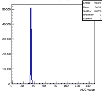
Pedestals mcm13-2414-rfv3-g0-s0-p1 ch 29 test1
