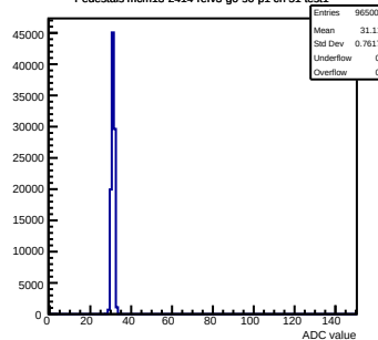
Pedestals mcm13-2414- rev3 -g0-s0-p1 ch 51 test1
