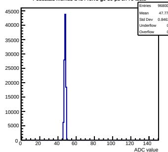
Pedestals mcm13-2414-refv3-g0-s0-p1 ch 79 test1
