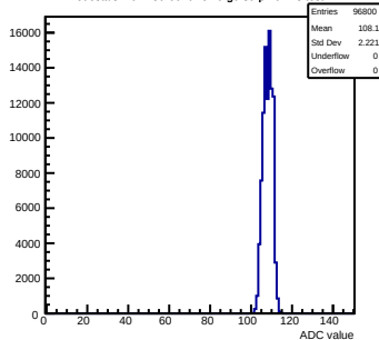
Pedestals mcm130-6610- \text{rev0} -g0-s0-p1 ch 78 test1
