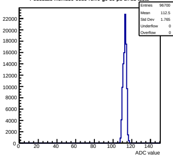
Pedestals mcm130-6610- \text{rev0} -g0-s0-p1 ch 23 \text{test1}
