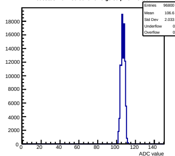
Pedestals mcm130-6610- \text{rev0} -g0-s0-p1 ch 75 test1
