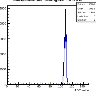
Pedestals mcm130-6610-rev0-g0-s0-p1 ch 89 test1
