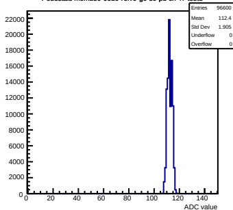
Pedestals mcm130-6610- \text{rev0} -g0-s0-p1 ch 47 test1
