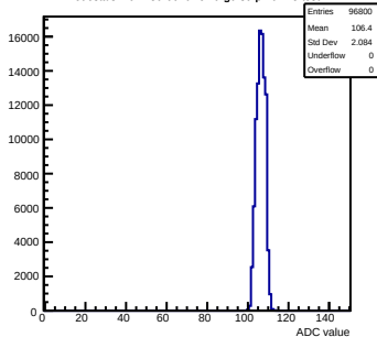
Pedestals mcm130-6610-refV0-g0-s0-p1 ch 15 test1
