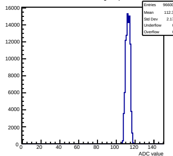
Pedestals mcm130-6610-refV0-g0-s0-p1 ch 111 test1
