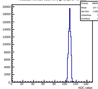
Pedestals mcm130-6610- \text{rev0} -g0-s0-p1 ch 41 test1
