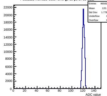
Pedestals mcm130-6610-refv0-g0-s0-p1 ch 63 test1
