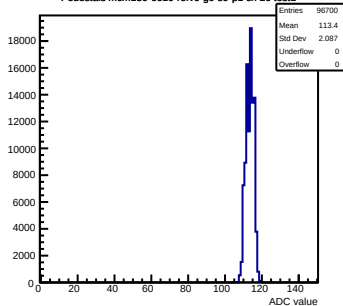
Pedestals mcm130-6610- \text{rev0} -g0-s0-p1 ch 20 \text{test1}
