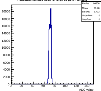
Pedestals mcm130-6610-refv2-g0-s0-p1 ch 48 test1
