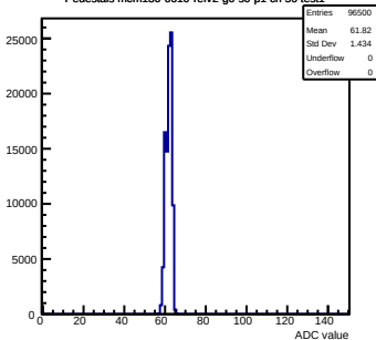
Pedestals mcm130-6610-refv2-g0-s0-p1 ch 50 test1
