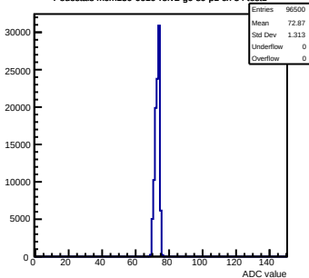
Pedestals mcm130-6610-refv2-g0-s0-p1 ch 54 test1
