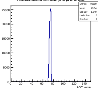
Pedestals mcm130-6610-refv2-g0-s0-p1 ch 60 test1
