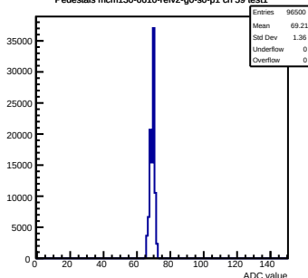
Pedestals mcm130-6610-refv2-g0-s0-p1 ch 59 test1
