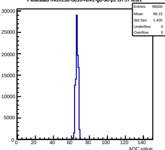
Pedestals mcm130-6610-refv2-g0-s0-p1 ch 57 test1
