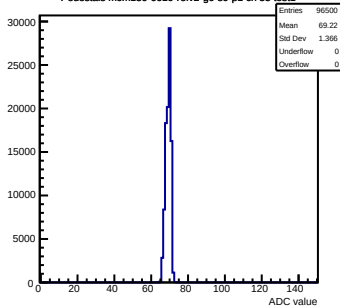
Pedestals mcm130-6610-refv2-g0-s0-p1 ch 55 test1
