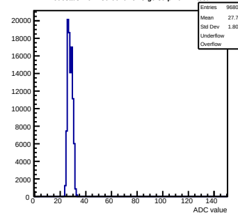
Pedestals mcm130-6610-refv3-g0-s0-p1 ch 11 test1
