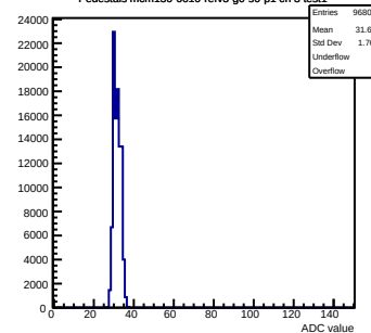
Pedestals mcm130-6610-refv3-g0-s0-p1 ch 3 test1
