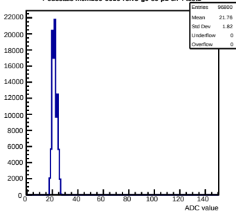
Pedestals mcm130-6610-refv3-g0-s0-p1 ch 4 test1
