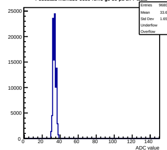
Pedestals mcm130-6610-refv3-g0-s0-p1 ch 7 test1
