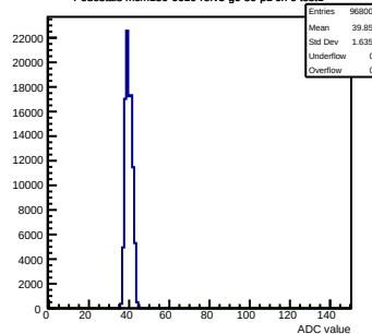
Pedestals mcm130-6610-refv3-g0-s0-p1 ch 6 test1
