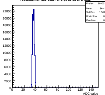
Pedestals mcm130-6610-refv3-g0-s0-p1 ch 1 test1
