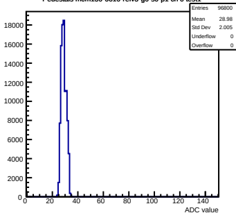
Pedestals mcm130-6610-refv3-g0-s0-p1 ch 0 test1
