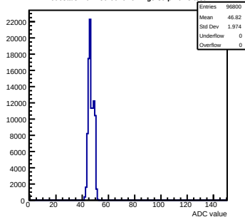
Pedestals mcm130-6610-refv4-g0-s0-p1 ch 5 test1
