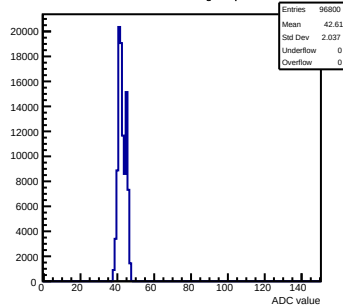
Pedestals mcm130-6610-refv4-g0-s0-p1 ch 11 test1
