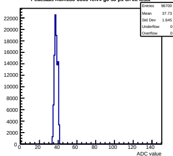
Pedestals mcm130-6610-refv4-g0-s0-p1 ch 22 test1
