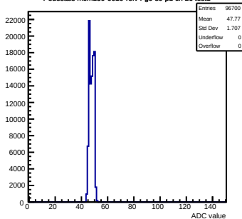
Pedestals mcm130-6610-refv4-g0-s0-p1 ch 26 test1
