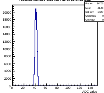
Pedestals mcm130-6610-refv4-g0-s0-p1 ch 21 test1
