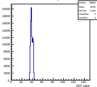
Pedestals mcm130-6610-refv4-g0-s0-p1 ch 14 test1
