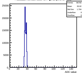
Pedestals mcm130-6610-refv4-g0-s0-p1 ch 27 test1
