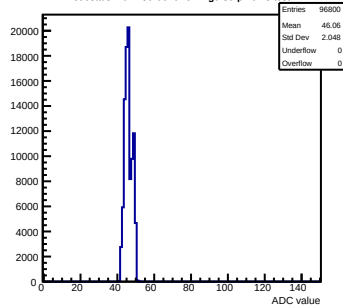
Pedestals mcm130-6610-refv4-g0-s0-p1 ch 3 test1
