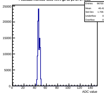
Pedestals mcm130-6610-refv4-g0-s0-p1 ch 17 test1
