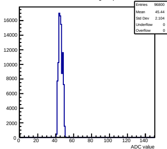
Pedestals mcm130-6610-refv4-g0-s0-p1 ch 10 test1
