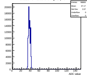
Pedestals mcm130-6610-refv4-g0-s0-p1 ch 4 test1
