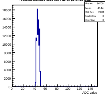
Pedestals mcm130-6610-refv4-g0-s0-p1 ch 20 test1
