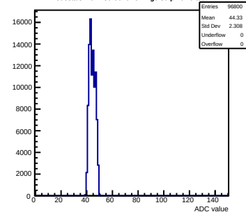
Pedestals mcm130-6610-refv4-g0-s0-p1 ch 0 test1
