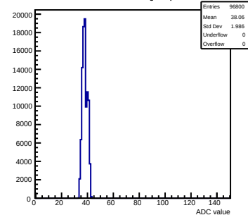
Pedestals mcm130-6610-refv4-g0-s0-p1 ch 12 test1
