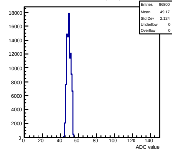
Pedestals mcm130-6610-refv4-g0-s0-p1 ch 8 test1
