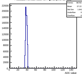
Pedestals mcm130-6610-refv4-g0-s0-p1 ch 30 test1
