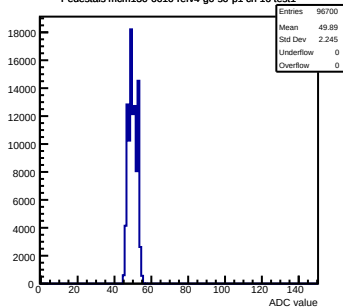
Pedestals mcm130-6610-refv4-g0-s0-p1 ch 16 test1
