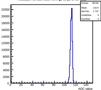
Pedestals mcm130-6610-rlv6-g0-s0-p1 ch 19 test1
