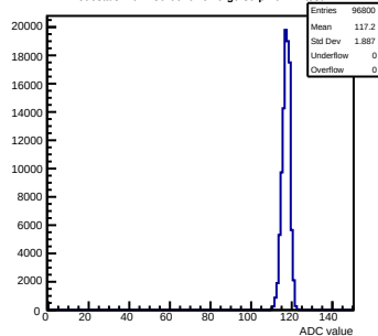
Pedestals mcm130-6610-rfv6-g0-s0-p1 ch 71 test1
