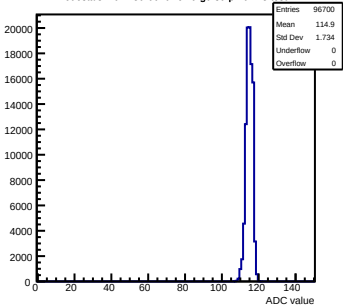
Pedestals mcm130-6610-rlv6-g0-s0-p1 ch 23 test1
