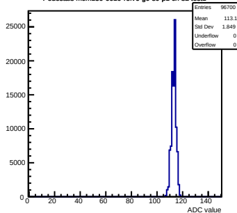
Pedestals mcm130-6610-rlv6-g0-s0-p1 ch 82 test1
