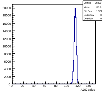
Pedestals mcm130-6610-rtv6-g0-s0-p1 ch 11 test1
