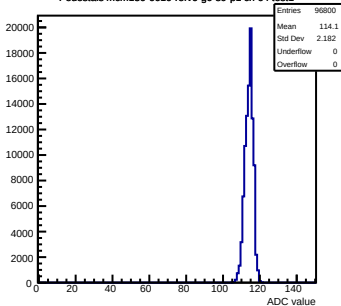
Pedestals mcm130-6610-rfv6-g0-s0-p1 ch 64 test1
