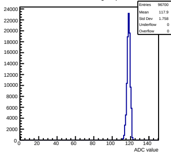
Pedestals mcm130-6610-rlv6-g0-s0-p1 ch 92 test1
