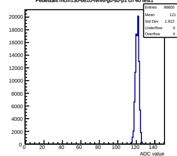
Pedestals mcm130-6610-rlv6-g0-s0-p1 ch 40 test1
