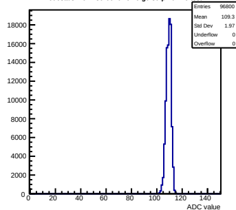
Pedestals mcm130-6610-rfv6-g0-s0-p1 ch 70 test1
