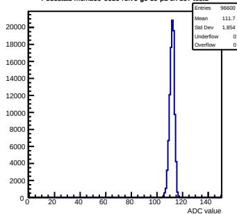
Pedestals mcm130-6610-rlv6-g0-s0-p1 ch 107 test1
