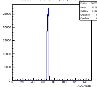
Pedestals mcm131-8416-refv2-g0-s0-p1 ch 91 test1
