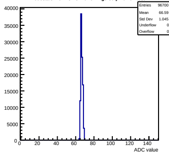
Pedestals mcm131-8416-refv2-g0-s0-p1 ch 94 test1
