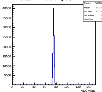
Pedestals mcm131-8416-refv2-g0-s0-p1 ch 86 test1
