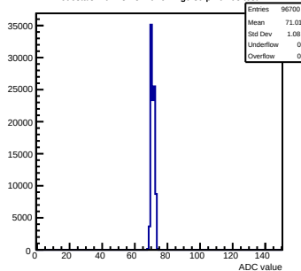
Pedestals mcm131-8416-refv2-g0-s0-p1 ch 93 test1
