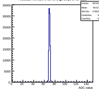
Pedestals mcm131-8416-refv2-g0-s0-p1 ch 89 test1
