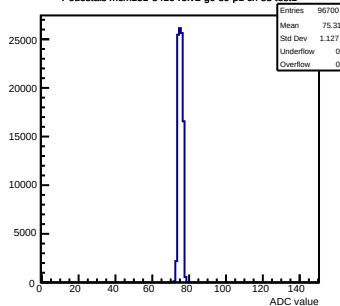
Pedestals mcm131-8416-refv2-g0-s0-p1 ch 85 test1
