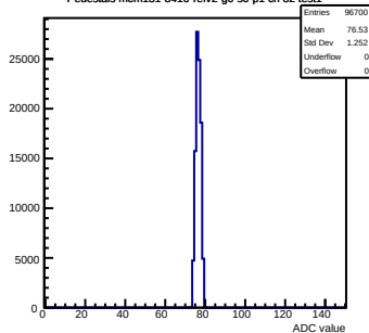
Pedestals mcm131-8416-refv2-g0-s0-p1 ch 82 test1
