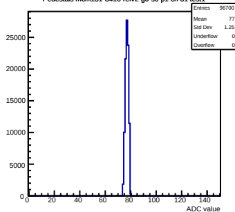
Pedestals mcm131-8416-refv2-g0-s0-p1 ch 81 test1
