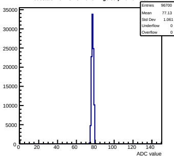
Pedestals mcm131-8416-refv2-g0-s0-p1 ch 92 test1
