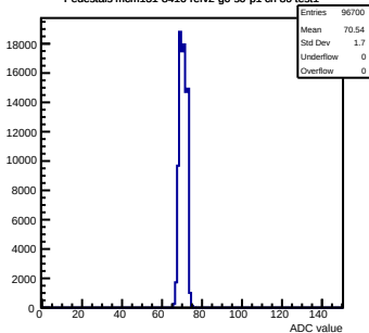
Pedestals mcm131-8416-refv2-g0-s0-p1 ch 80 test1
