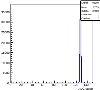
Pedestals mcm132-8015-refV0-g0-s0-p1 ch 15 test1
