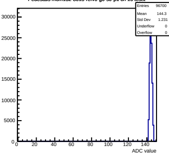
Pedestals mcm132-8015-relv0-g0-s0-p1 ch 16 test1
