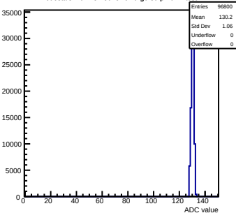
Pedestals mcm132-8015-refV0-g0-s0-p1 ch 4 test1
