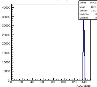
Pedestals mcm132-8015-rev0-g0-s0-p1 ch 95 test1
