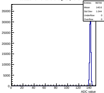
Pedestals mcm132-8015-rev0-g0-s0-p1 ch 84 test1
