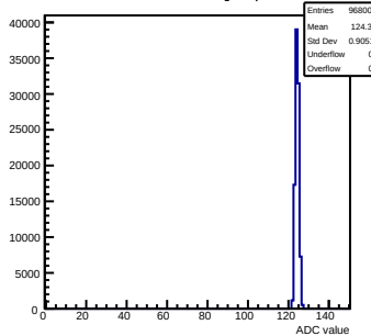
Pedestals mcm132-8015-refv0-g0-s0-p1 ch 78 test1
